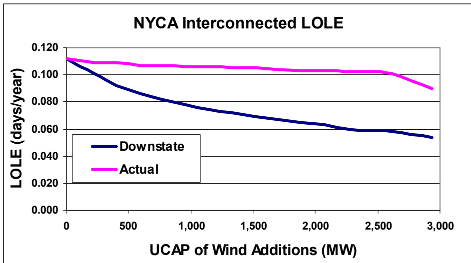
Figure 5.3 NYCA Interconnected LOLE vs. UCAP of Wind Additions
