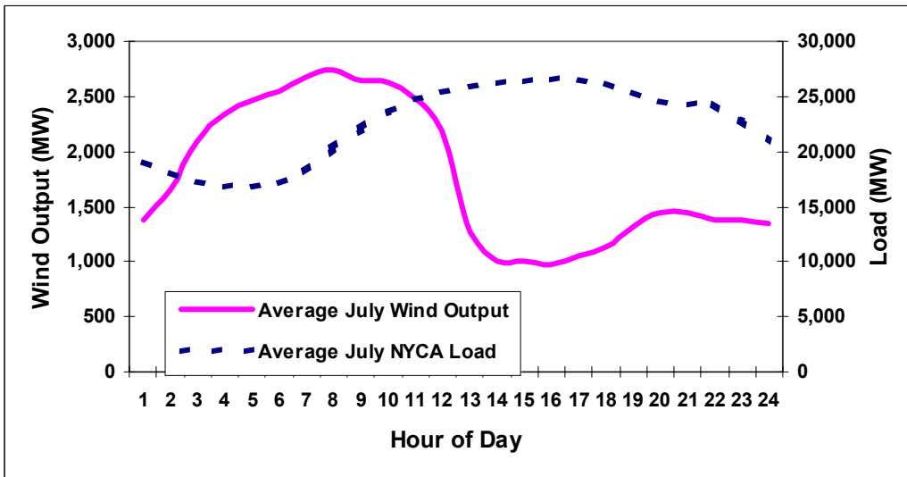
Figure 5.17 Average hourly output for all 101 wind sites and NYCA average load for July
