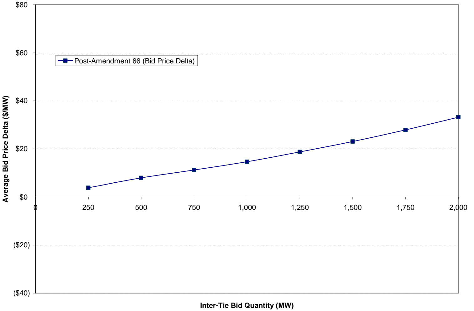
Figure 10. Average Bid Price Deltas for Incremental Energy (September 2006)
