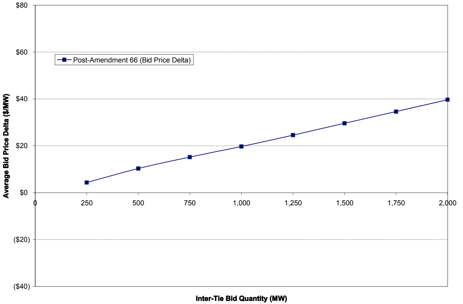
Figure 10. Average Bid Price Deltas for Incremental Energy (January 2007)
