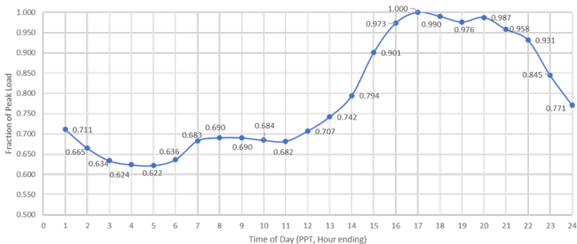
Figure 3.5-80 Goleta LCR Sub-area 2028 Peak Day Forecast Profiles
