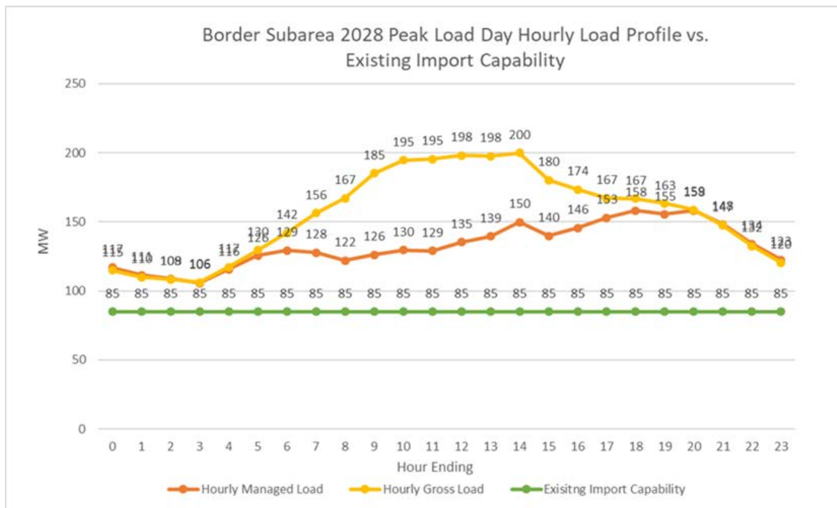
Figure 3.5-99 Border LCR Sub-area 2028 Peak Day Forecast Profiles
