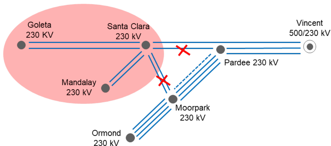
Figure 3.5-81 Santa Clara LCR Sub-area
