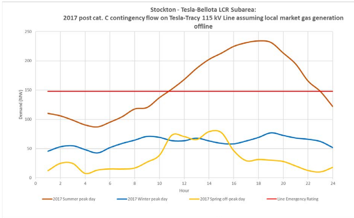
Figure 3.5-27 Tesla-Bellota LCR Sub-area 2017 Limiting Post Contingency Peak Day Profiles
