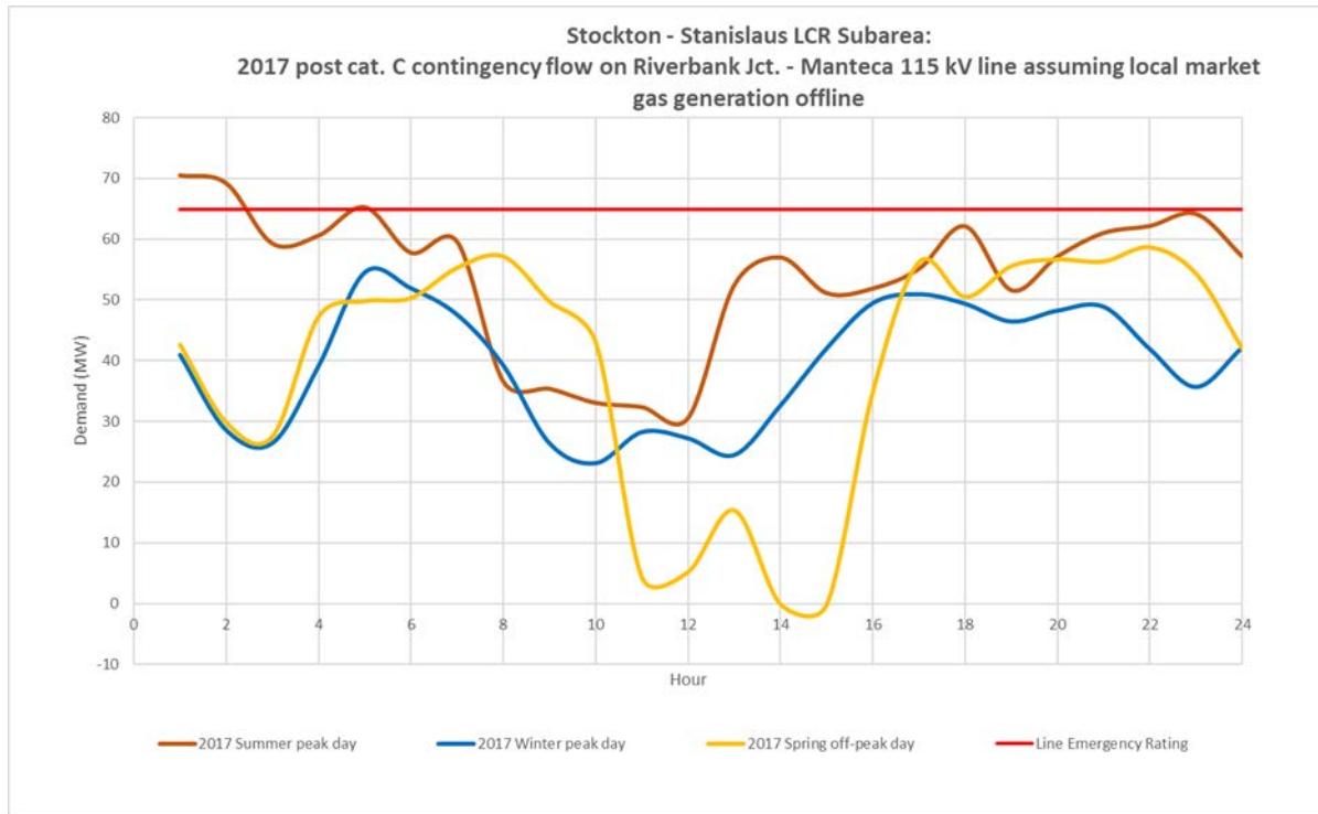
Figure 3.5-24 Stanislaus LCR Sub-area 2017 Limiting Post Contingency Peak Day Profiles
