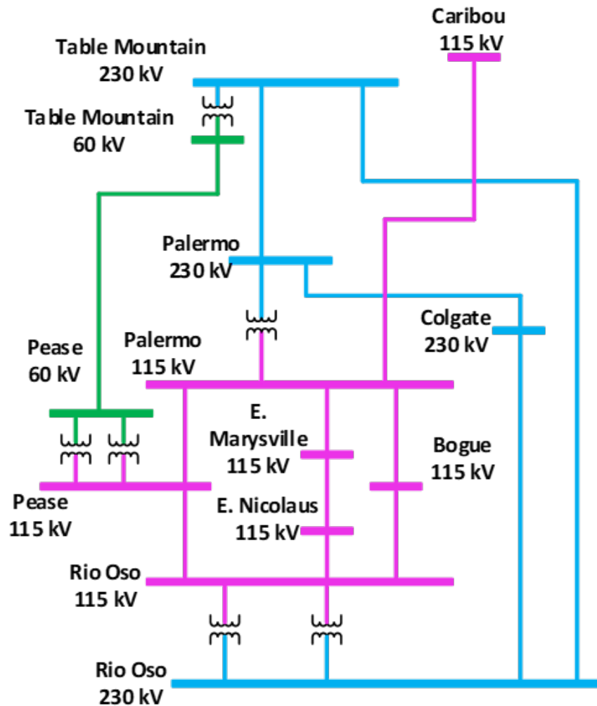
Figure 3.5-17 Table Mountain LCR Sub-area
