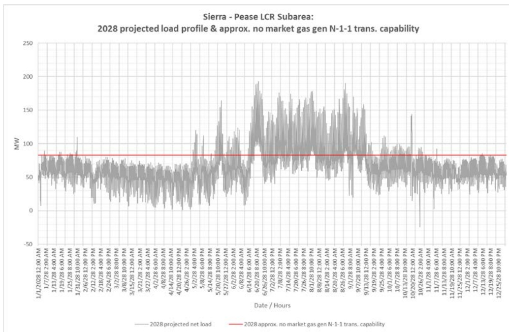
Figure 3.5-13 Pease LCR Sub-area 2028 Forecast Hourly Profiles
