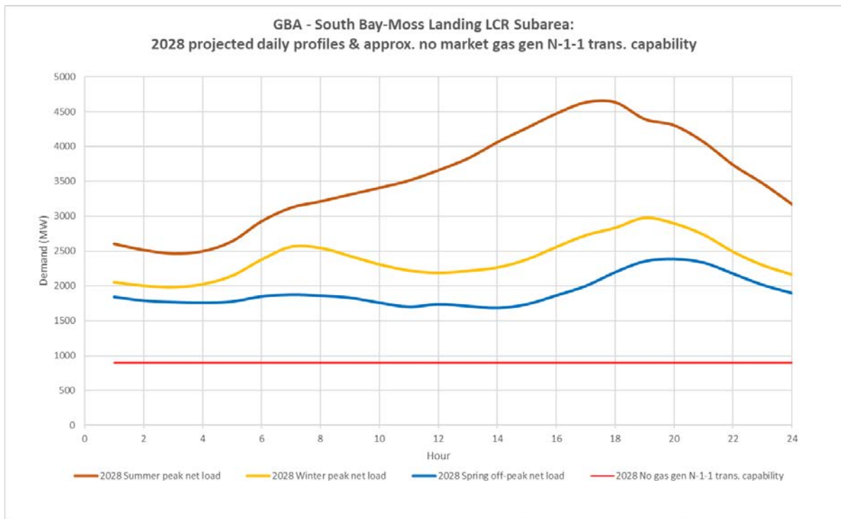
Figure 3.5-35 South Bay-Moss Landing LCR Sub-area 2028 Peak Day Forecast Profiles
