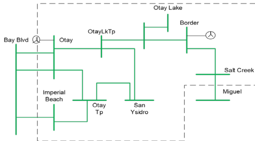
Figure 3.5-98 Border LCR Sub-area
