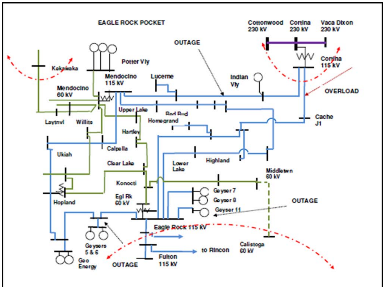
Figure 3.5-7 Eagle Roc LCR Sub-area
