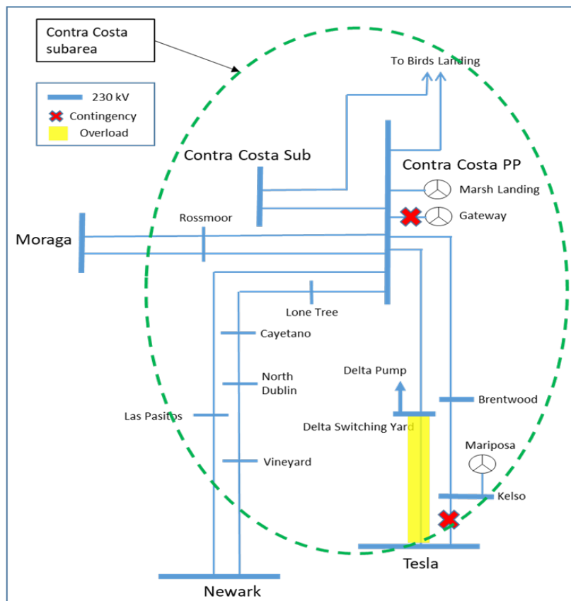
Figure 3.5-45 Contra Costa LCR Sub-area
