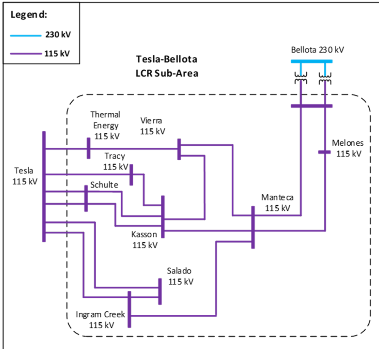
Figure 3.5-26 Tesla-Bellota LCR Sub-area
