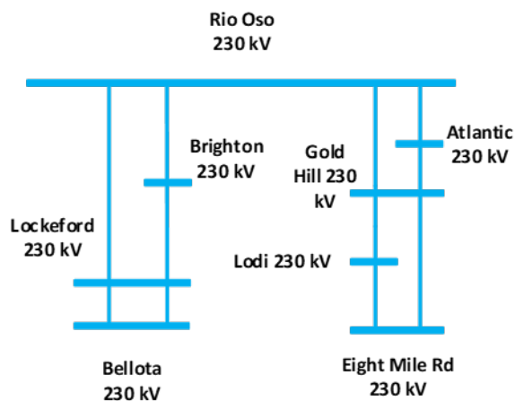
Figure 3.5-14 Pease LCR Sub-area
