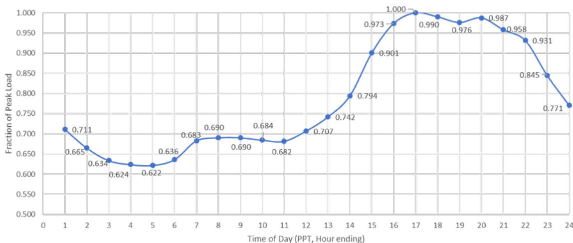
Figure 3.5-82 Santa Clara LCR Sub-area 2028 Peak Day Forecast Profiles
