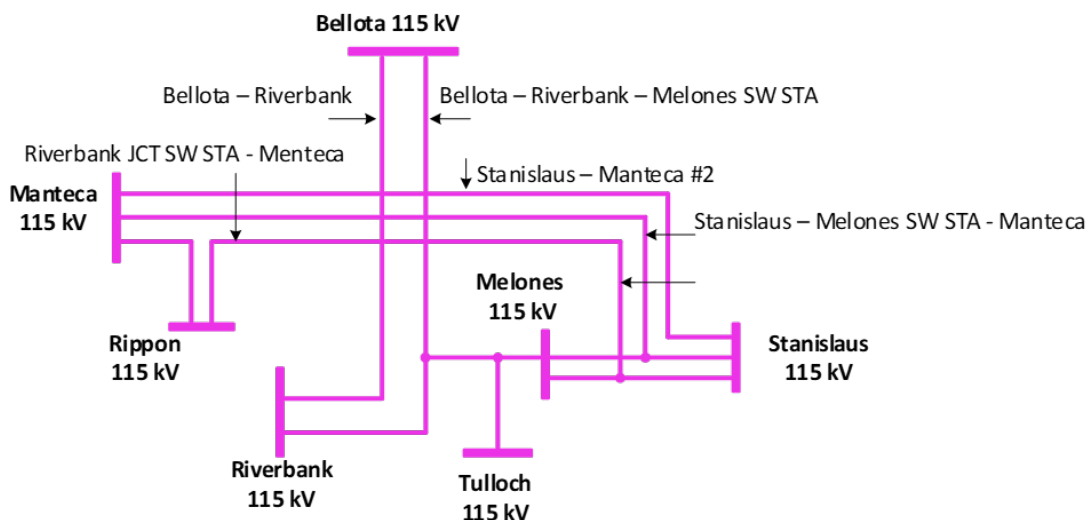
Figure 3.5-23 Stanislaus LCR Sub-area
