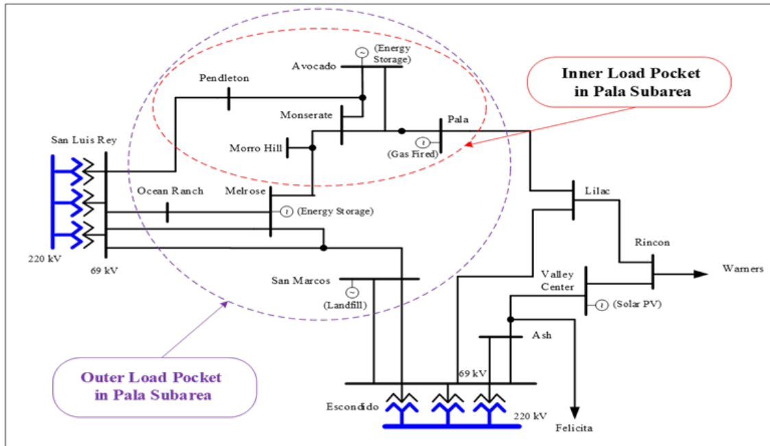
Figure 3.5-94 Pala Inner LCR Sub-area
