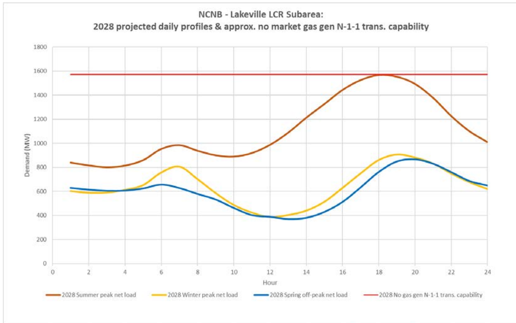
Figure 3.5-5 North Coast and North Bay 2028 Peak Day Forecast Profiles
