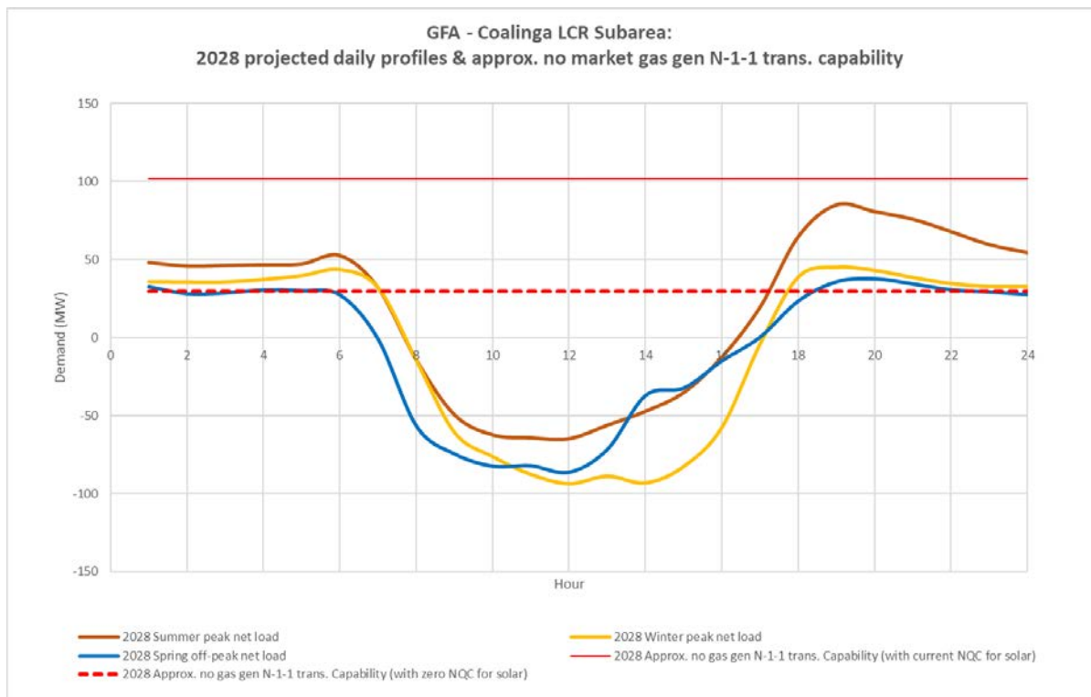
Figure 3.5-53 Coalinga LCR Sub-area 2028 Peak Day Forecast Profiles
