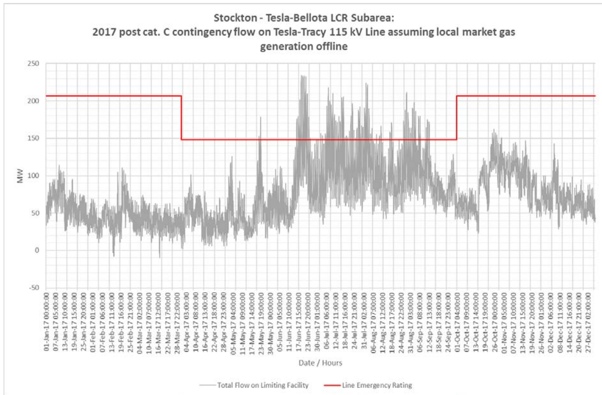
Figure 3.5-28 Tesla-Bellota LCR Sub-area 2017 Limiting Post Contingency Hourly Profiles
