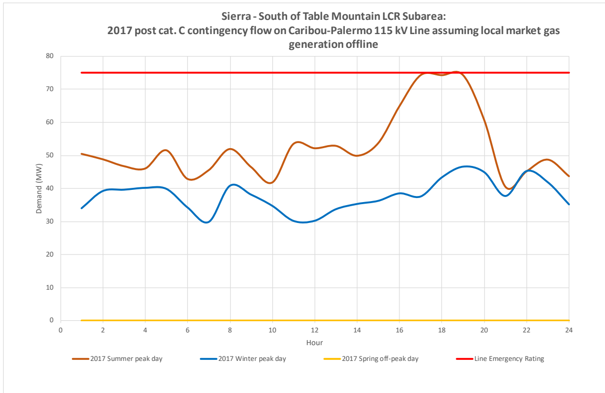
Figure 3.5-19 South of Table Mountain Sub-area 2017 Limiting Post Contingency Hourly Profiles
