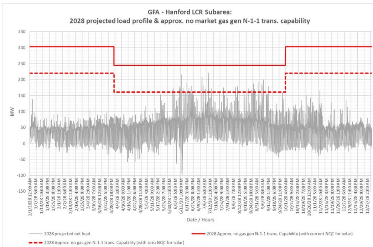
Figure 3.5-51 Hanford LCR Sub-area 2028 Forecast Hourly Profiles
