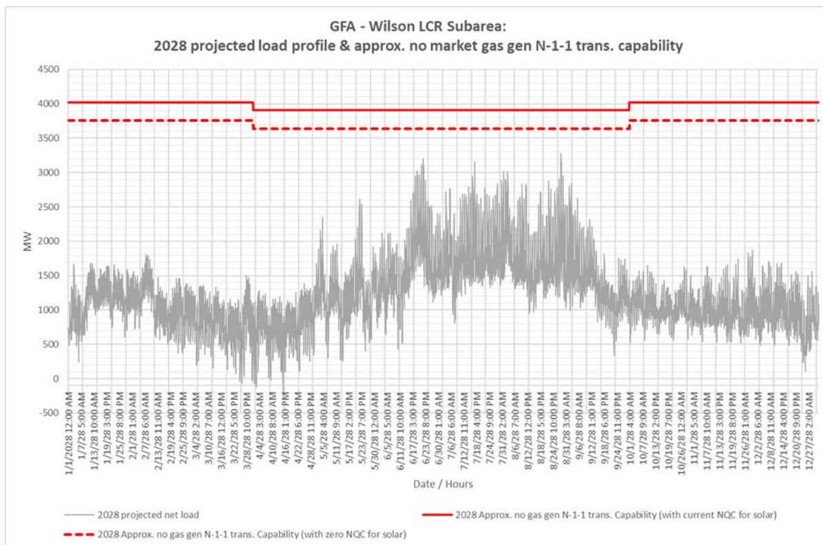
Figure 3.5-66 Wilson LCR Sub-area 2028 Forecast Hourly Profiles
