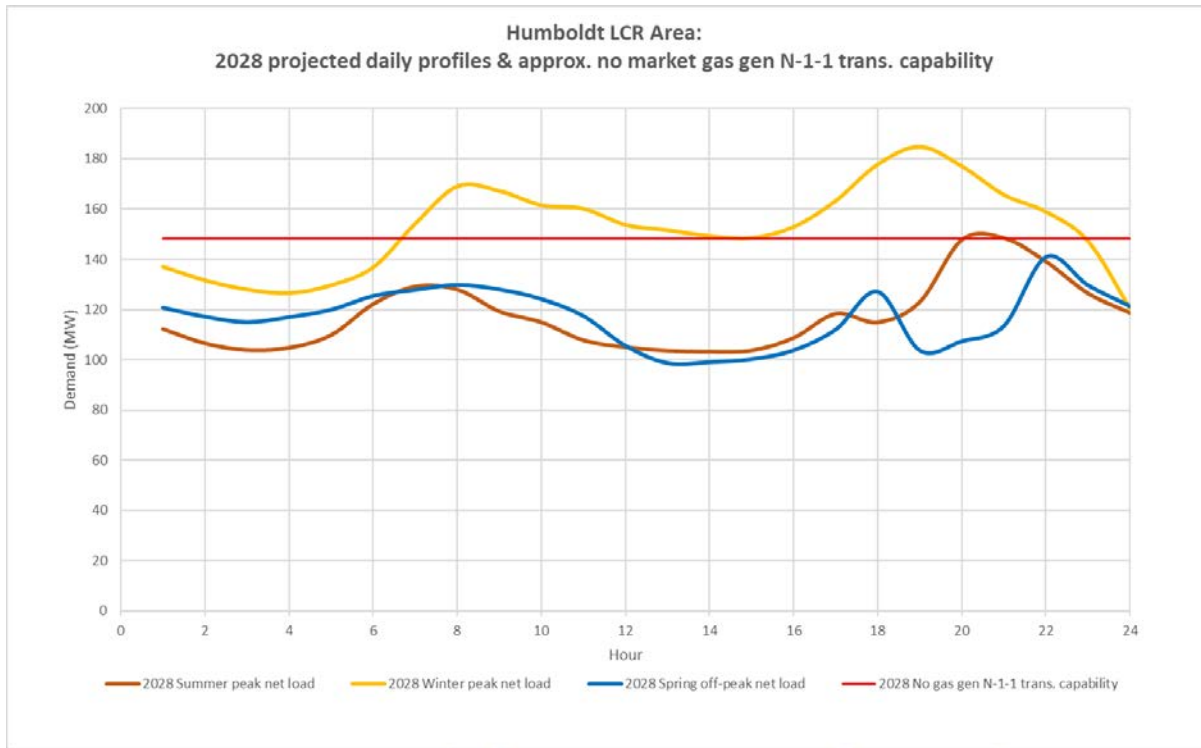
Figure 3.5-3 Humboldt 2028 Forecast Hourly Profile
