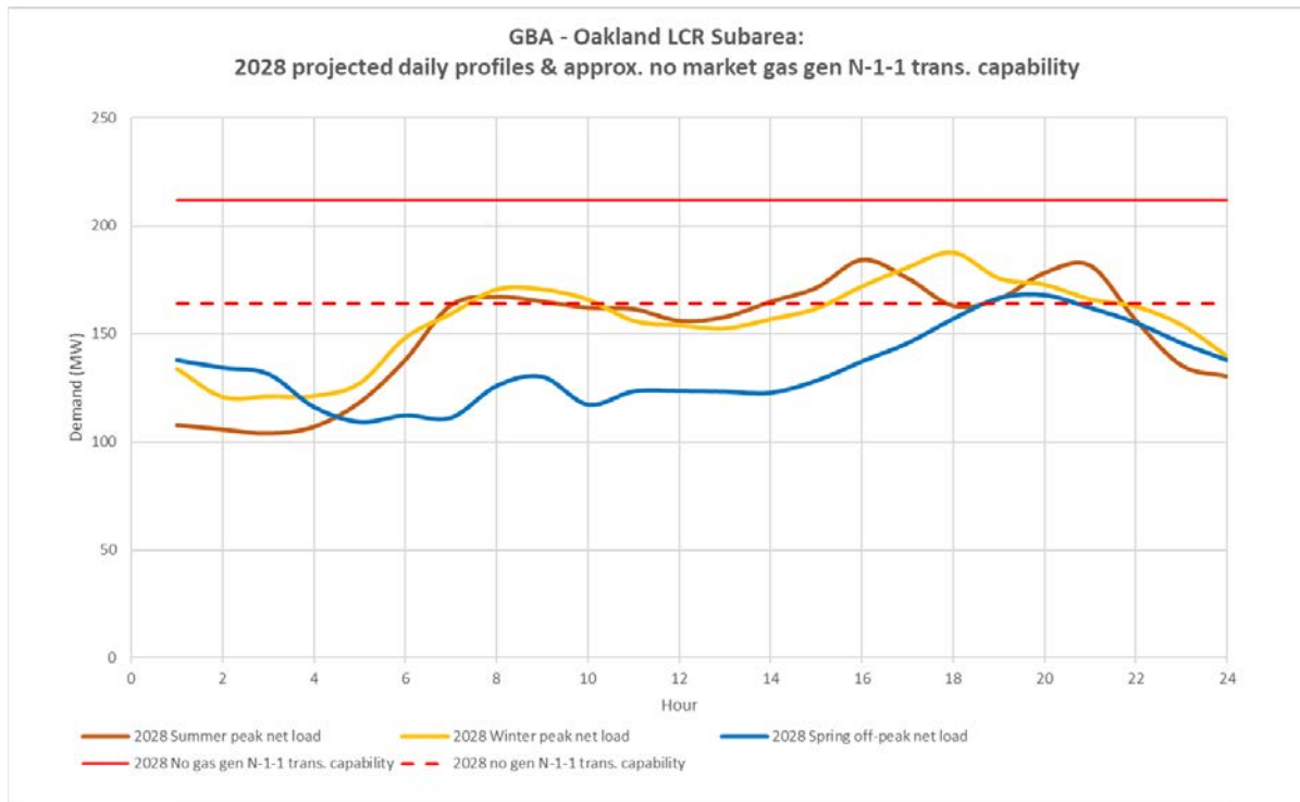
Figure 3.5-38 Oakland LCR Sub-area 2028 Peak Day Forecast Profiles
