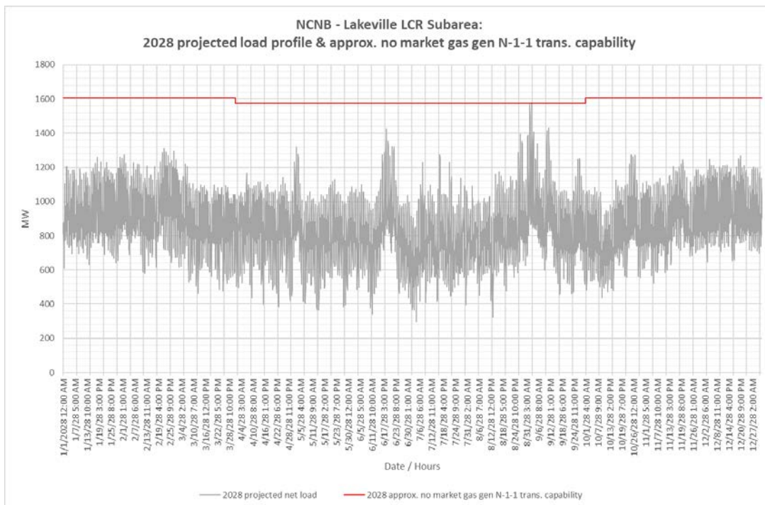
Figure 3.5-6 North Coast and North Bay 2028 Forecast Hourly Profile
