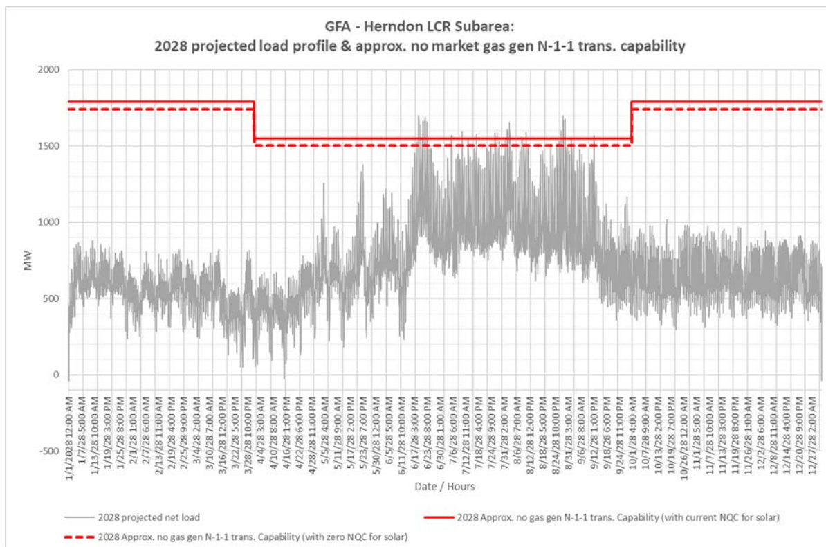
Figure 3.5-63 Herndon LCR Sub-area 2028 Forecast Hourly Profiles
