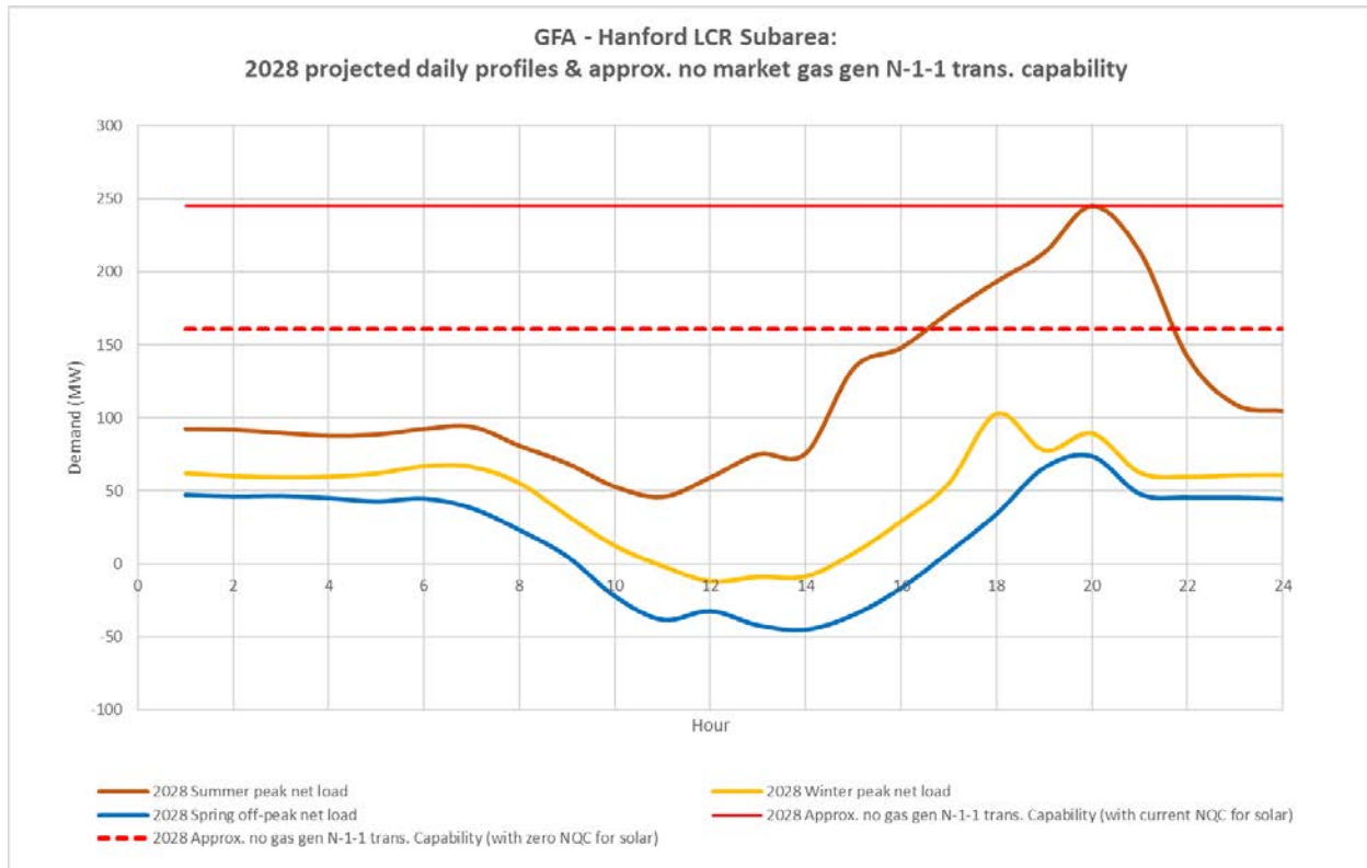
Figure 3.5-50 Hanford LCR Sub-area 2028 Peak Day Forecast Profiles
