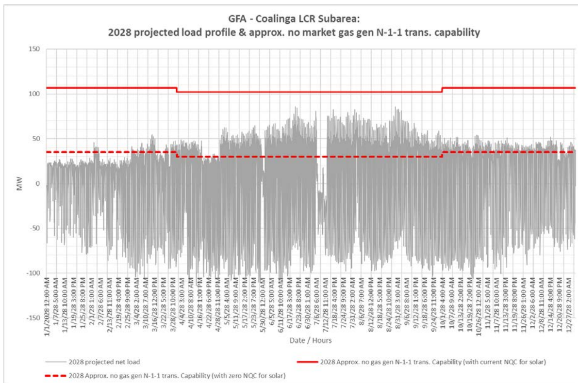
Figure 3.5-54 Coalinga LCR Sub-area 2028 Forecast Hourly Profiles
