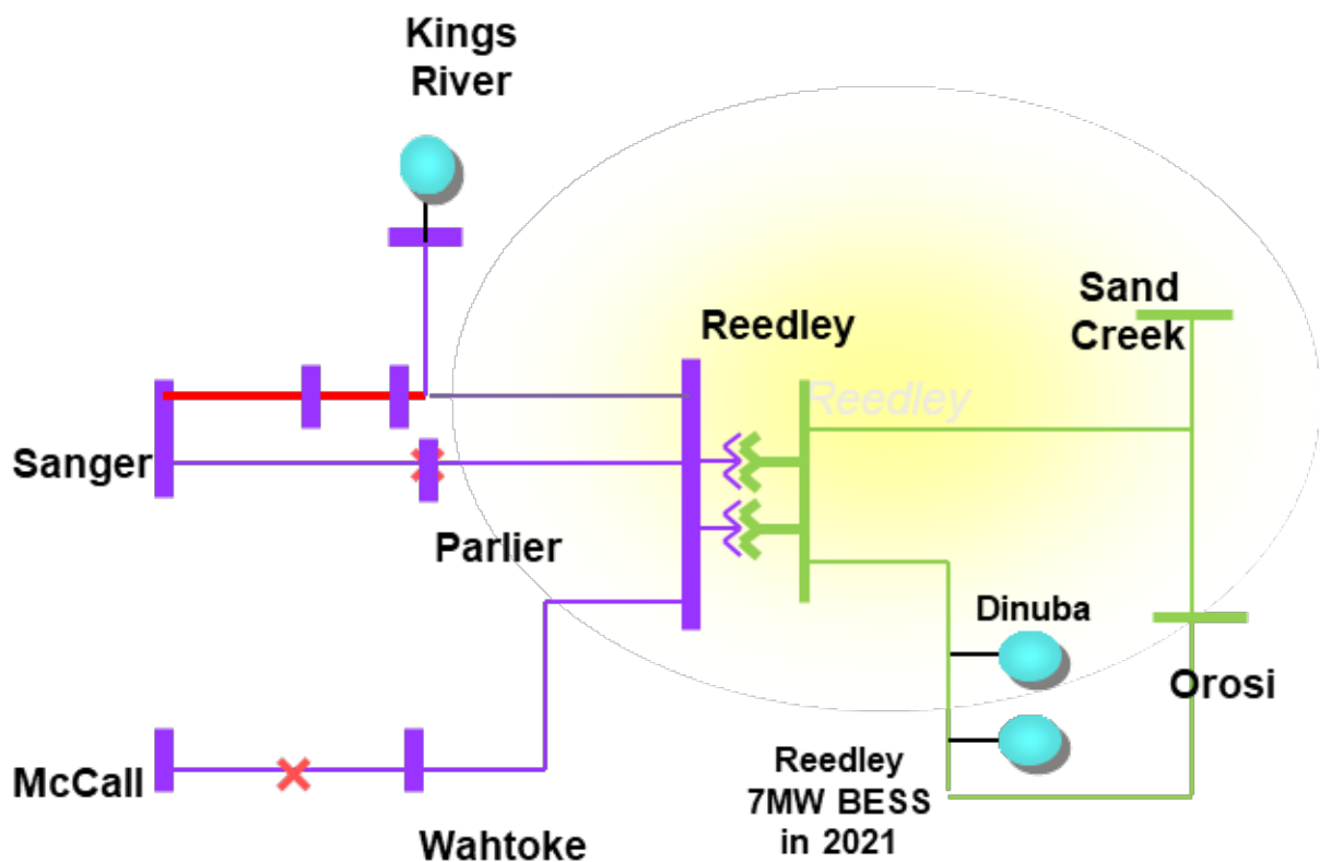
Figure 3.5-58 Reedley LCR Sub-area
