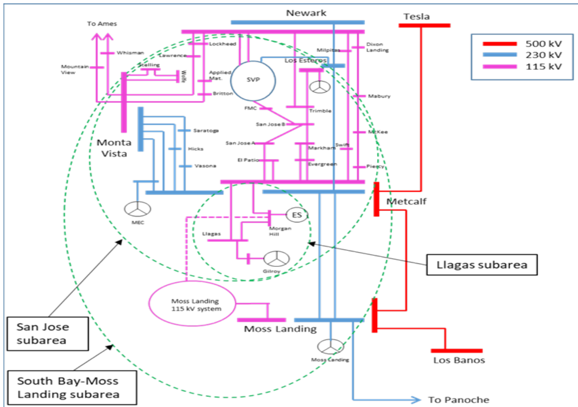
Figure 3.5-30 Llagas LCR Sub-area
