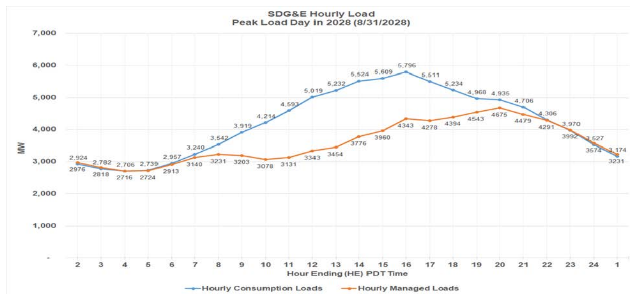
Figure 3.5-100 San Diego LCR Sub-area 2028 Peak Day Forecast Profiles
