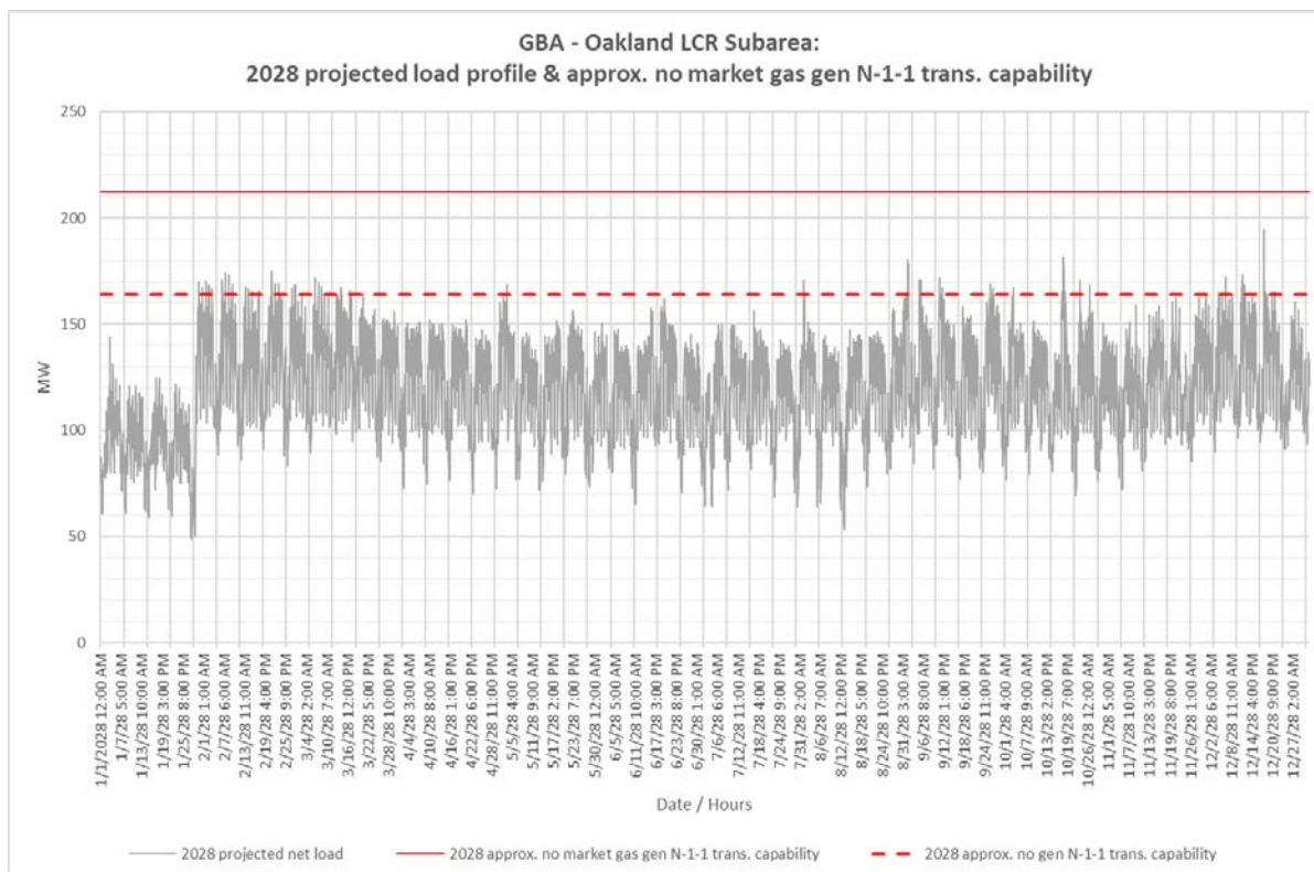
Figure 3.5-39 Oakland LCR Sub-area 2028 Forecast Hourly Profiles
