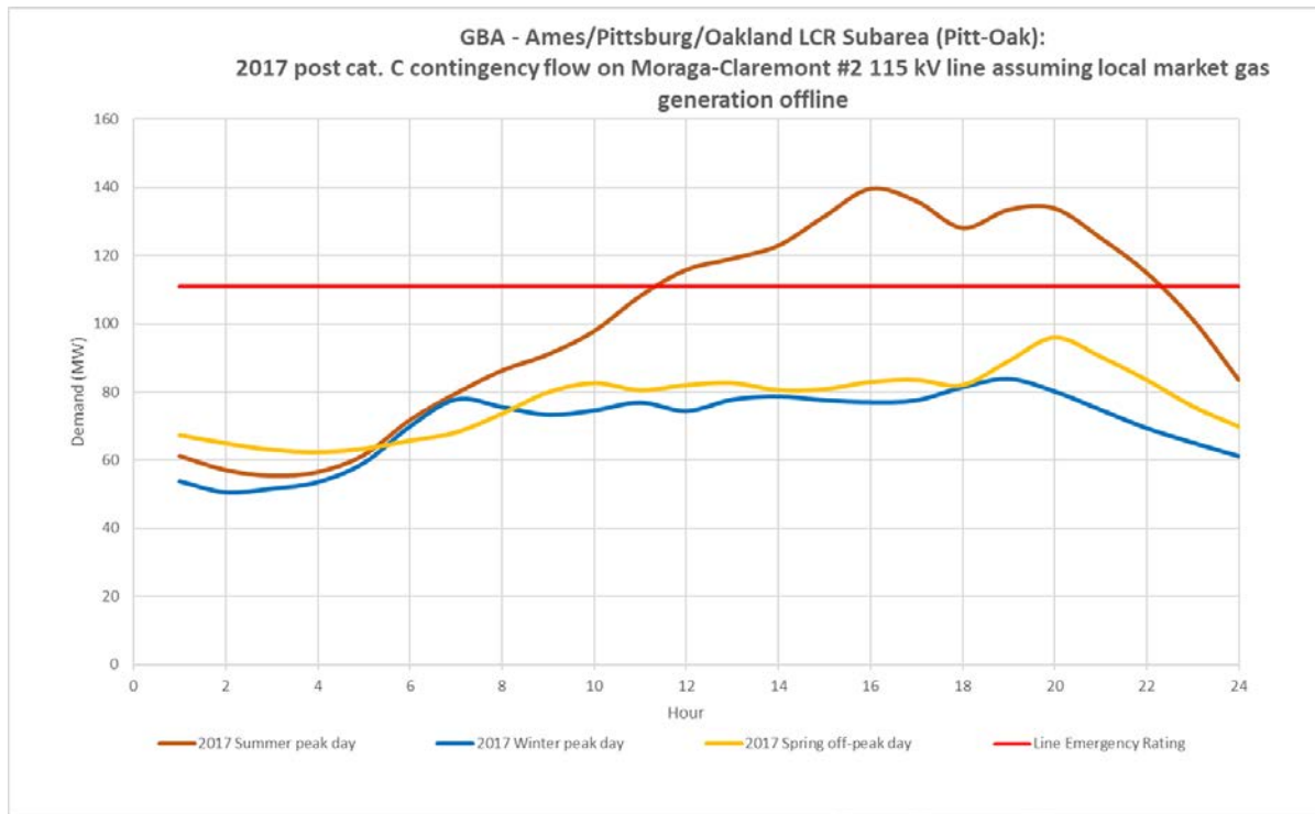
Figure 3.5-41 Ames-Pittsburg-Oakland LCR Sub-area 2017 Limiting Post Contingency Peak Day Profiles (Moraga-Claremont #2 115 kV line)
