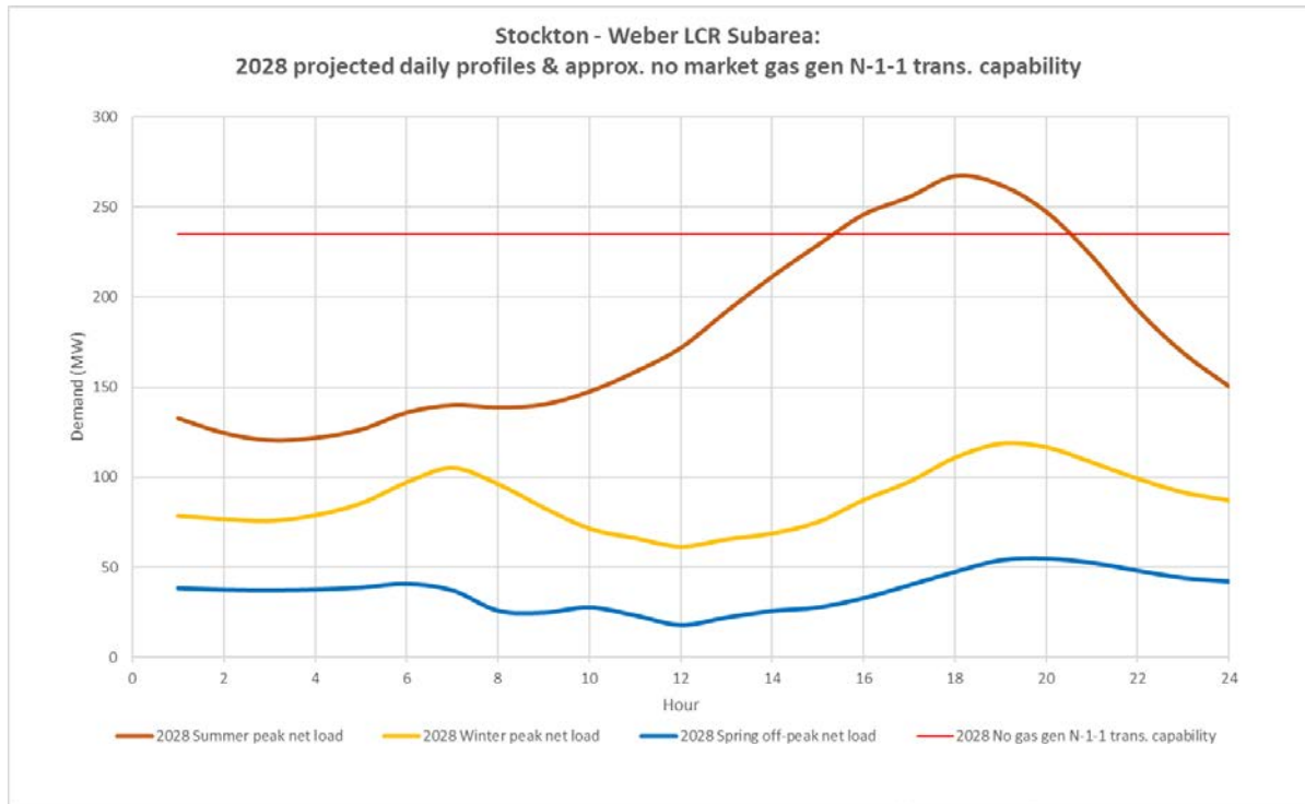
Figure 3.5-21 Weber LCR Sub-area 2028 Peak Day Forecast Profiles
