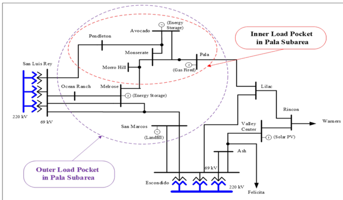
Figure 3.5-96 Pala Outer LCR Sub-area
