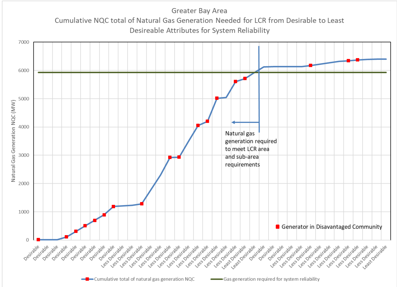
Figure C-1 Greater Bay Area Gas-Fired Flexible Attributes
