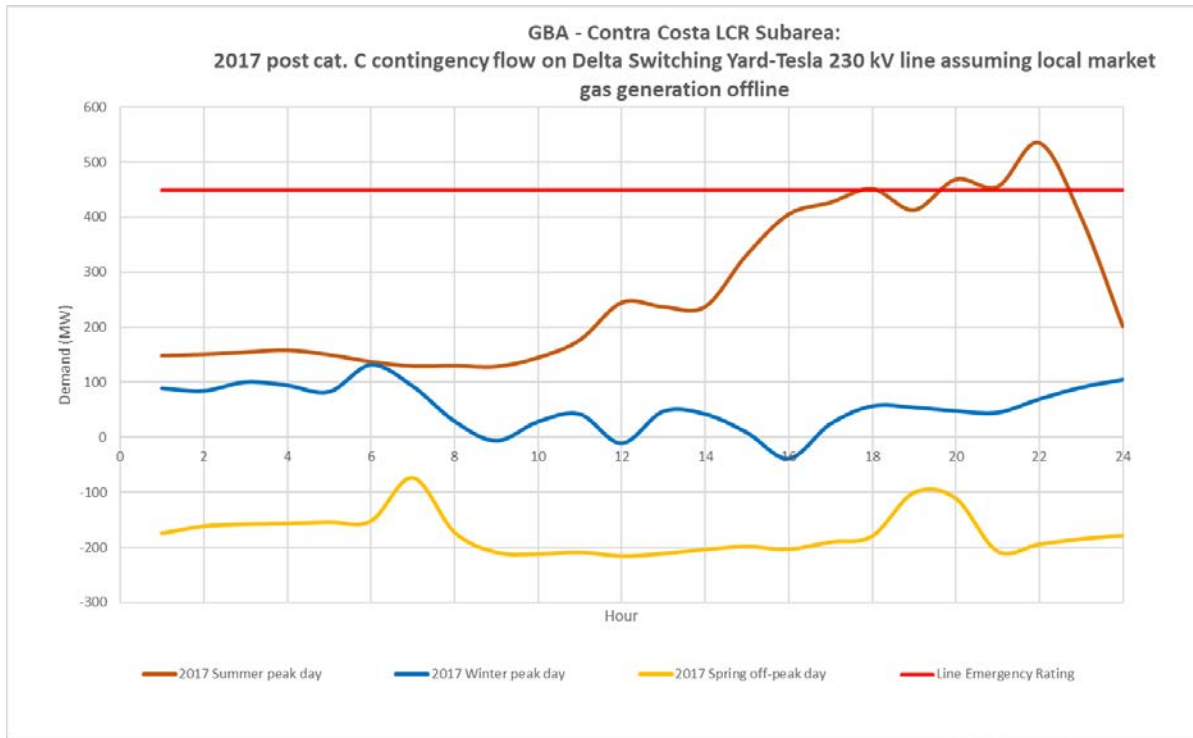
Figure 3.5-46 Contra Costa LCR Sub-area 2017 Limiting Post Contingency Peak Day Profiles
