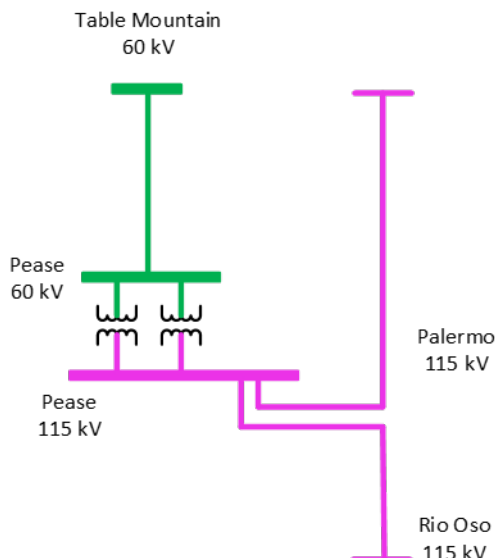
Figure 3.5-11 Pease LCR Sub-area
