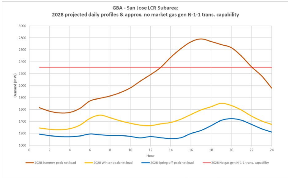
Figure 3.5-33 San Jose LCR Sub-area 2028 Peak Day Forecast Profiles
