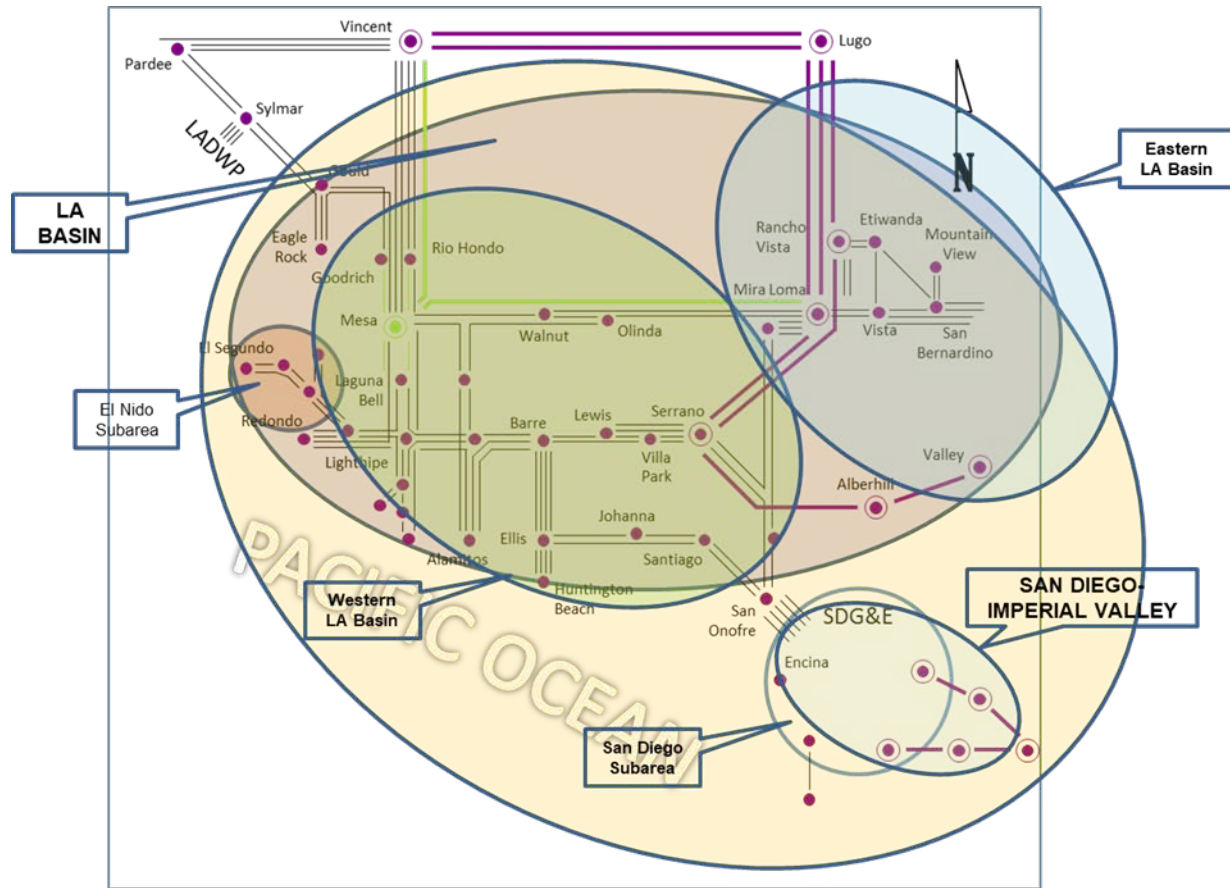
Figure 3.5-89 San Diego-Imperial Valley LCR Area
