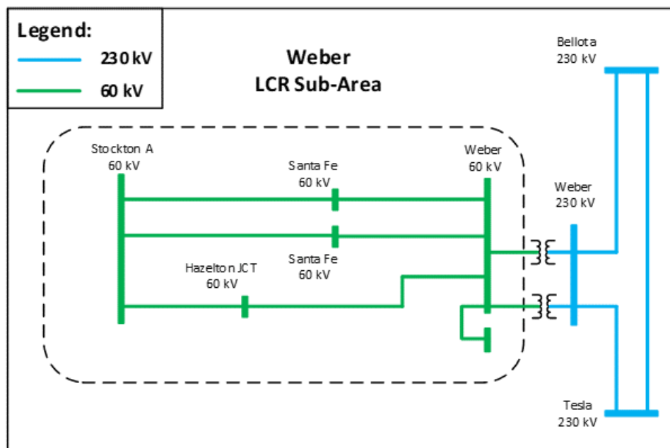
Figure 3.5-20 Weber LCR Sub-area
