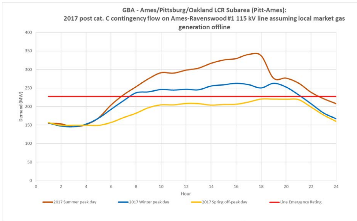
Figure 3.5-43 Ames-Pittsburg-Oakland LCR Sub-area 2017 Limiting Post Contingency Peak Day Profiles (Ames-Ravenswood #1 115 kV line)
