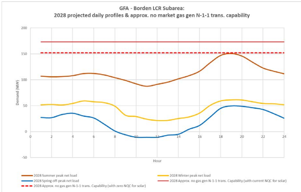
Figure 3.5-56 Borden LCR Sub-area 2028 Peak Day Forecast Profiles
