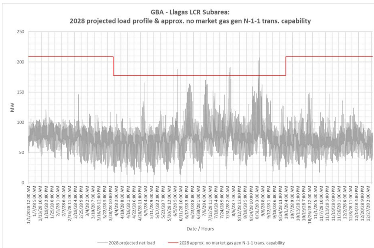
Figure 3.5-32 Llagas LCR Sub-area 2028 Forecast Hourly Profiles
