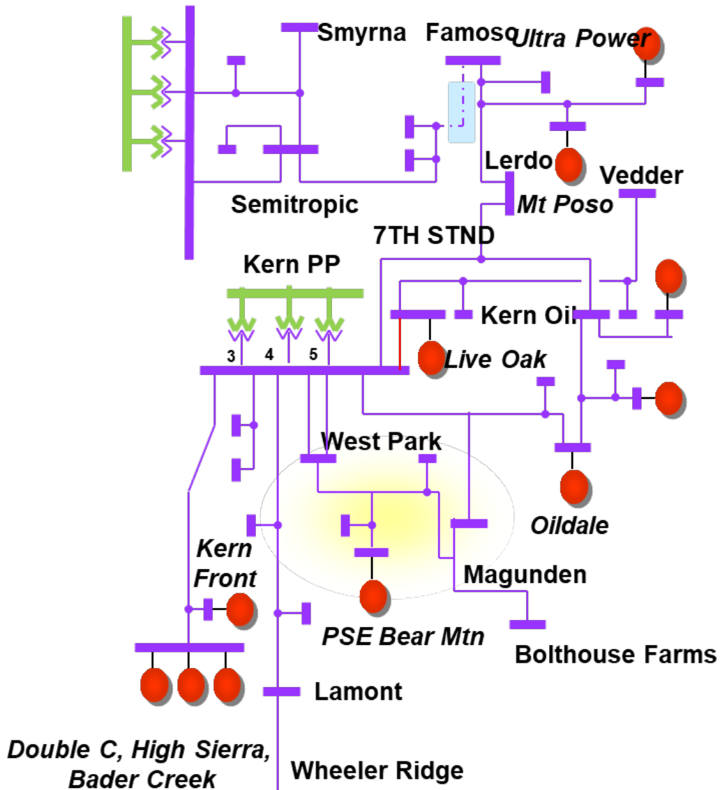
Figure 3.5-73 Kern Oil LCR Sub-area
