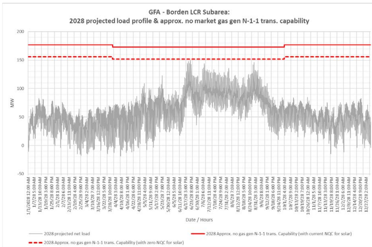
Figure 3.5-57 Borden LCR Sub-area 2028 Forecast Hourly Profiles
