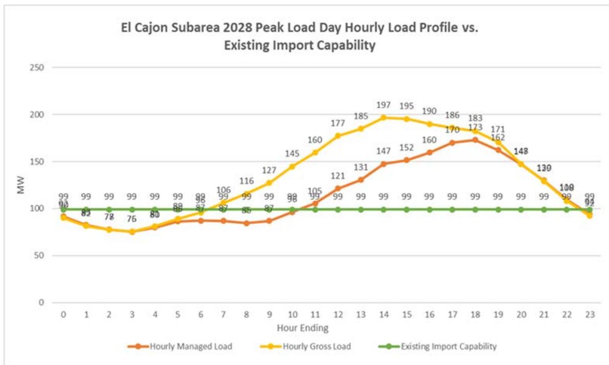
Figure 3.5-91 El Cajon LCR Sub-area 2028 Peak Day Forecast Profiles
