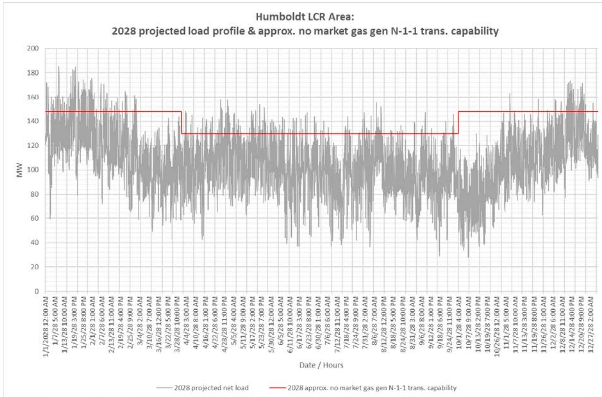
Figure 3.5-3 Humboldt 2028 Forecast Hourly Profile
