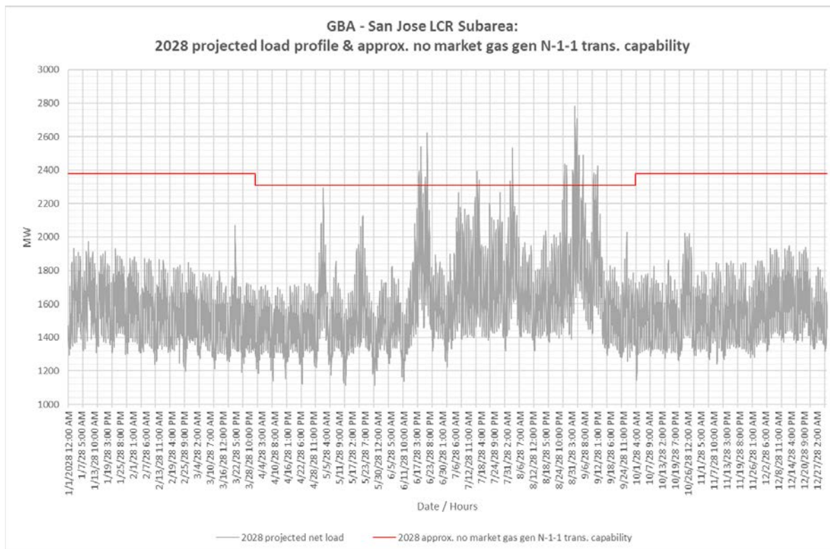
Figure 3.5-34 San Jose LCR Sub-area 2028 Forecast Hourly Profiles
