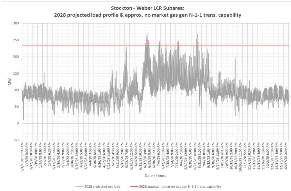
Figure 3.5-22 Weber LCR Sub-area 2028 Forecast Hourly Profiles
