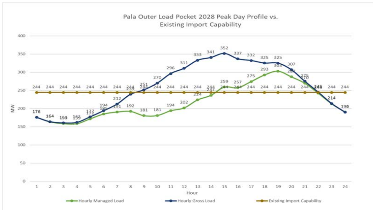
Figure 3.5-97 Pala Outer LCR Sub-area 2028 Peak Day Forecast Profiles
