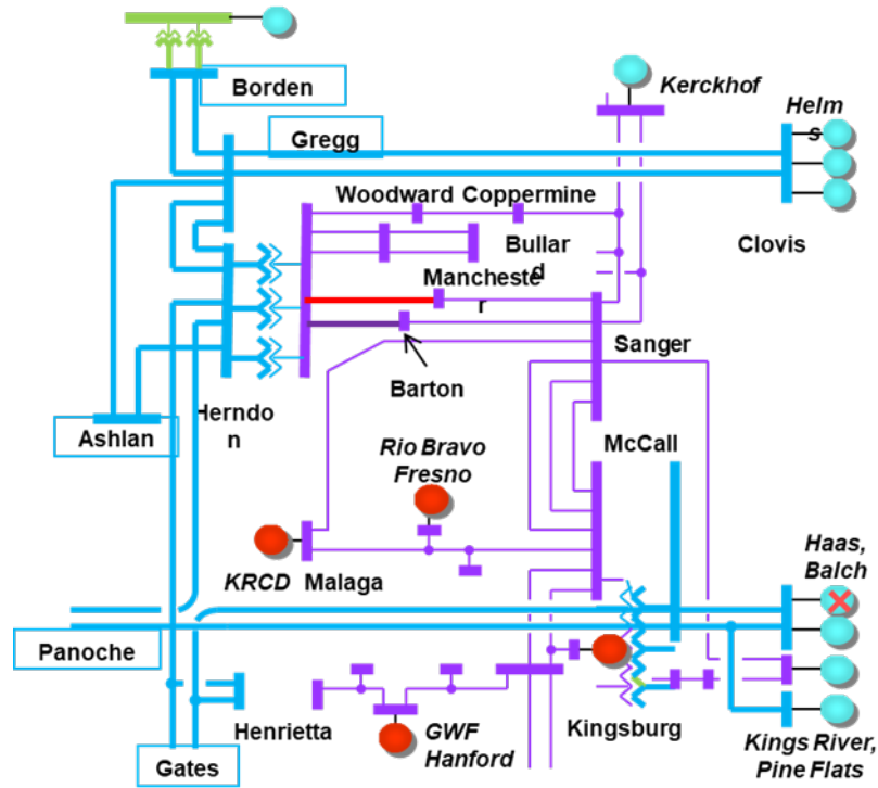
Figure 3.5-61 Herndon LCR Sub-area
