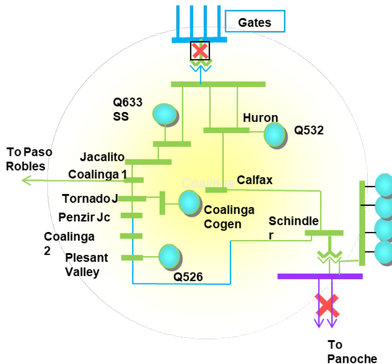
Figure 3.5-52 Coalinga LCR Sub-area
