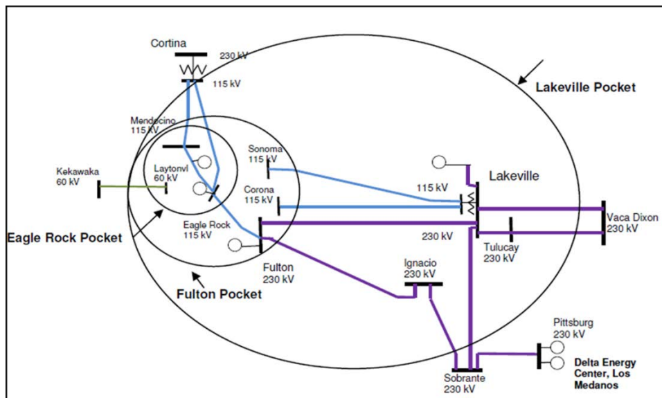
Figure 3.5-4 North Coast and North Bay LCR Area
