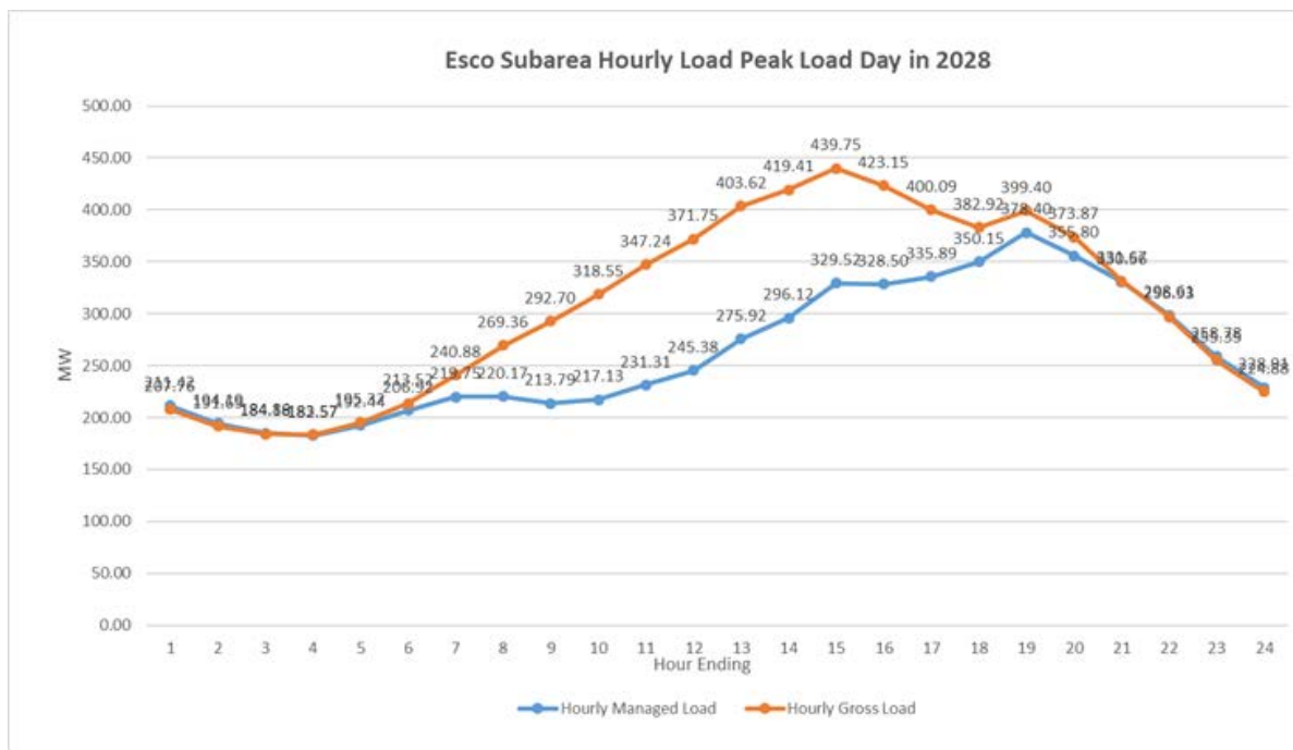
Figure 3.5-93 Esco LCR Sub-area 2028 Peak Day Forecast Profiles
