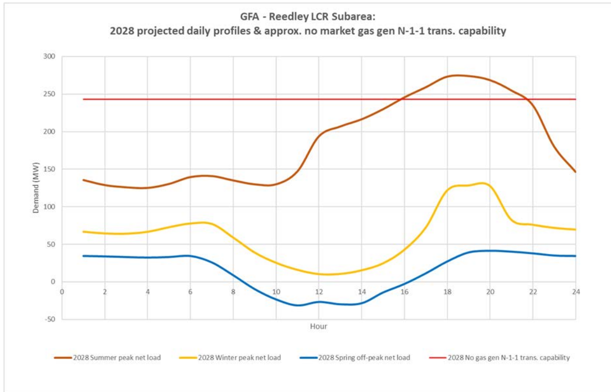
Figure 3.5-60 Reedley LCR Sub-area 2028 Forecast Hourly Profiles
