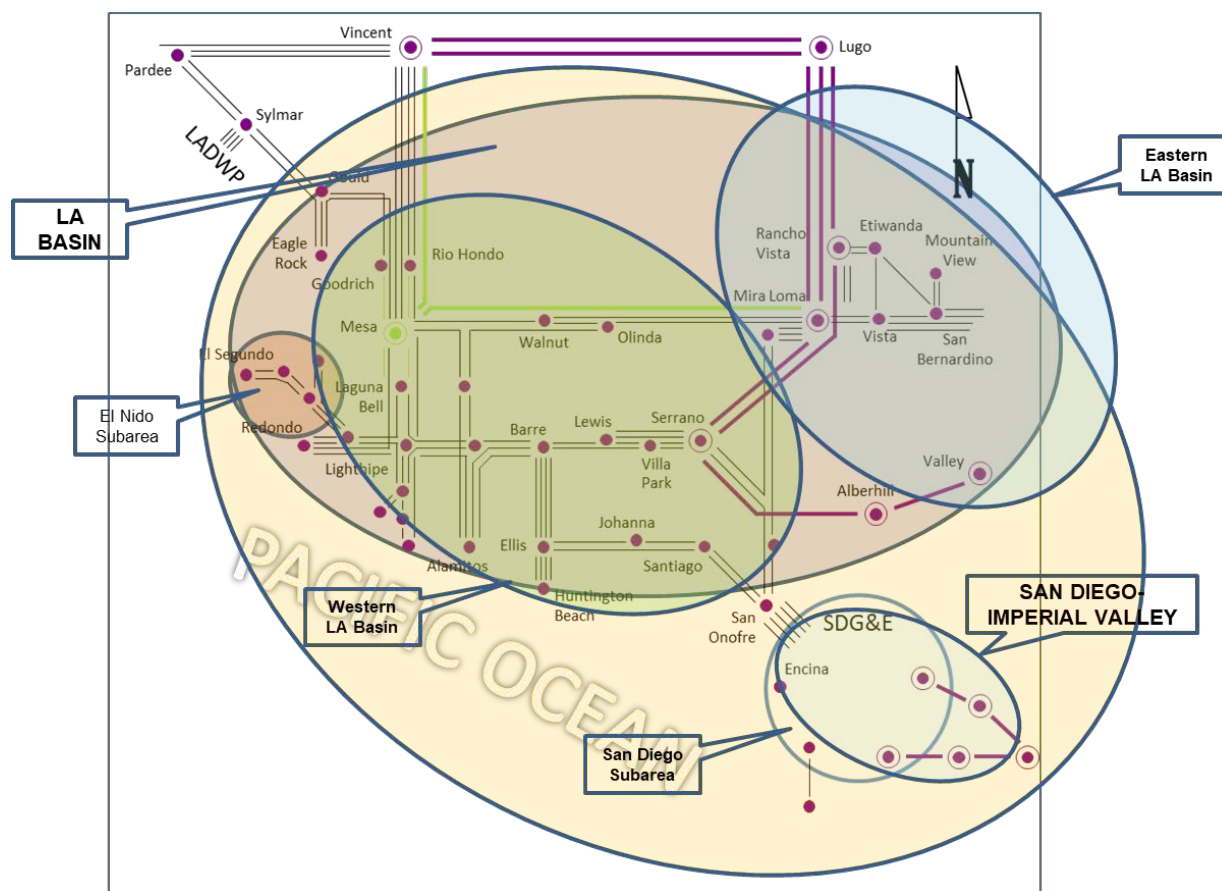
Figure 3.5-84 LA Basin LCR Area
