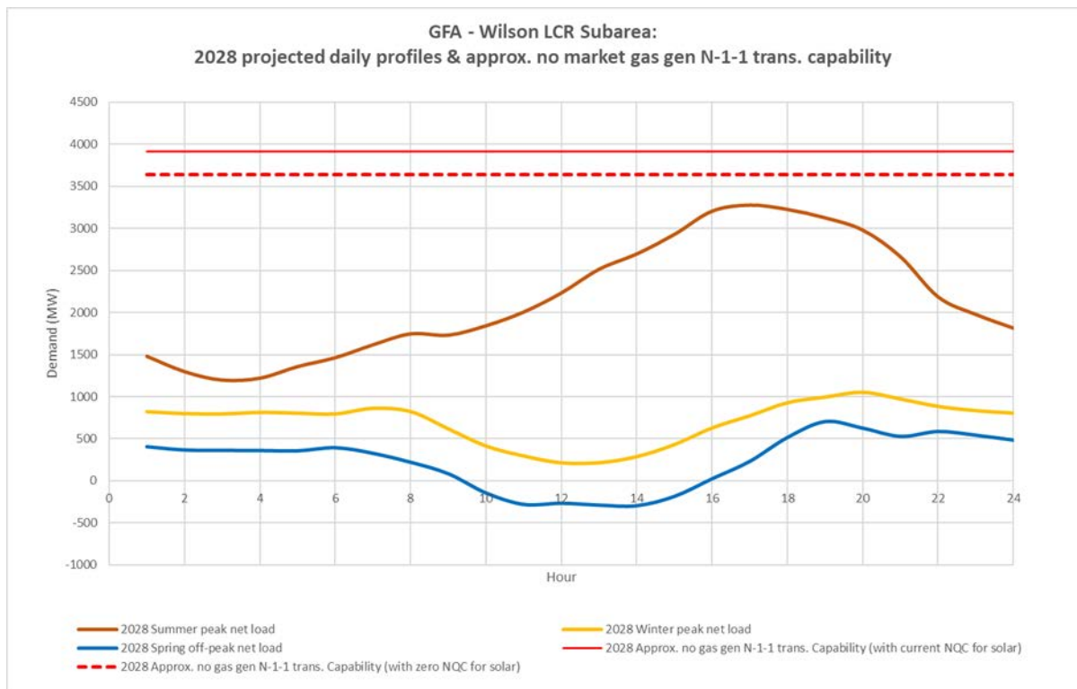
Figure 3.5-65 Wilson LCR Sub-area 2028 Peak Day Forecast Profiles
