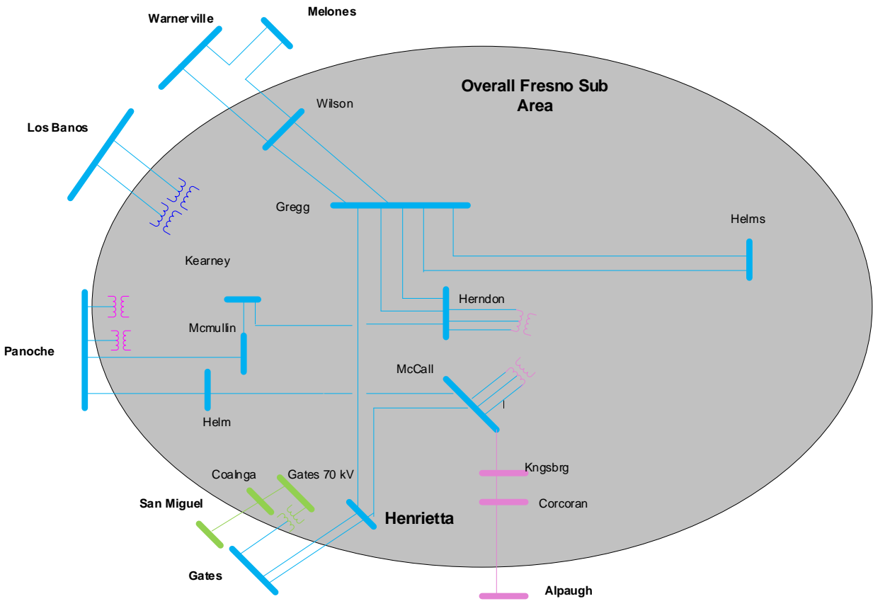
Figure 3.5-48 Fresno LCR Area
