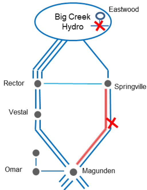
Figure 3.5-77 Vestal LCR Sub-area
