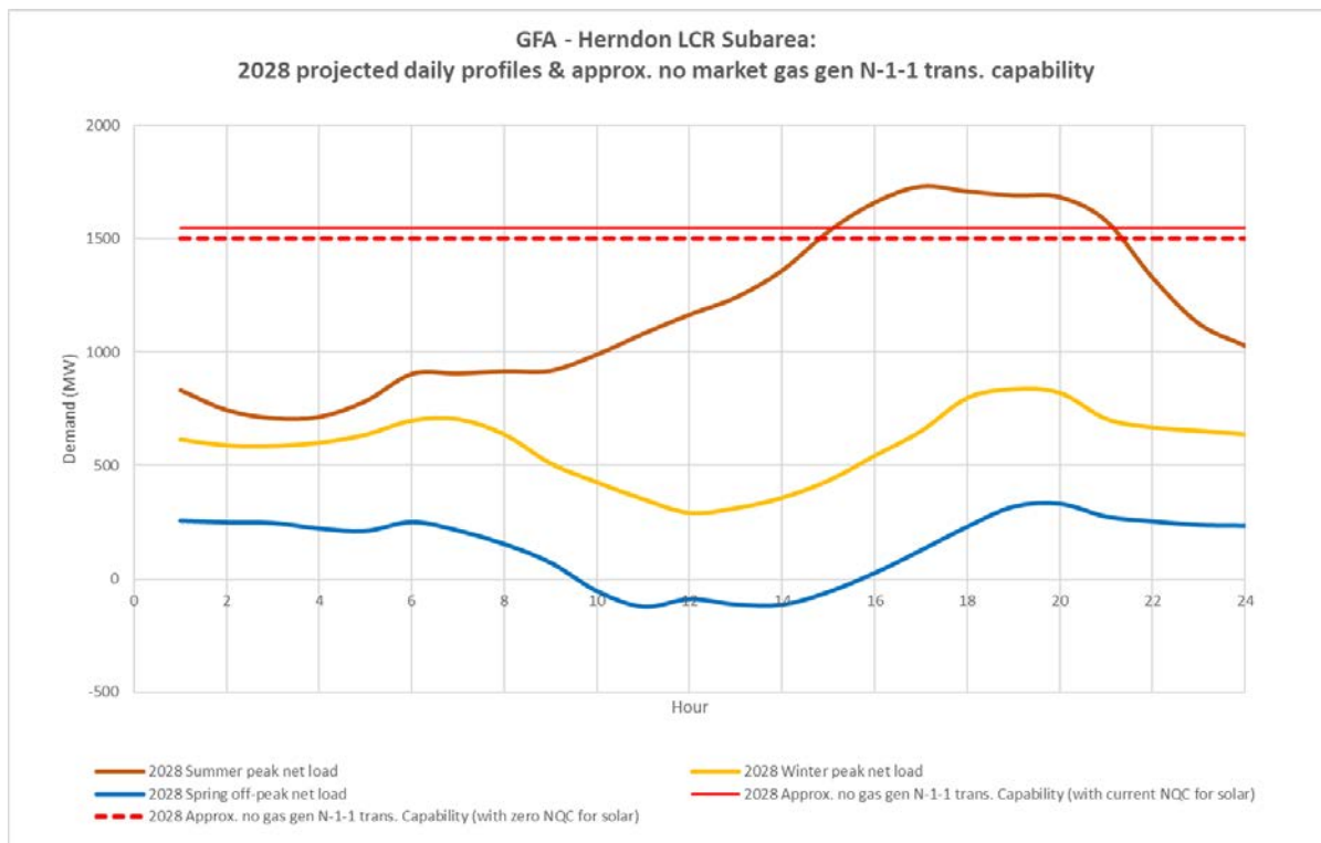
Figure 3.5-62 Herndon LCR Sub-area 2028 Peak Day Forecast Profiles
