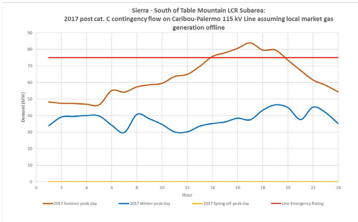
Figure 3.5-18 South of Table Mountain Sub-area 2017 Limiting Post Contingency Peak Day Profiles
