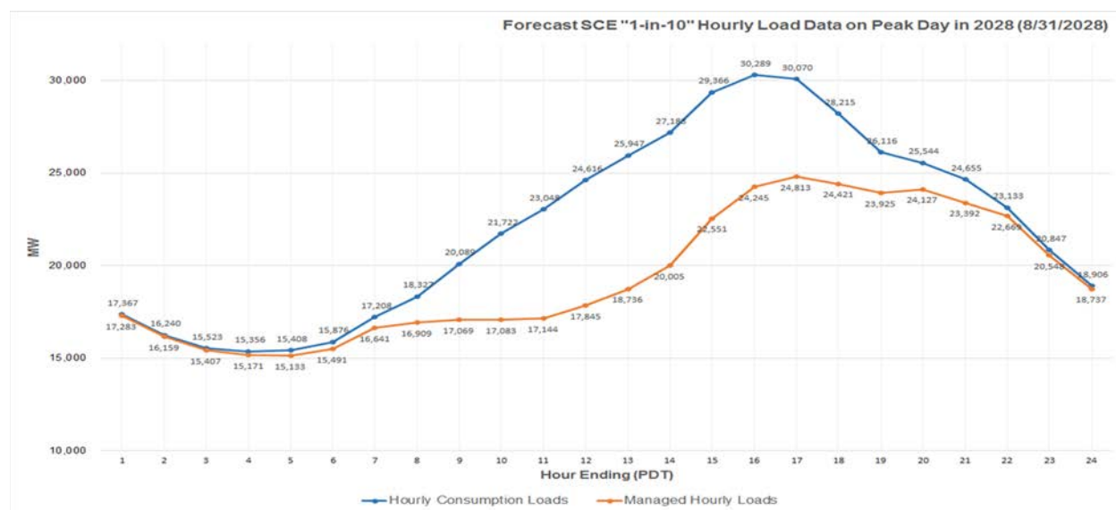
Figure 3.5-88 LA Basin LCR area 2028 Peak Day Forecast Profiles
