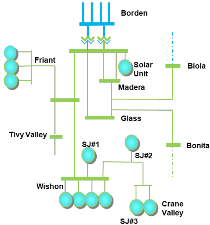
Figure 3.5-55 Borden LCR Sub-area
