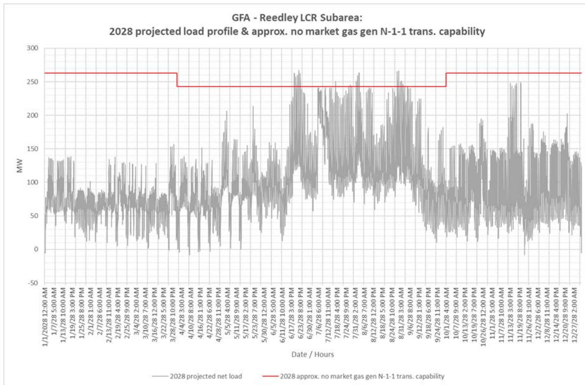
Figure 3.5-60 Reedley LCR Sub-area 2028 Forecast Hourly Profiles
