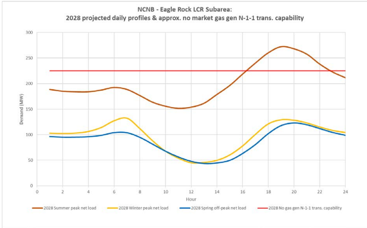
Figure 3.5-8 Eagle Rock LCR Sub-area 2028 Peak Day Forecast Profiles
