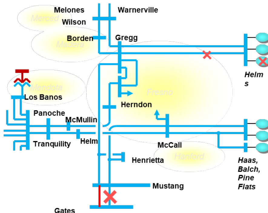
Figure 3.5-64 Wilson LCR Sub-area
