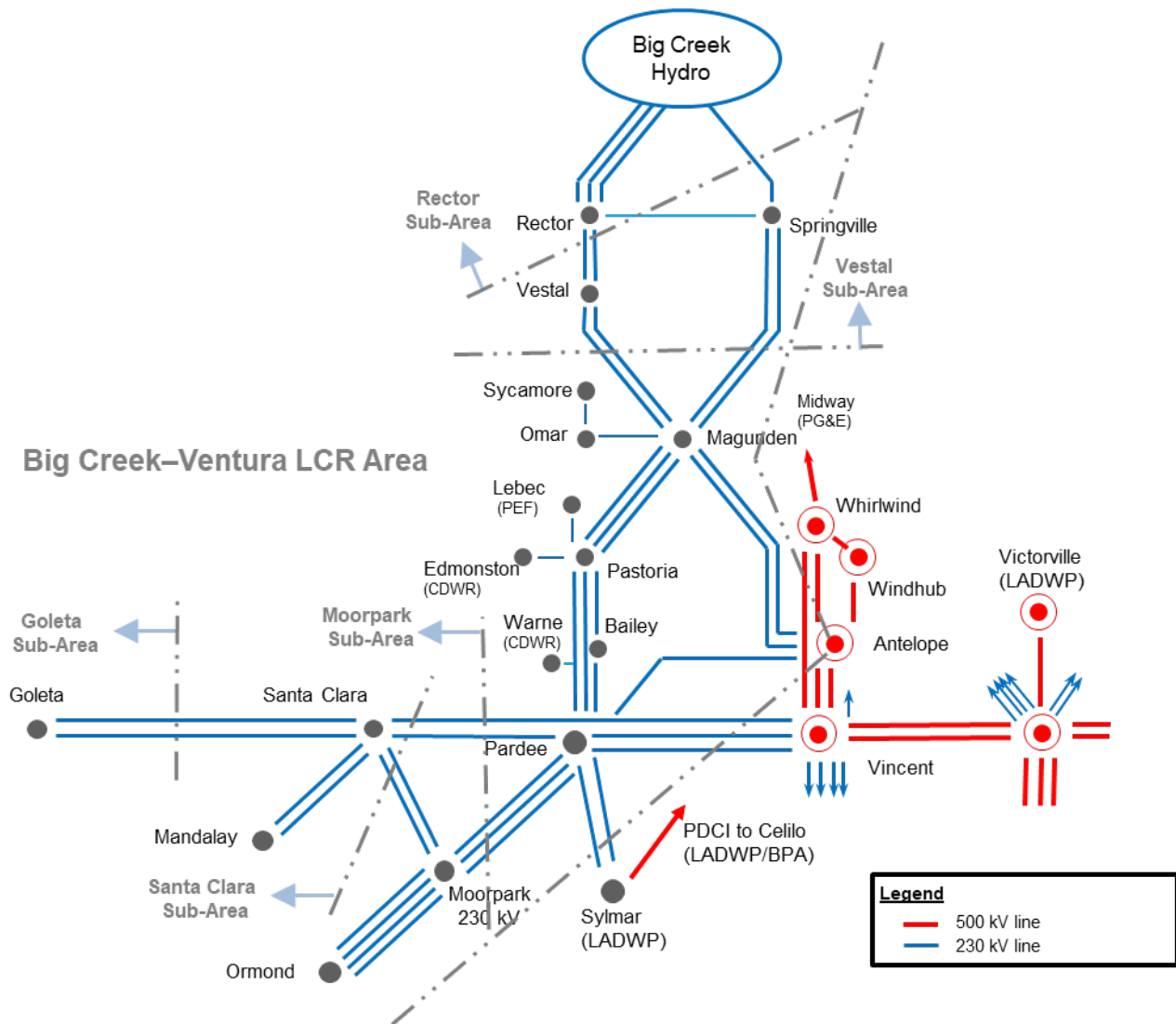
Figure 3.5-76 Big Creek/Ventura LCR Area
