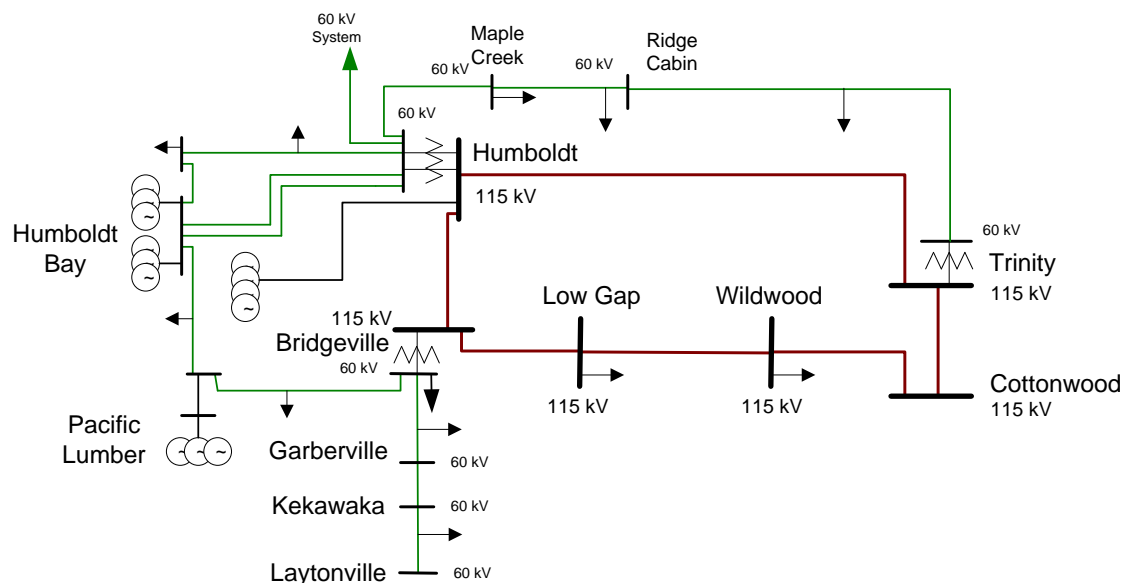
Figure 3.5-1 Humboldt LCR Area
