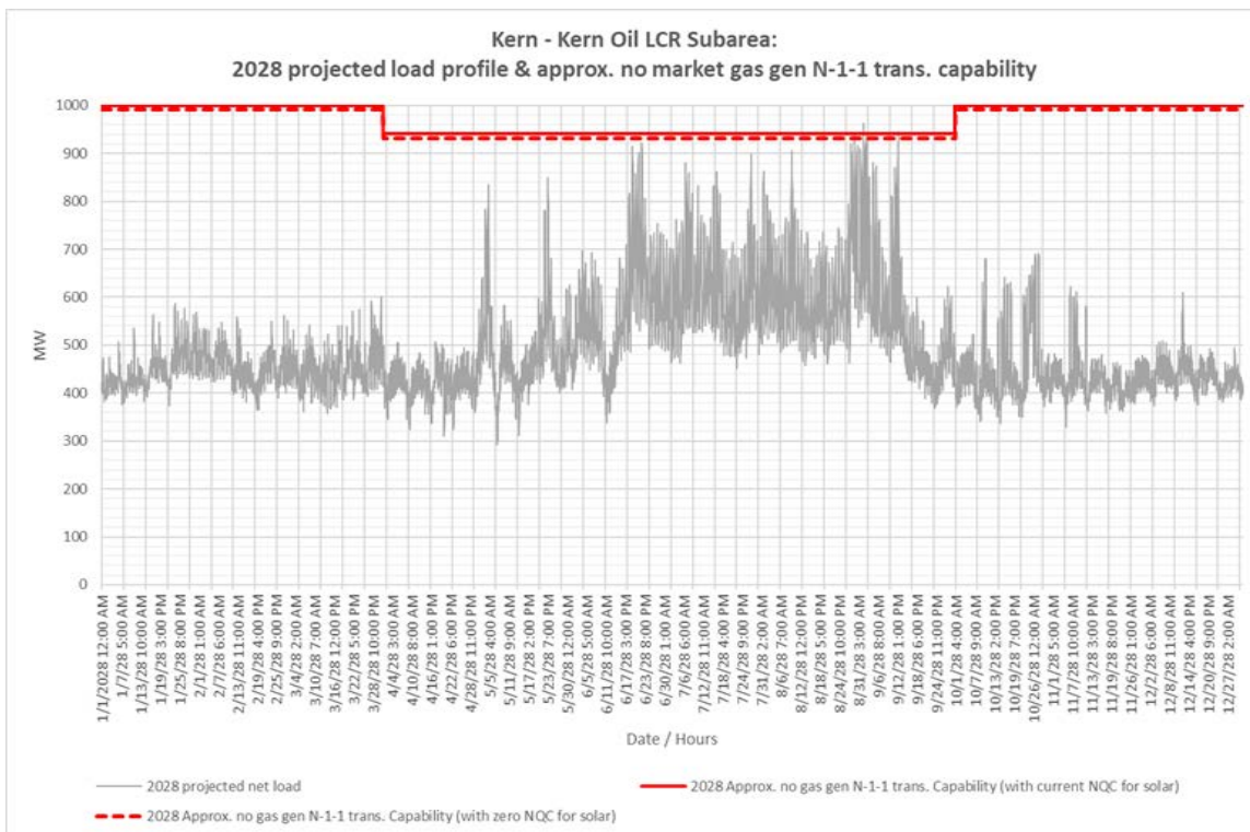
Figure 3.5-75 Kern Oil LCR Sub-area 2028 Forecast Hourly Profiles
