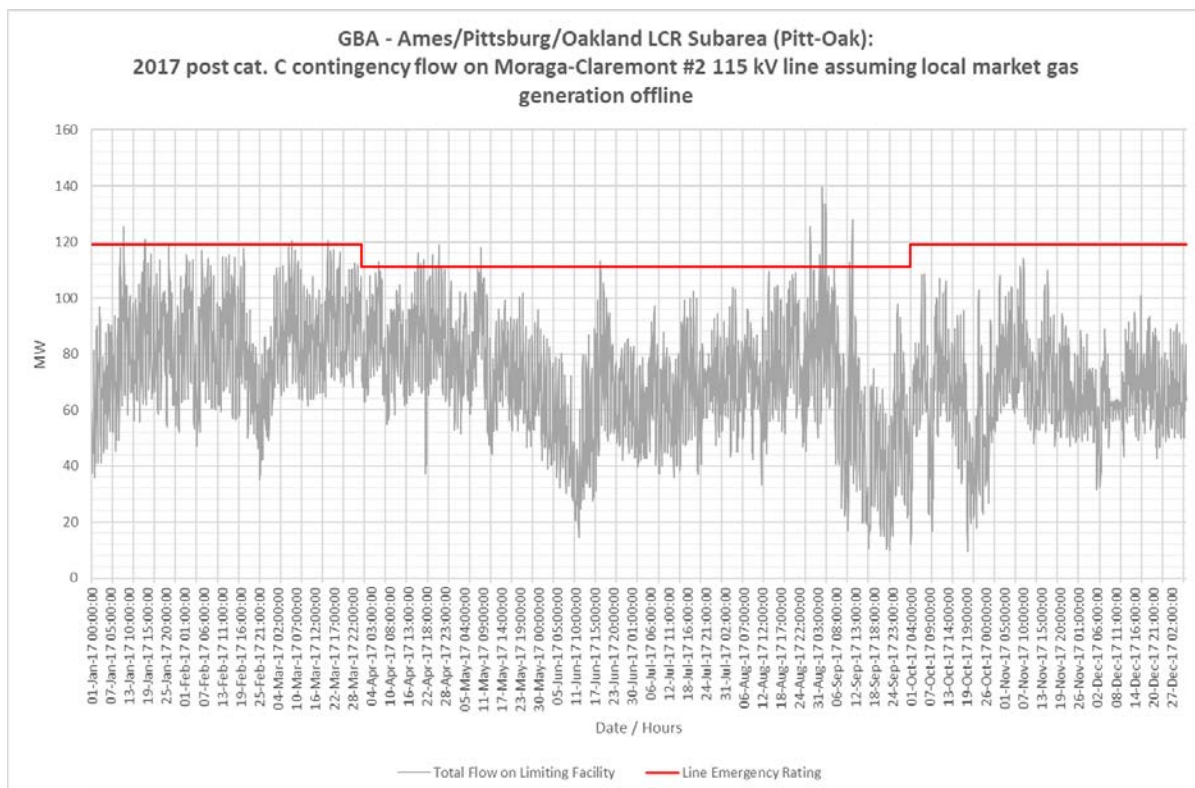
Figure 3.5-42 Ames-Pittsburg-Oakland LCR Sub-area 2017 Limiting Post Contingency Hourly Profiles (Moraga-Claremont #2 115 kV line)
