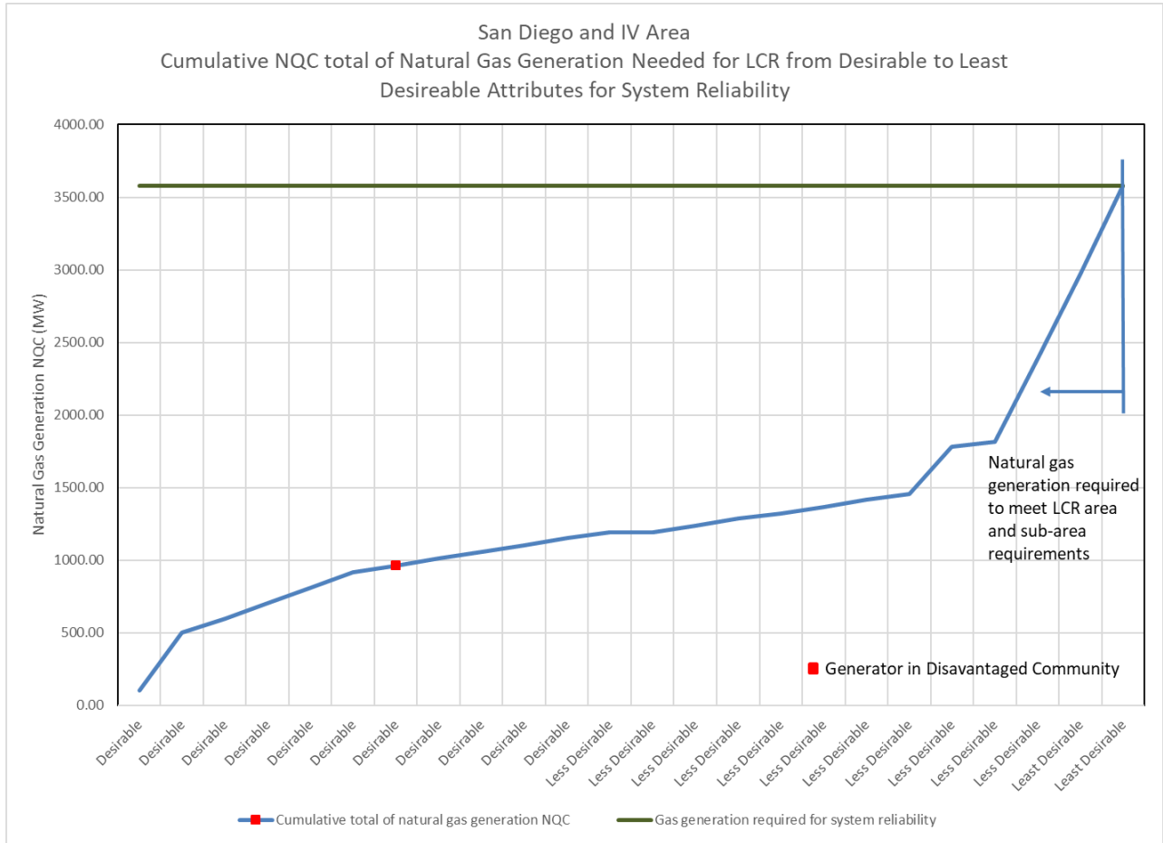
Figure C-1 San Diego and IV Area Gas-Fired Flexible Attributes
