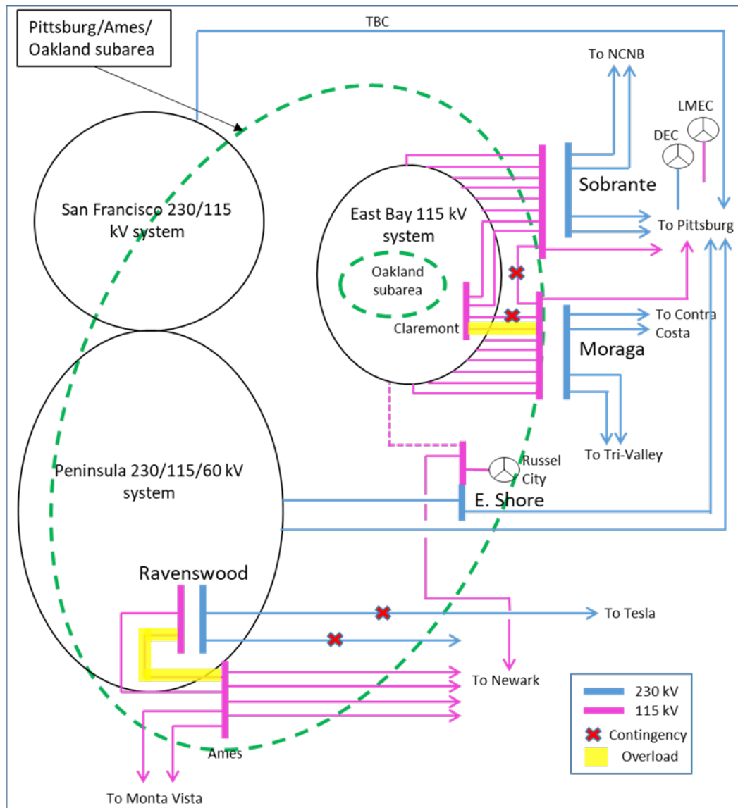
Figure 3.5-40 Ames-Pittsburg-Oakland LCR Sub-area
