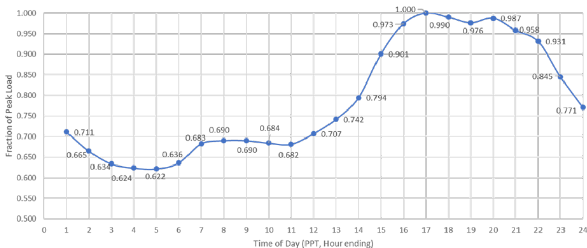
Figure 3.5-86 Western LA Basin LCR Sub-area 2028 Peak Day Forecast Profiles
