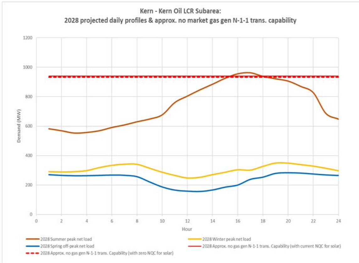
Figure 3.5-75 Kern Oil LCR Sub-area 2028 Forecast Hourly Profiles
