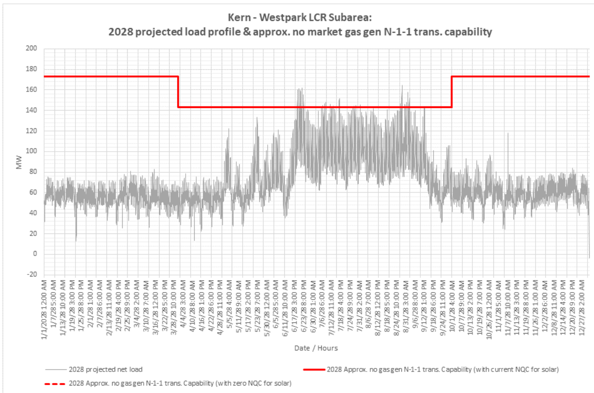
Figure 3.5-72 Westpark LCR Sub-area 2028 Forecast Hourly Profiles
