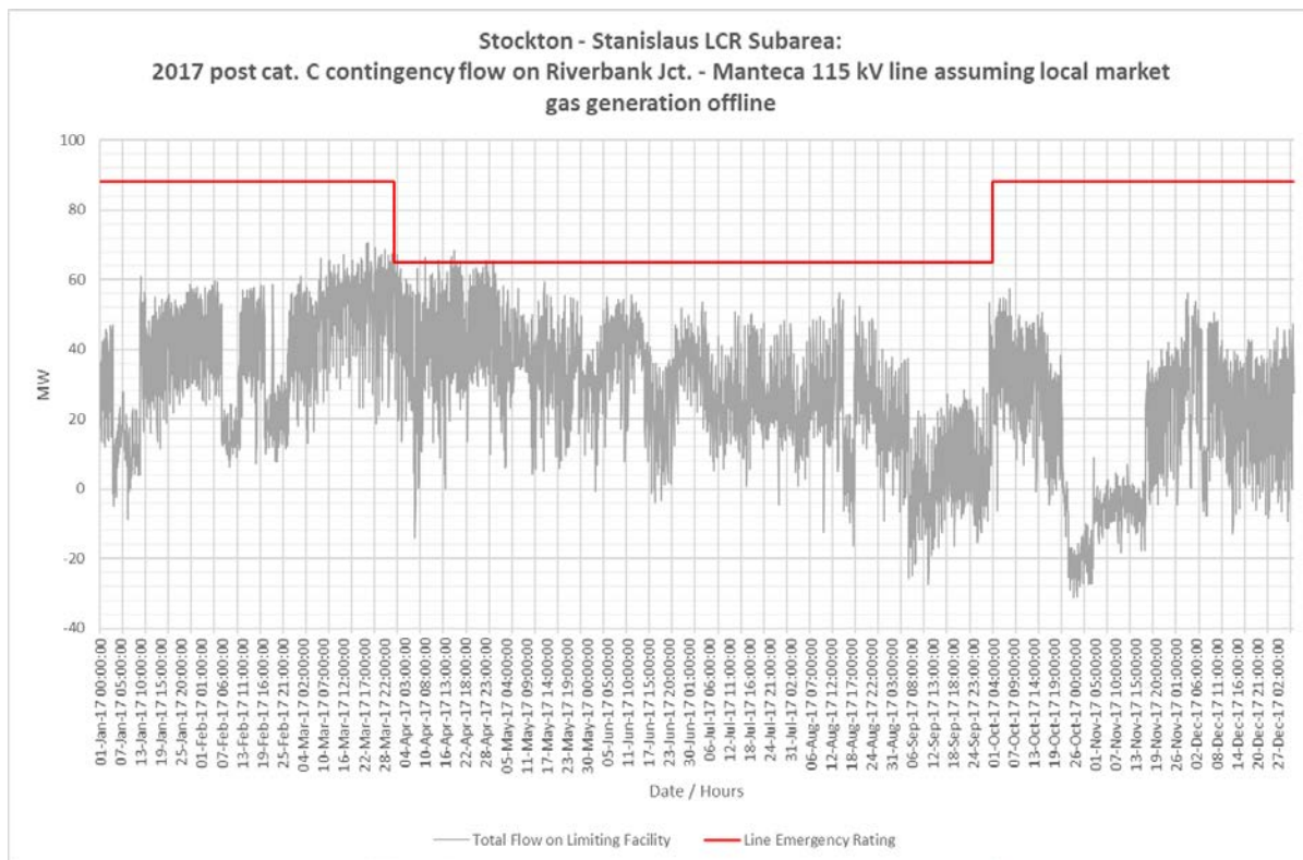
Figure 3.5-25 Stanislaus LCR Sub-area 2017 Limiting Post Contingency Hourly Profiles
