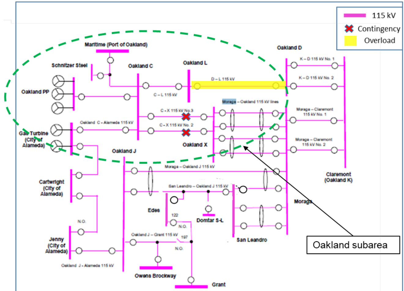
Figure 3.5-37 Oakland LCR Sub-area
