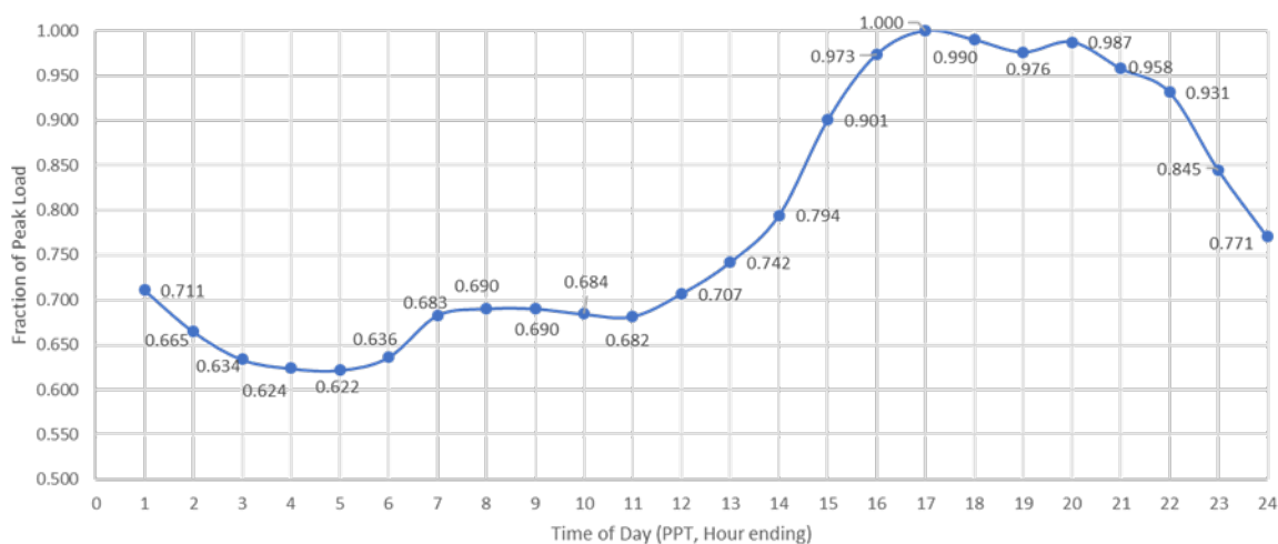
Figure 3.5-83 Big Creek/Ventura LCR area 2028 Peak Day Forecast Profiles
