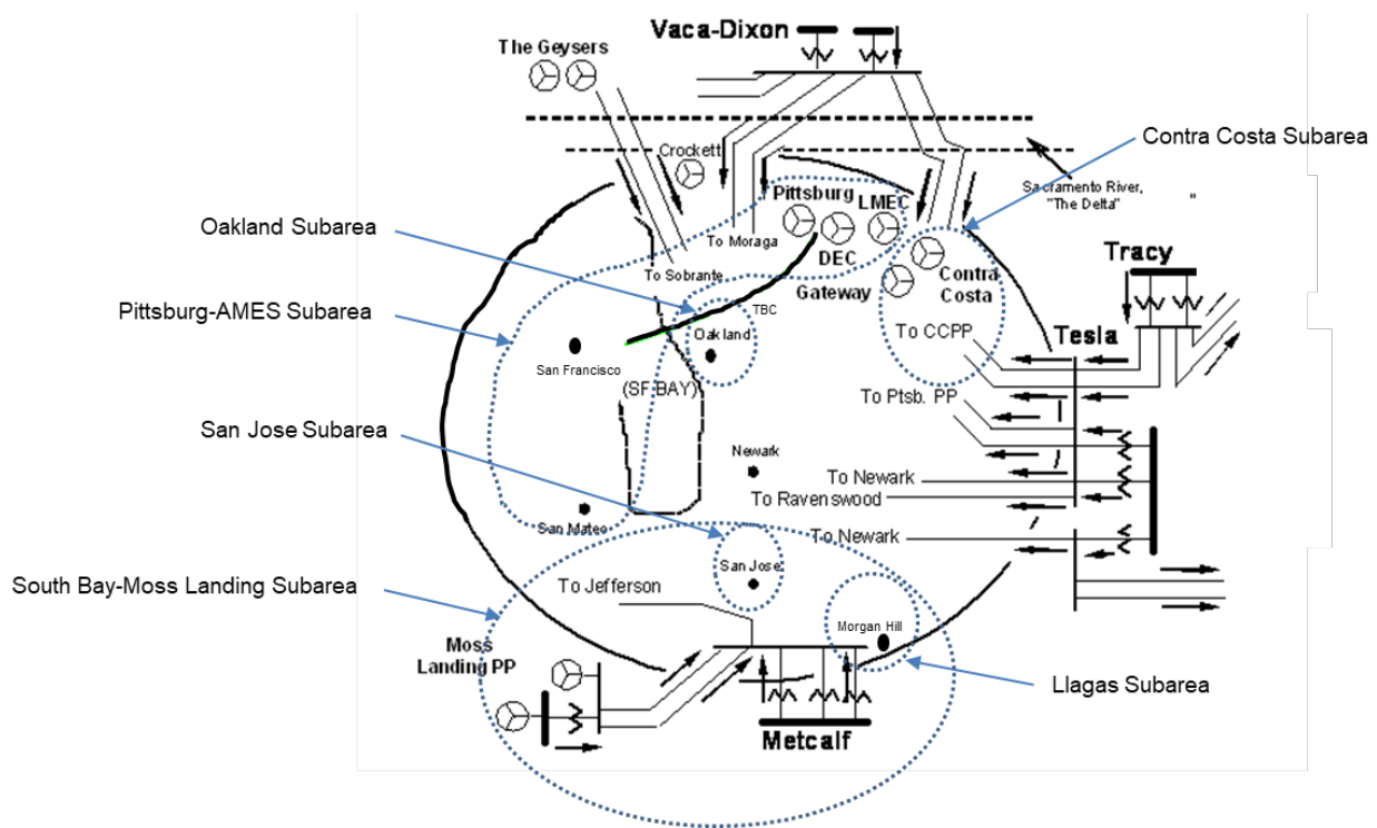
Figure 3.5-29 Greater Bay LCR Area
