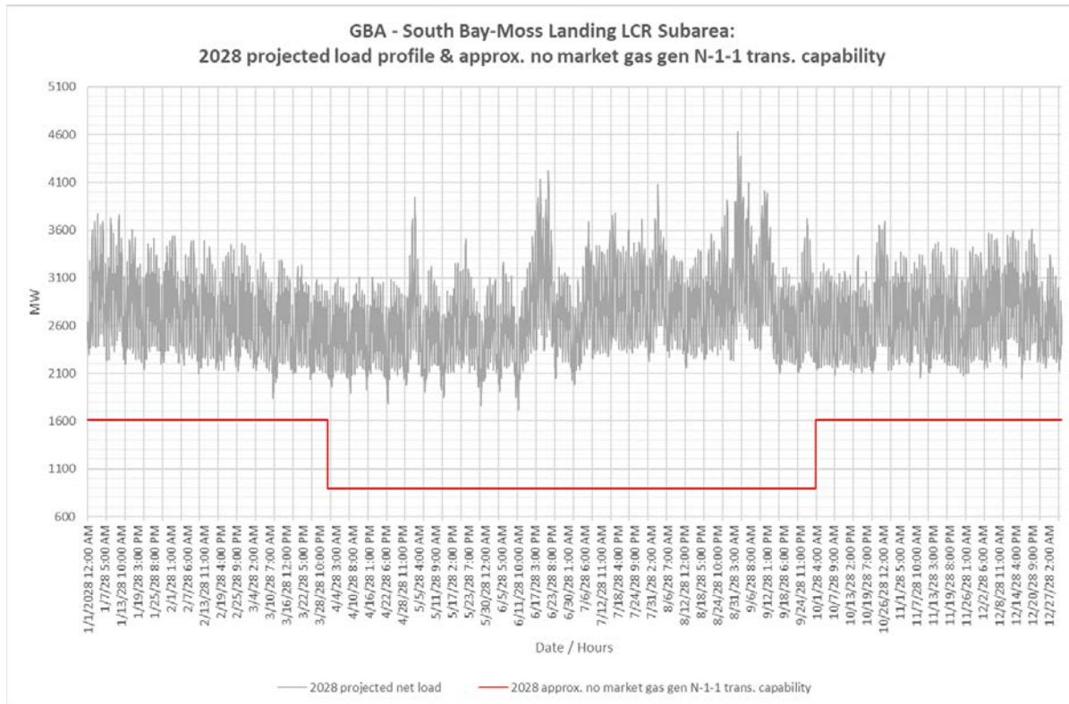
Figure 3.5-36 South Bay-Moss Landing LCR Sub-area 2028 Forecast Hourly Profiles
