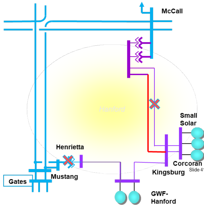
Figure 3.5-49 Hanford LCR Sub-area
