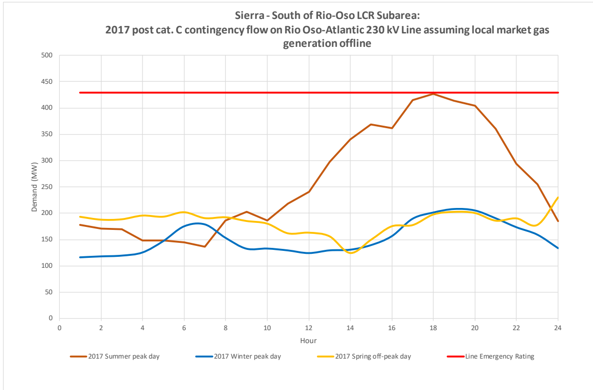
Figure 3.5-15 South of Rio Oso LCR Sub-area 2017 Limiting Post Contingency Peak Day Profiles
