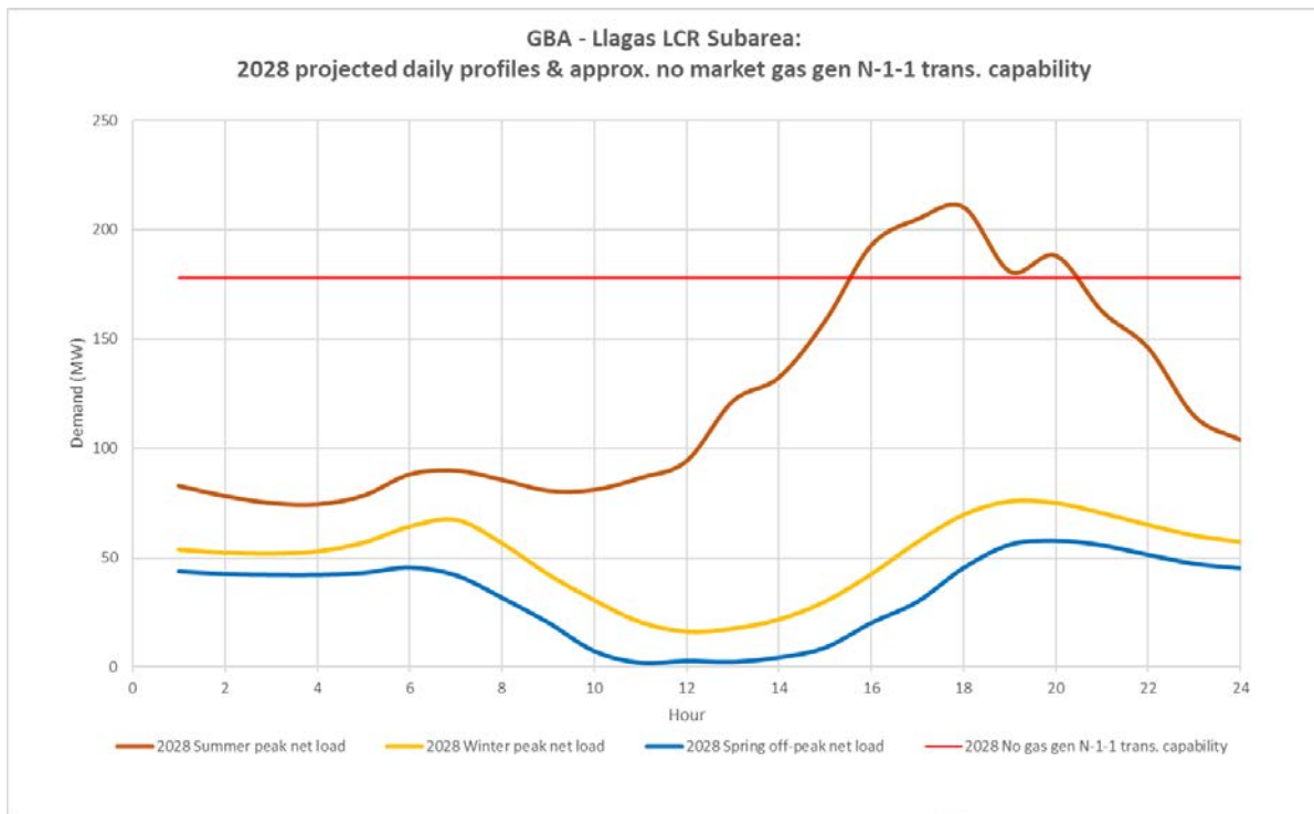
Figure 3.5-31 Llagas LCR Sub-area 2028 Peak Day Forecast Profiles
