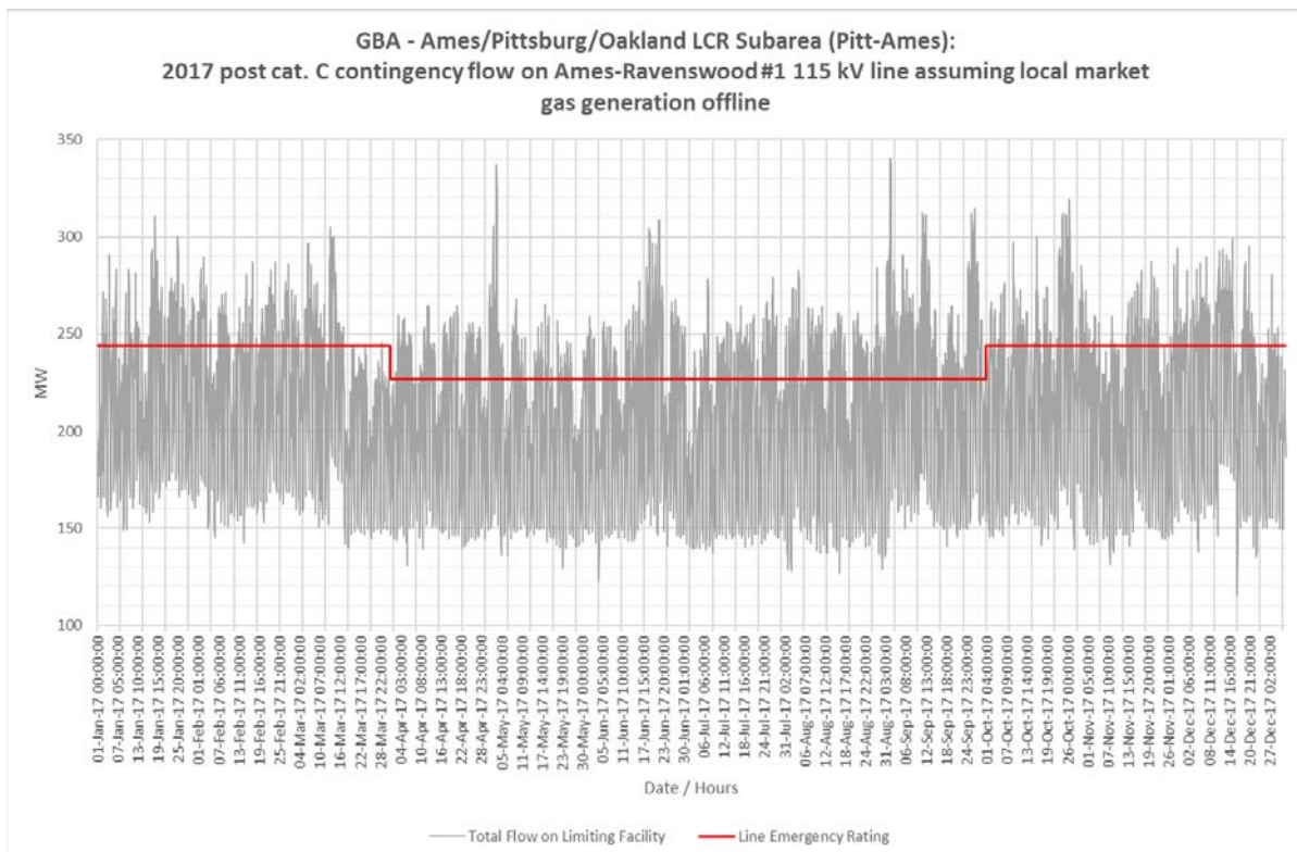
Figure 3.5-44 Ames-Pittsburg-Oakland LCR Sub-area 2017 Limiting Post Contingency Hourly Profiles (Ames-Ravenswood #1 115 kV line)
