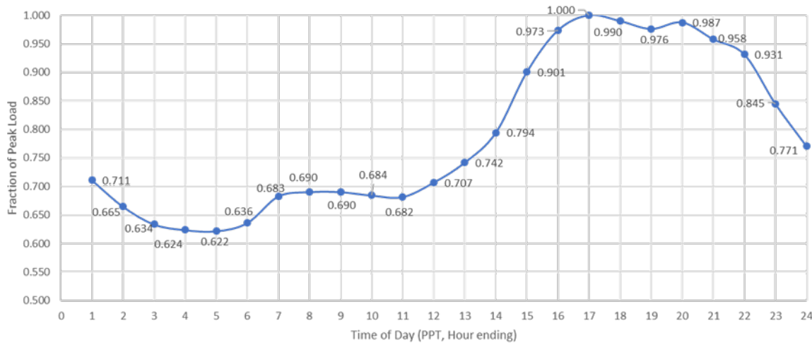
Figure 3.5-87 Eastern LA Basin LCR Sub-area 2028 Peak Day Forecast Profiles
