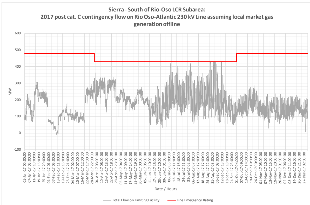
Figure 3.5-16 South of Rio Oso LCR Sub-area 2017 Limiting Post Contingency Hourly Profiles
