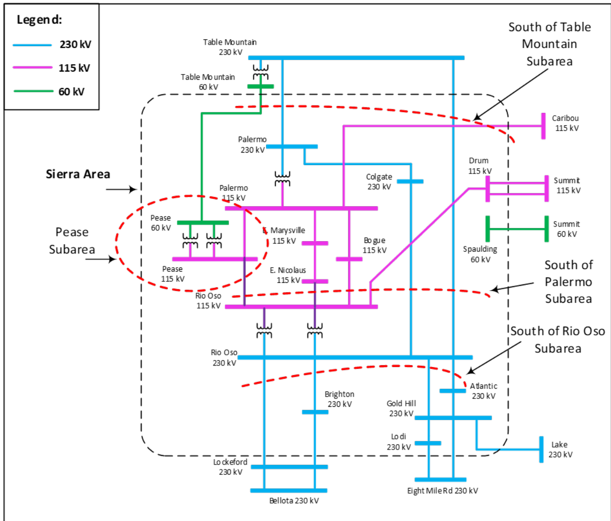
Figure 3.5-10 Sierra LCR Area
