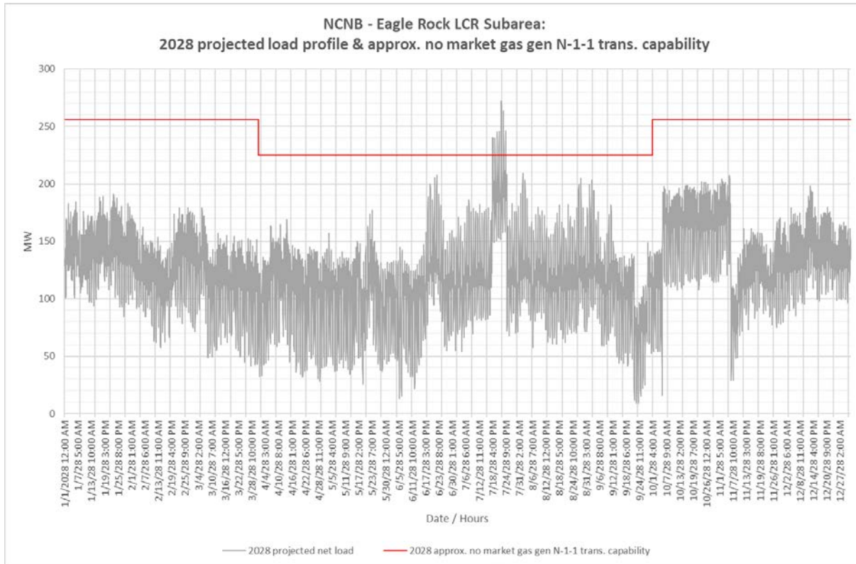
Figure 3.5-9 Eagle Rock LCR Sub-area 2028 Forecast Hourly Profiles
