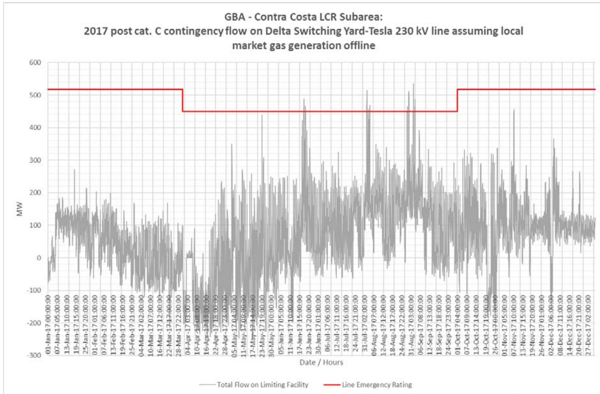
Figure 3.5-47 Contra Costa LCR Sub-area 2017 Limiting Post Contingency Hourly Profiles
