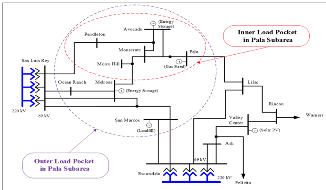
Figure 3.5-96 Pala Outer LCR Sub-area
