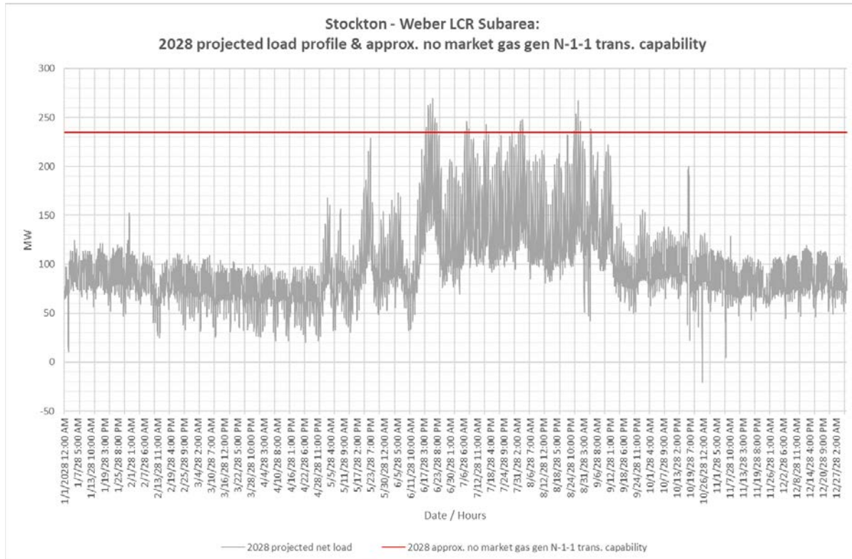
Figure 3.5-22 Weber LCR Sub-area 2028 Forecast Hourly Profiles
