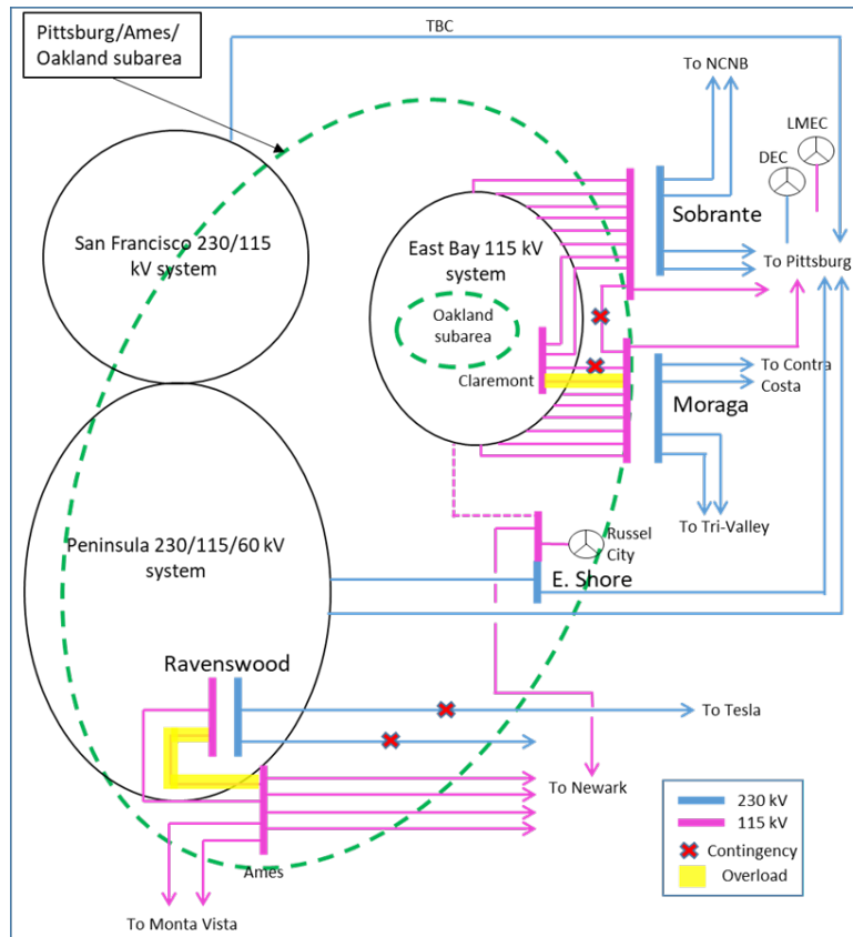
Figure 3.5-40 Ames-Pittsburg-Oakland LCR Sub-area
