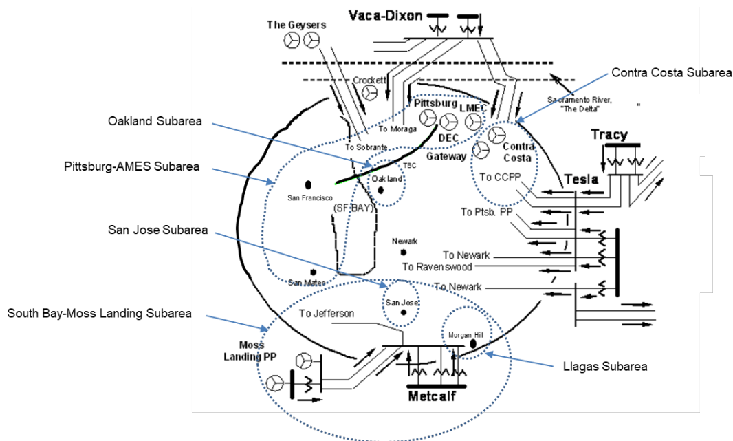
Figure 3.5-29 Greater Bay LCR Area
