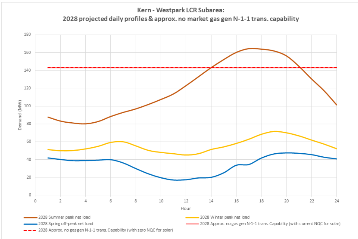
Figure 3.5-72 Westpark LCR Sub-area 2028 Forecast Hourly Profiles
