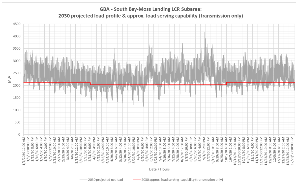
Figure 3.6-26 South Bay-Moss Landing LCR Sub-area 2030 Forecast Hourly Profiles
