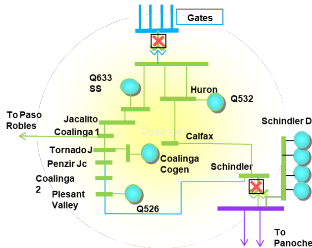
Figure 3.6-38 Coalinga LCR Sub-area
