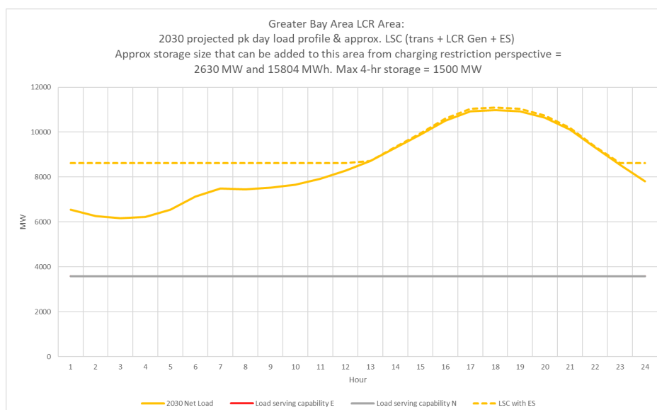
Figure 3.6-32 Bay Area LCR Area 2030 Peak Day Forecast Profiles
