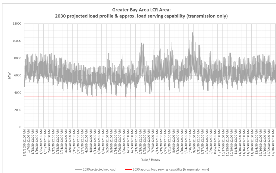
Figure 3.6-33 Bay Area LCR Area 2030 Forecast Hourly Profiles
