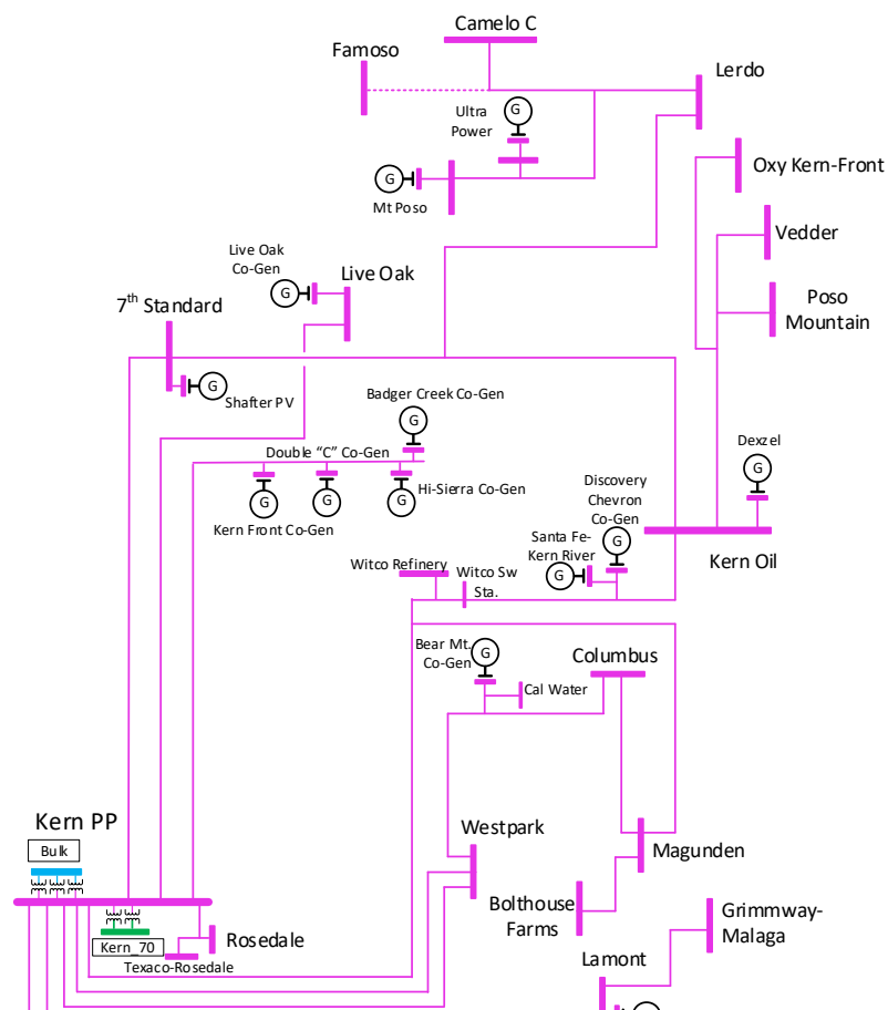
Figure 3.6-56 Kern Oil LCR Sub-area
