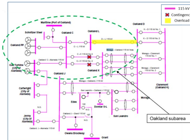
Figure 3.6-27 Oakland LCR Sub-area
