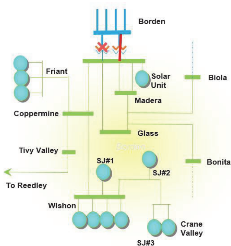
Figure 3.3-53 Borden LCR Sub-area
