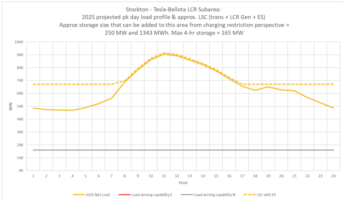
Figure 3.3-30 Tesla-Bellota LCR Sub-area 2025 Forecast Hourly Profiles
