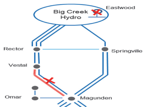
Figure 3.3-77 Vestal LCR Sub-area
