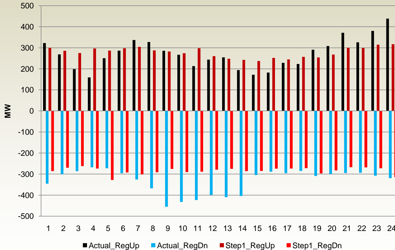
Regulation Comparison (Actual vs. Step 1) Summer 2010
