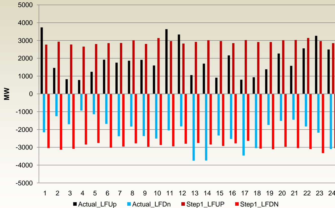
Load Following Comparison (Actual vs. Step 1) Summer 2010
