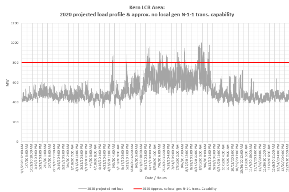
Figure 3.3-92 South Kern PP LCR Sub-area 2020 Forecast Hourly Profiles
