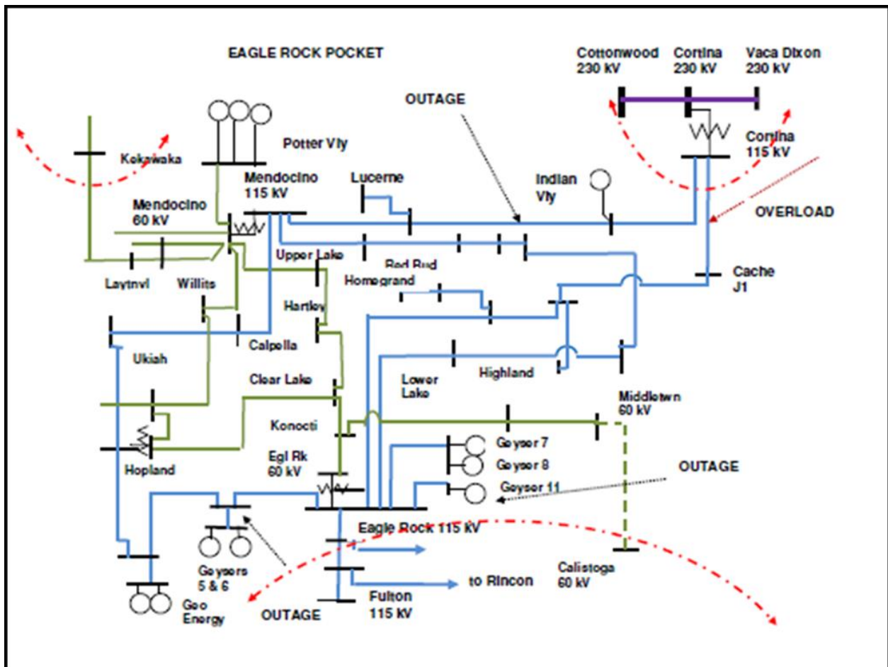
Figure 3.3-7 Eagle Rock LCR Sub-area
