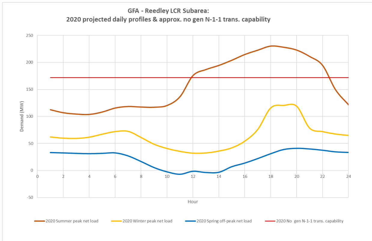
Figure 3.3-73 Reedley LCR Sub-area 2020 Peak Day Forecast Profiles
