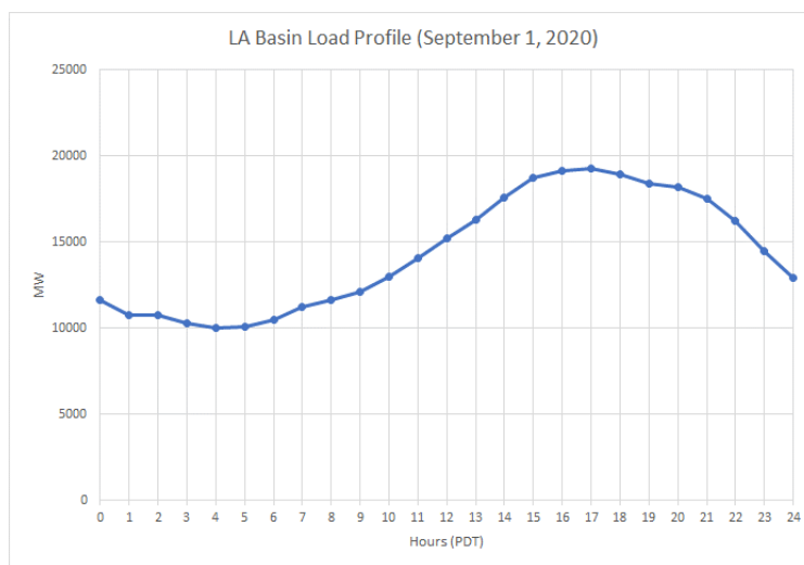
Figure 3.3-105 LA Basin LCR area 2020 Peak Day Forecast Profiles
