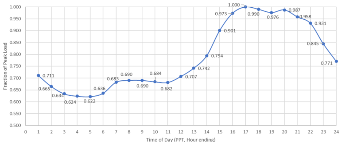
Figure 3.3-104 Eastern LA Basin LCR Sub-area 2020 Peak Day Forecast Profiles
