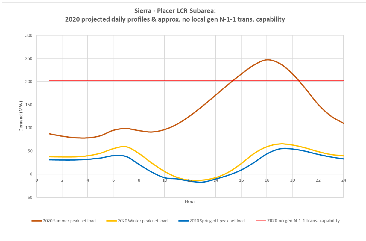
Figure 3.3-16 Placer LCR Sub-area 2020 Forecast Hourly Profiles
