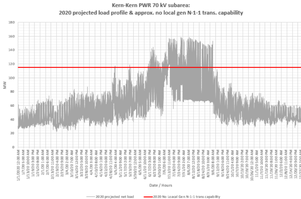
Figure 3.3-84 Kern 70 kV LCR Sub-area 2020 Forecast Hourly Profiles
