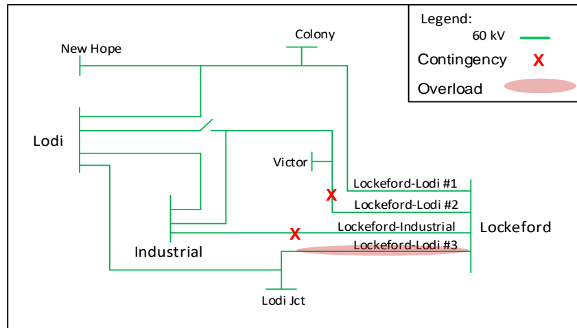
Figure 3.3-34 Lockeford LCR Sub-area
