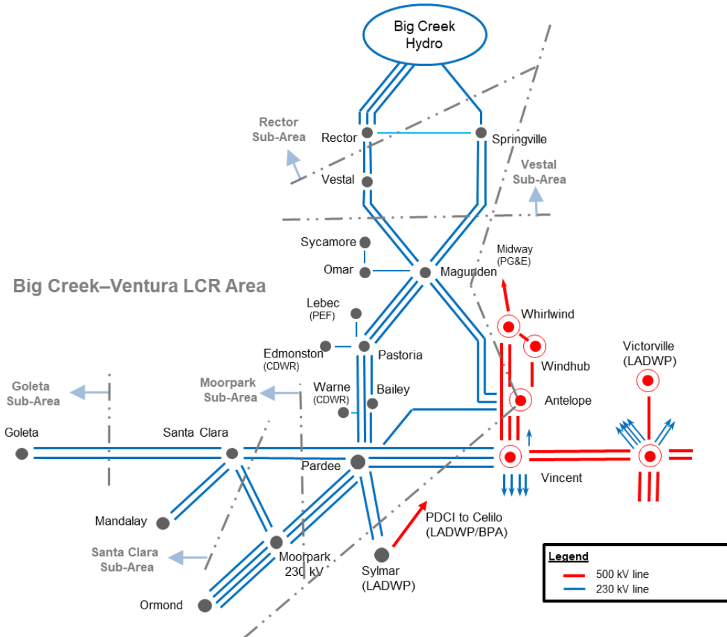
Figure 3.3-93 Big Creek/Ventura LCR Area
