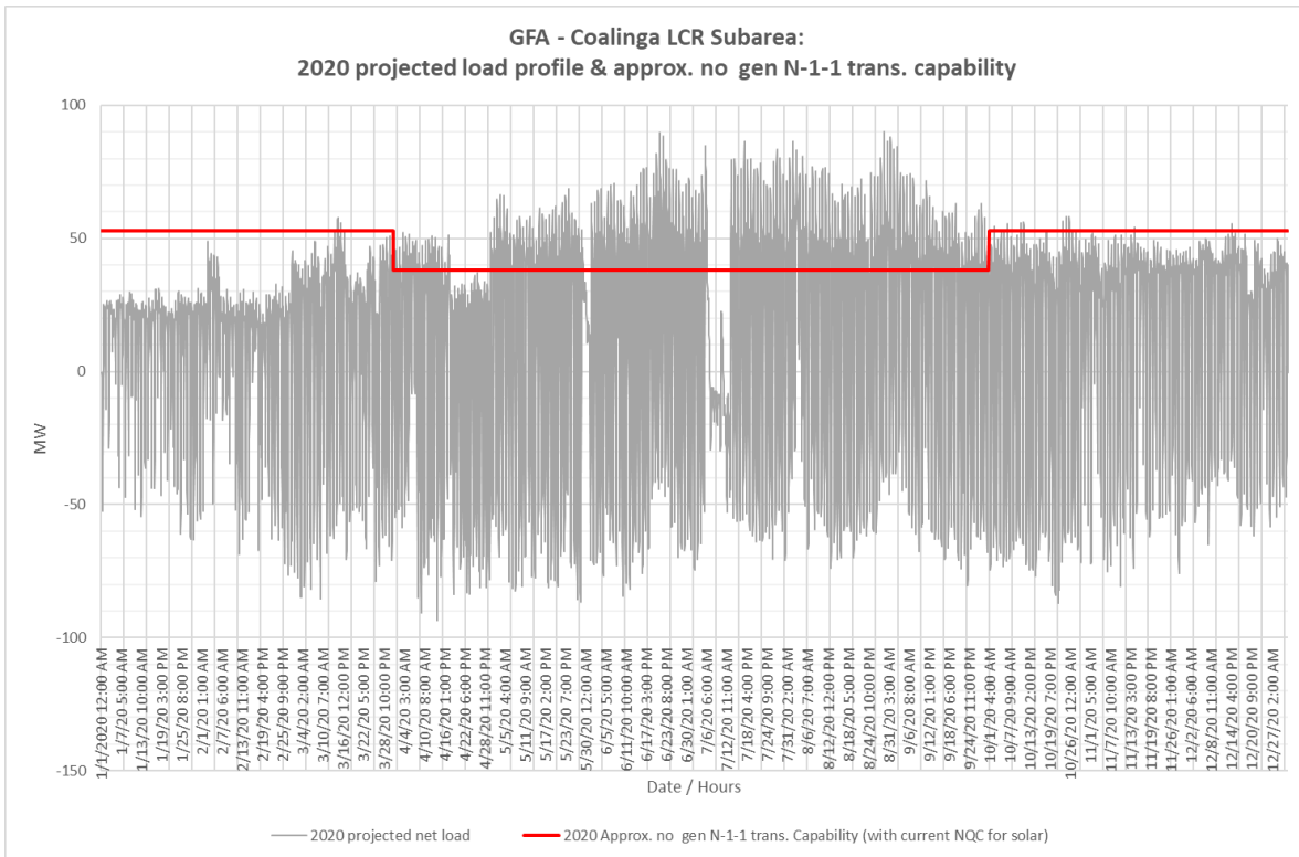
Figure 3.3-68 Coalinga LCR Sub-area 2020 Forecast Hourly Profiles
