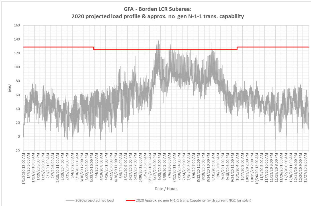
Figure 3.3-71 Borden LCR Sub-area 2020 Forecast Hourly Profiles
