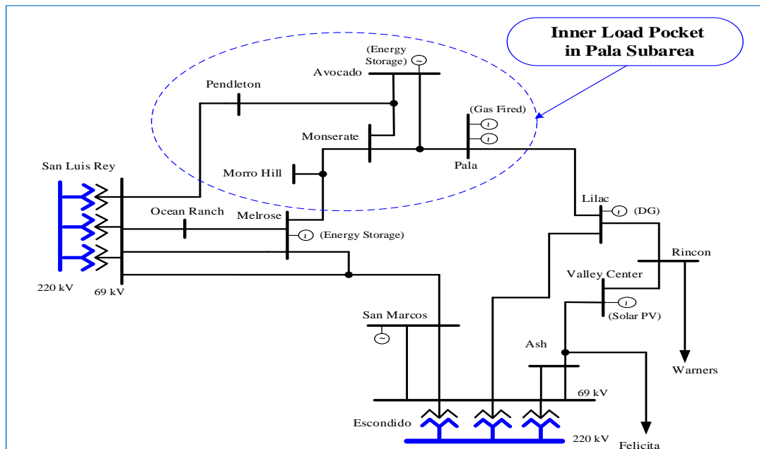
Figure 3.3-111 Pala Inner LCR Sub-area
