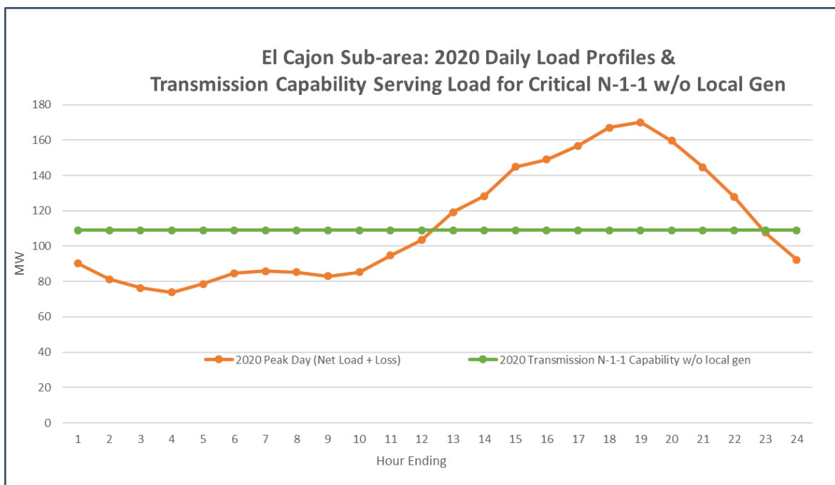
Figure 3.3-108 El Cajon LCR Sub-area 2020 Peak Day Forecast Profiles
