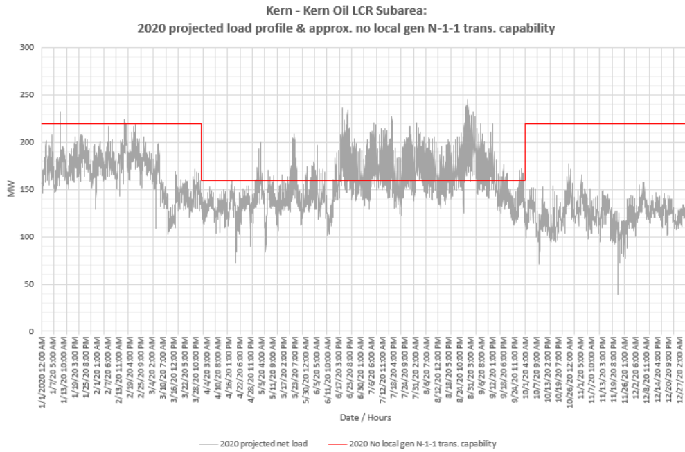
Figure 3.3-89 Kern Oil LCR Sub-area 2020 Forecast Hourly Profiles
