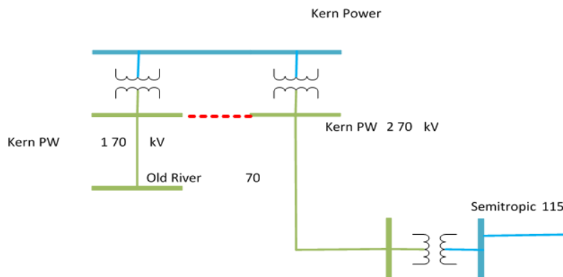
Figure 3.3-82 Kern 70 kV LCR Sub-area
