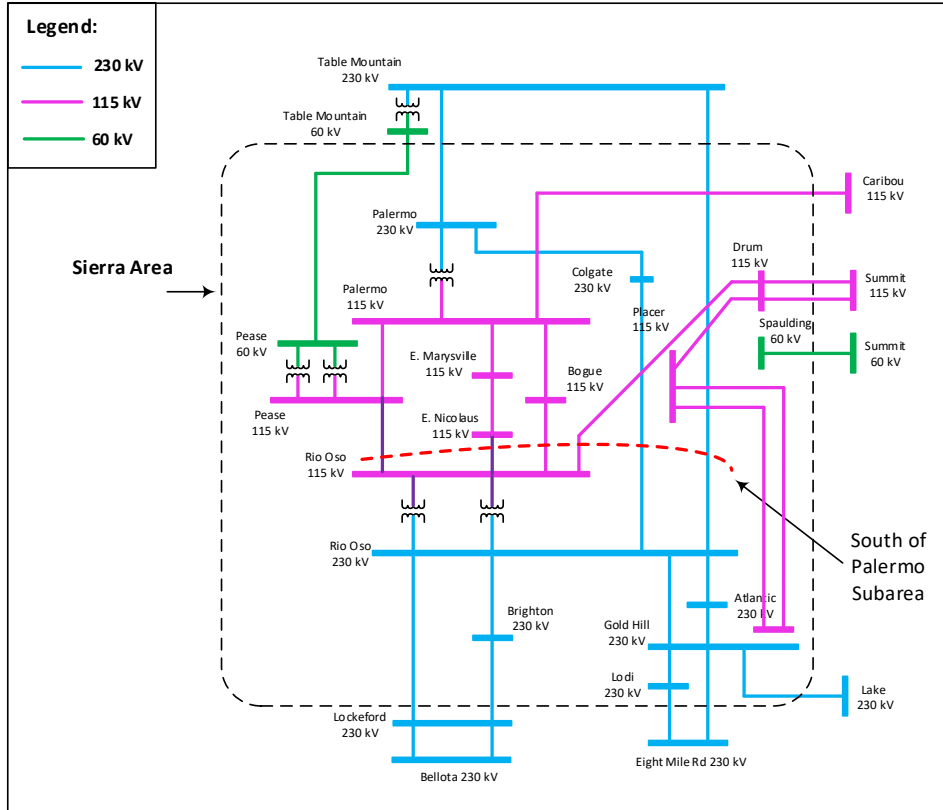
Figure 3.3-26 South of Palermo LCR Sub-area
