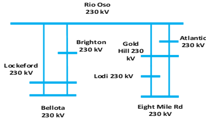
Figure 3.3-23 South of Rio Oso LCR Sub-area
