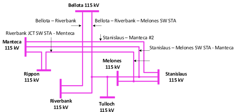
Figure 3.3-37 Stanislaus LCR Sub-area
