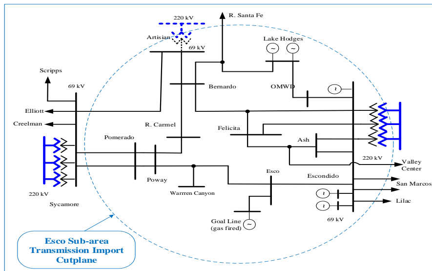
Figure 3.3-109 Esco LCR Sub-area
