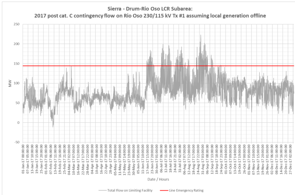
Figure 3.3-22 Drum-Rio Oso LCR Sub-area 2017 Limiting Post Contingency Hourly Profiles
