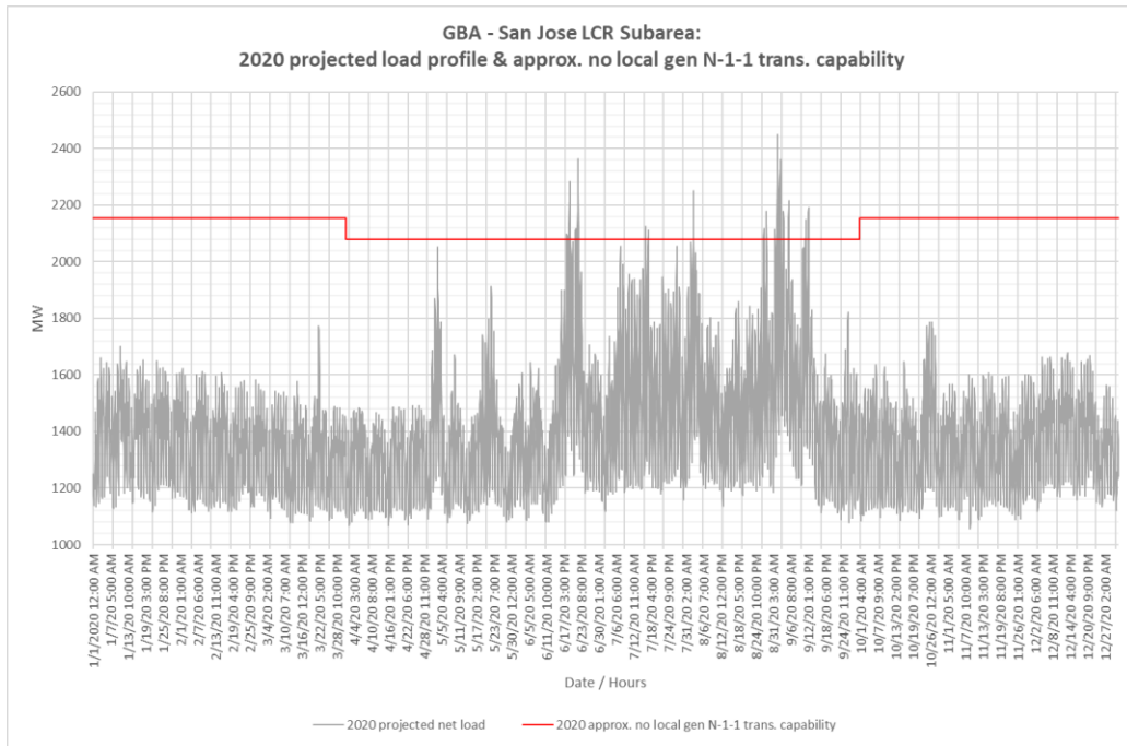
Figure 3.3-48 San Jose LCR Sub-area 2020 Forecast Hourly Profiles
