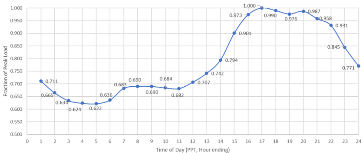
Figure 3.3-103 Western LA Basin LCR Sub-area 2020 Peak Day Forecast Profiles
