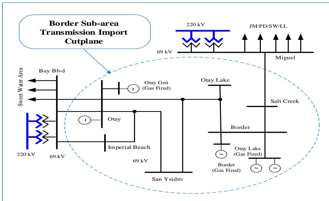
Figure 3.3-115 Border LCR Sub-area
