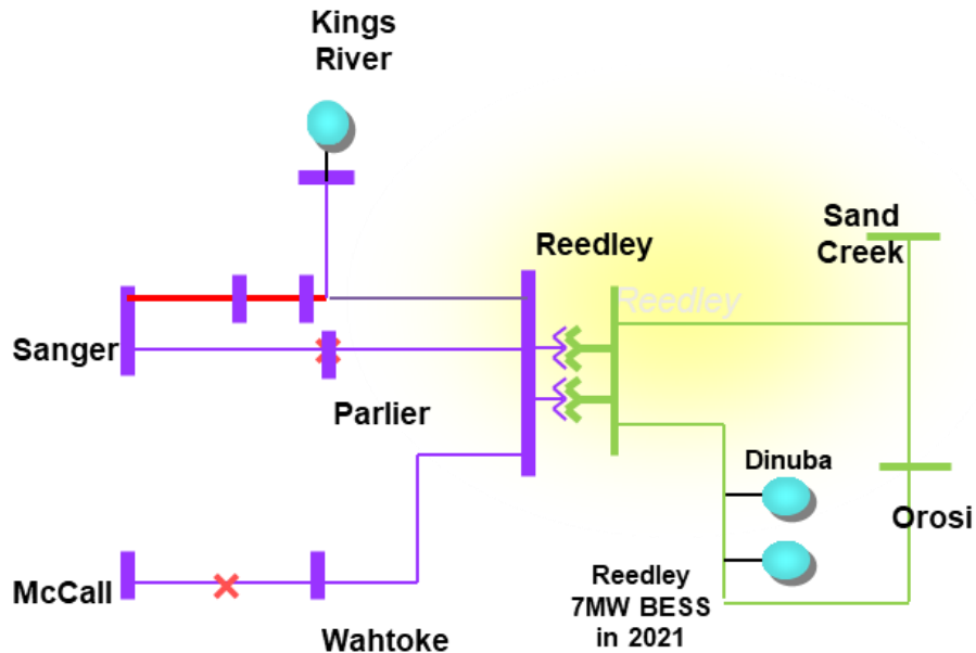
Figure 3.3-72 Reedley LCR Sub-area
