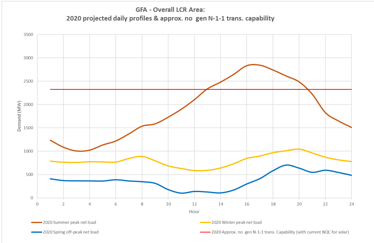
Figure 3.3-79 Fresno LCR area 2020 Peak Day Forecast Profiles
