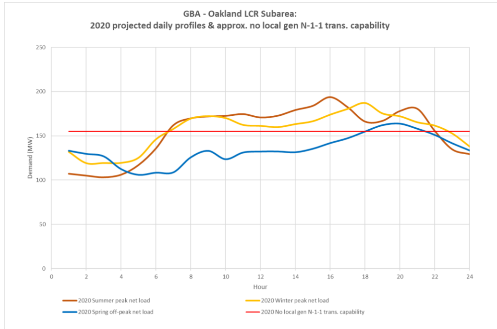
Figure 3.3-53 Oakland LCR Sub-area 2020 Forecast Hourly Profiles
