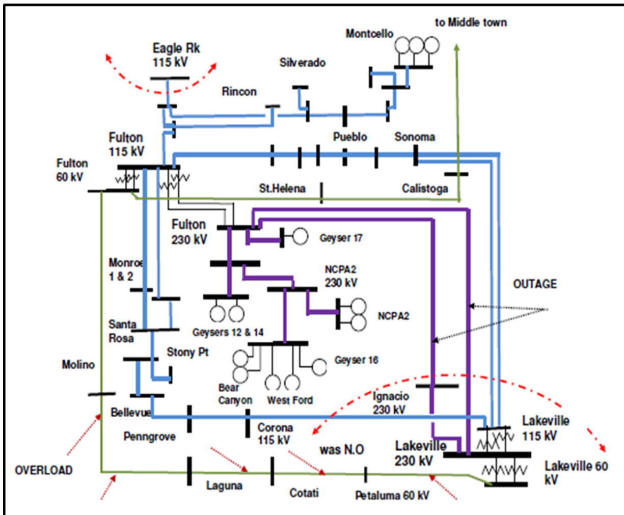
Figure 3.3-10 Fulton LCR Sub-area
