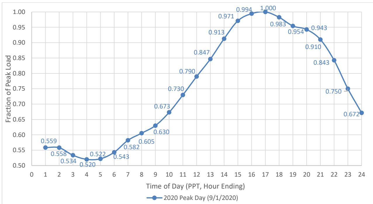
Figure 3.3-99 Moorpark LCR Sub-area 2020 Peak Day Forecast Profiles
