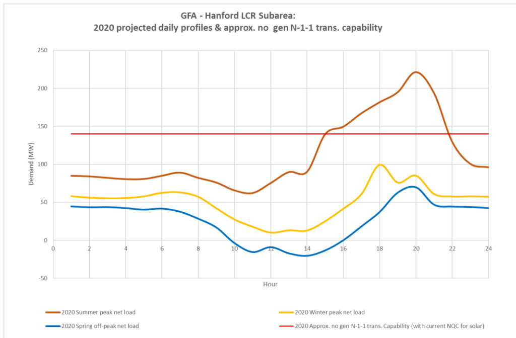
Figure 3.3-64 Hanford LCR Sub-area 2020 Peak Day Forecast Profiles
