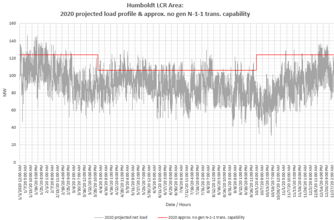
Figure 3.3-3 Humboldt 2020 Forecast Hourly Profile
