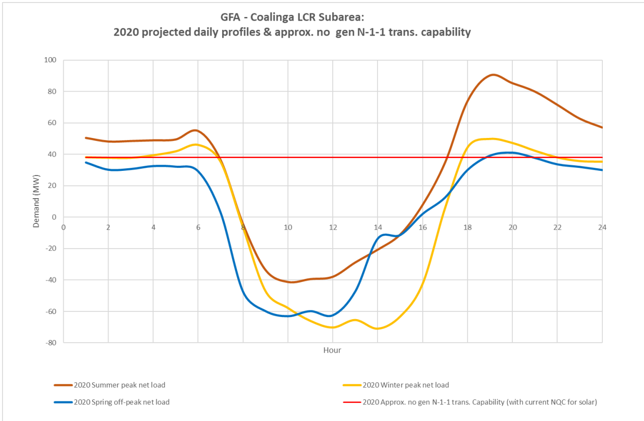
Figure 3.3-68 Coalinga LCR Sub-area 2020 Forecast Hourly Profiles
