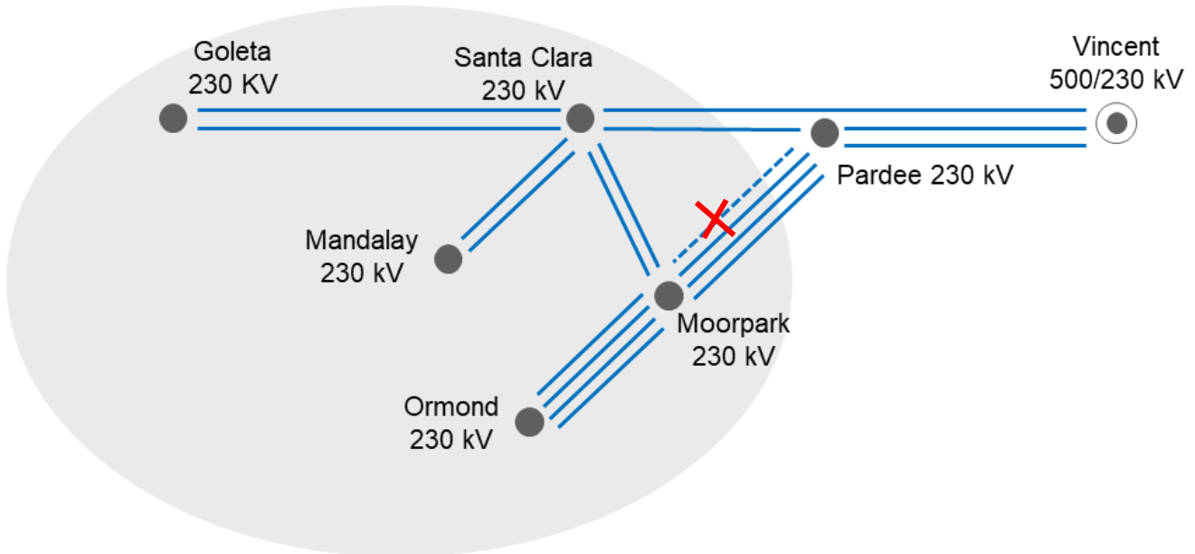
Figure 3.3-98 Moorpark LCR Sub-area
