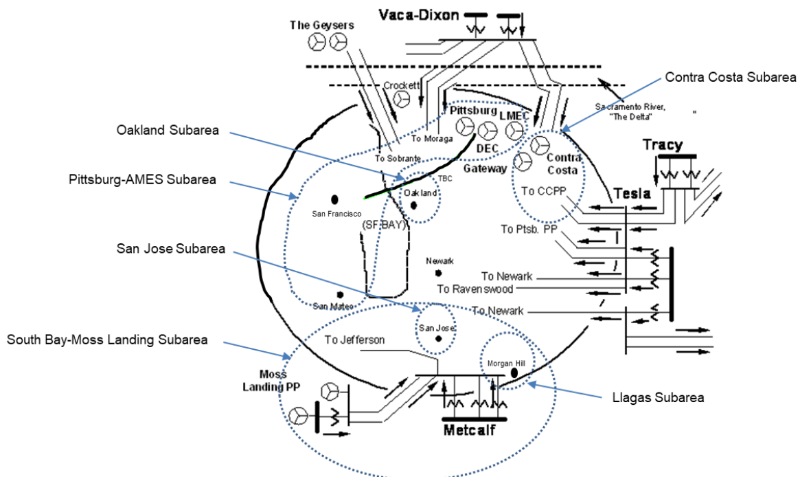
Figure 3.3-43 Greater Bay LCR Area
