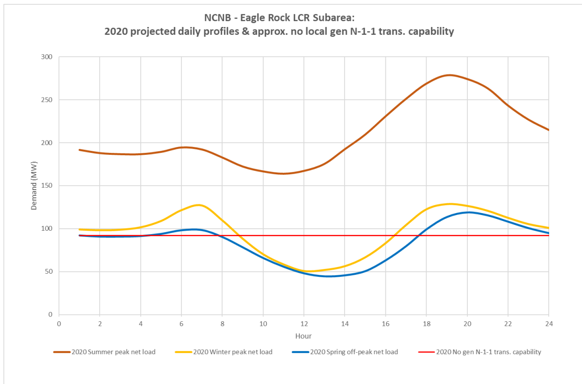
Figure 3.3-8 Eagle Rock LCR Sub-area 2020 Peak Day Forecast Profiles
