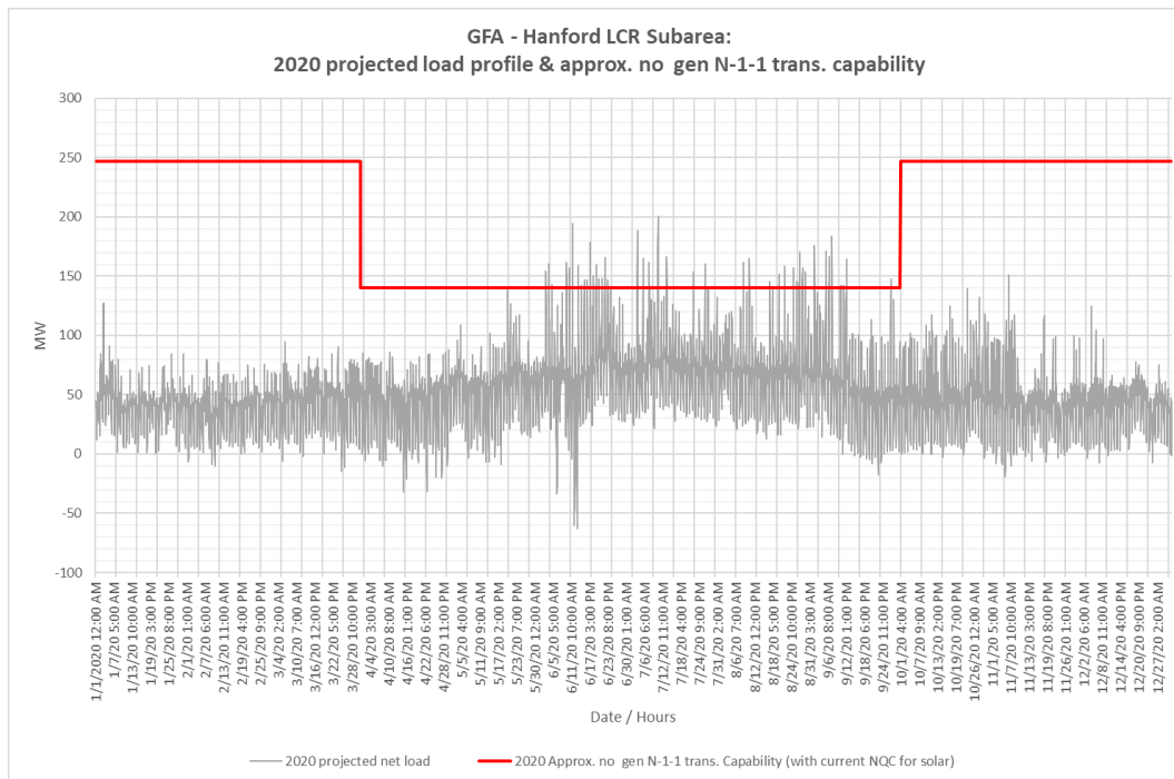
Figure 3.3-65 Hanford LCR Sub-area 2020 Forecast Hourly Profiles
