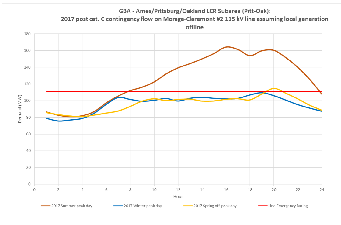
Figure 3.3-55 Ames-Pittsburg-Oakland LCR Sub-area 2017 Limiting Post Contingency Peak Day Profiles (Moraga-Claremont #2 115 kV line)
