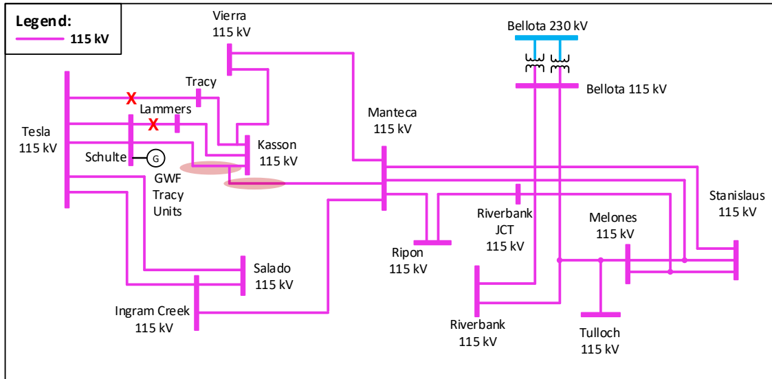
Figure 3.3-40 Tesla-Bellota LCR Sub-area
