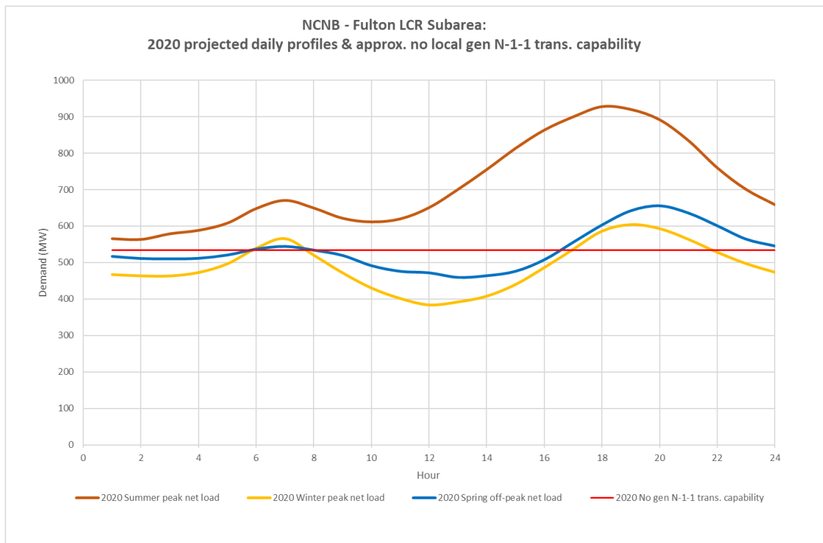
Figure 3.3-11 Fulton LCR Sub-area 2020 Peak Day Forecast Profiles
