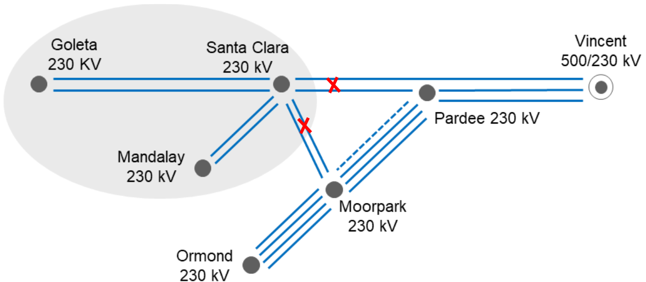
Figure 3.3-96 Santa Clara LCR Sub-area
