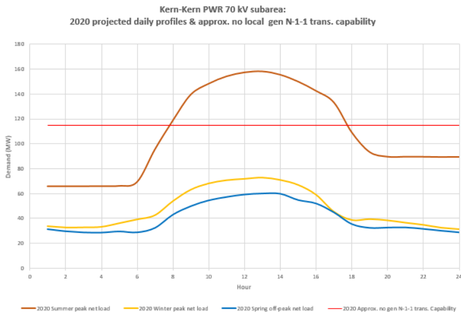
Figure 3.3-83 Kern 70 kV LCR Sub-area 2020 Peak Day Forecast Profiles
