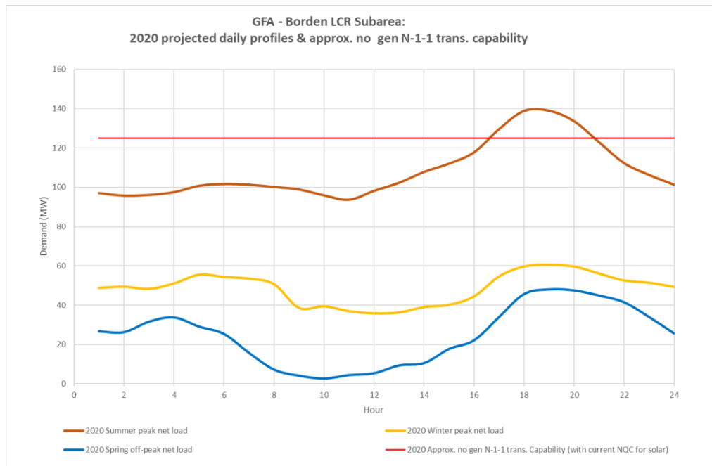
Figure 3.3-70 Borden LCR Sub-area 2020 Peak Day Forecast Profiles
