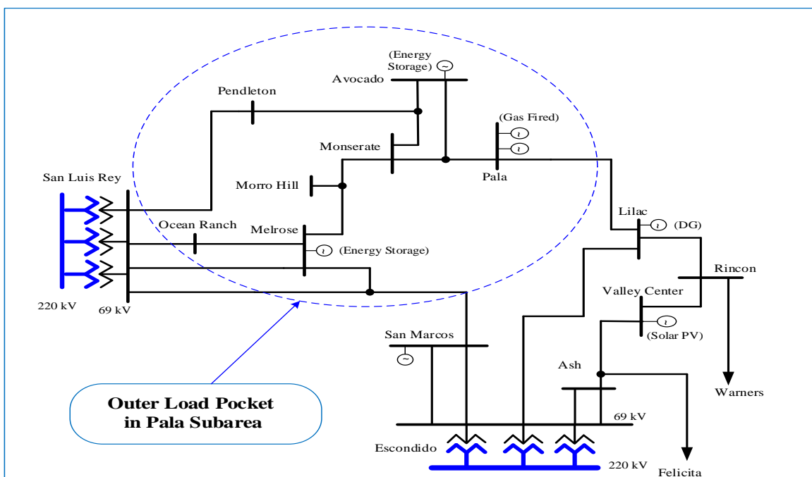
Figure 3.3-113 Pala Outer LCR Sub-area
