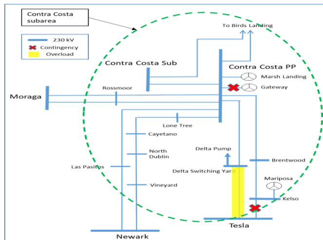
Figure 3.3-59 Contra Costa LCR Sub-area
