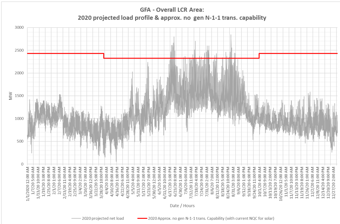
Figure 3.3-80 Fresno LCR area 2020 Forecast Hourly Profiles
