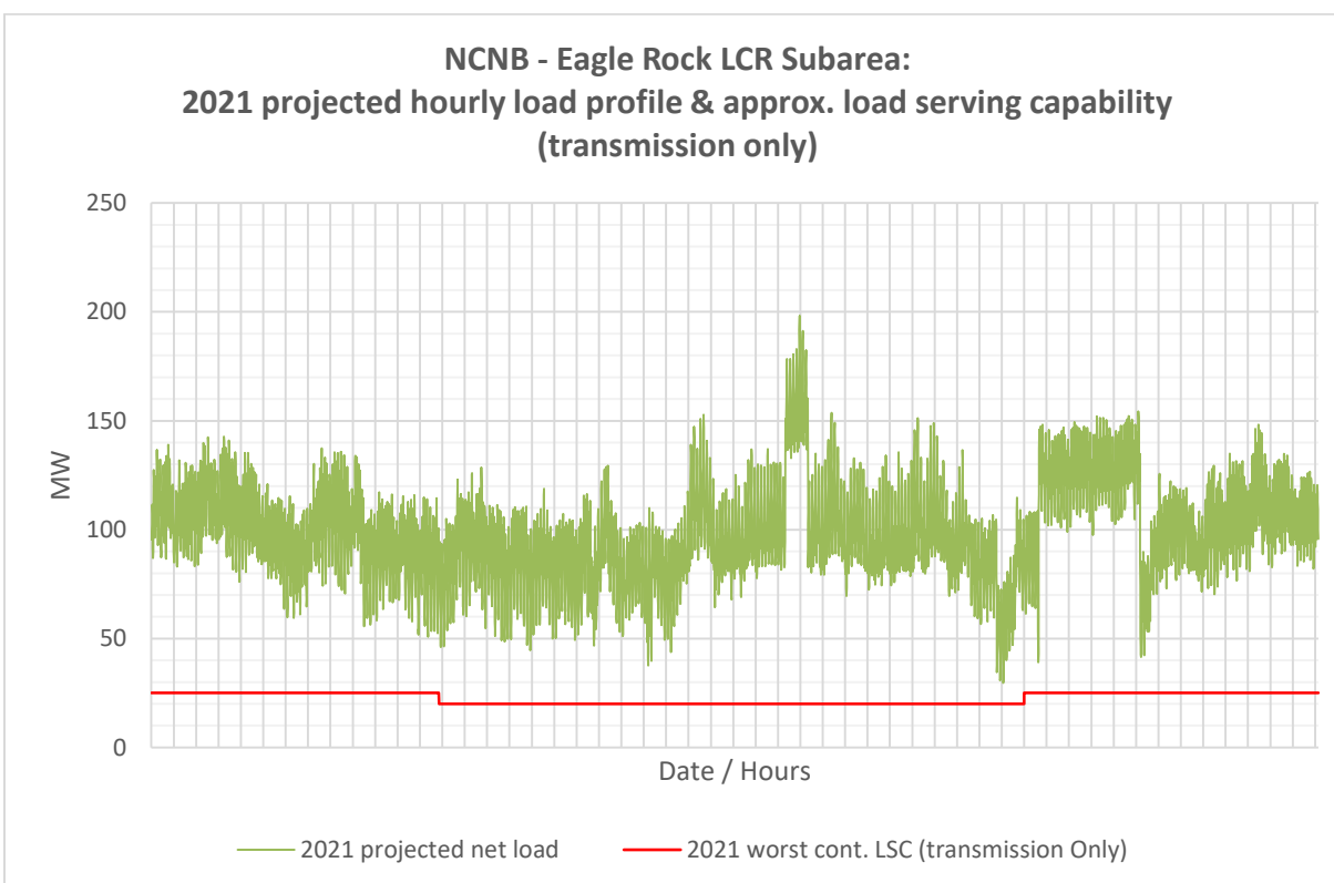
Figure 3.3-9 Eagle Rock LCR Sub-area 2021 Forecast Hourly Profiles
