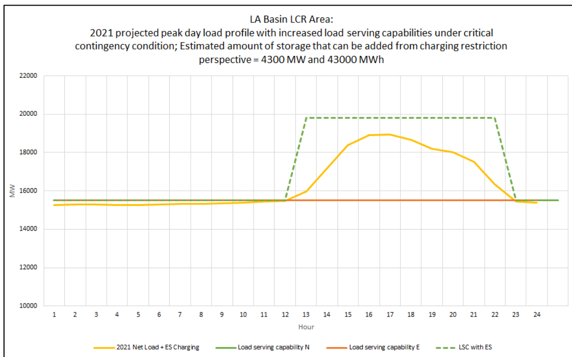
Figure 3.3-95 LA Basin Area 2021 Estimated Amount of Storage that Can Be Added With Higher Load Serving Capability
