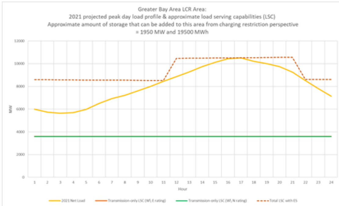
Figure 3.3-46 Bay Area LCR Area 2021 Peak Day Forecast Profiles
