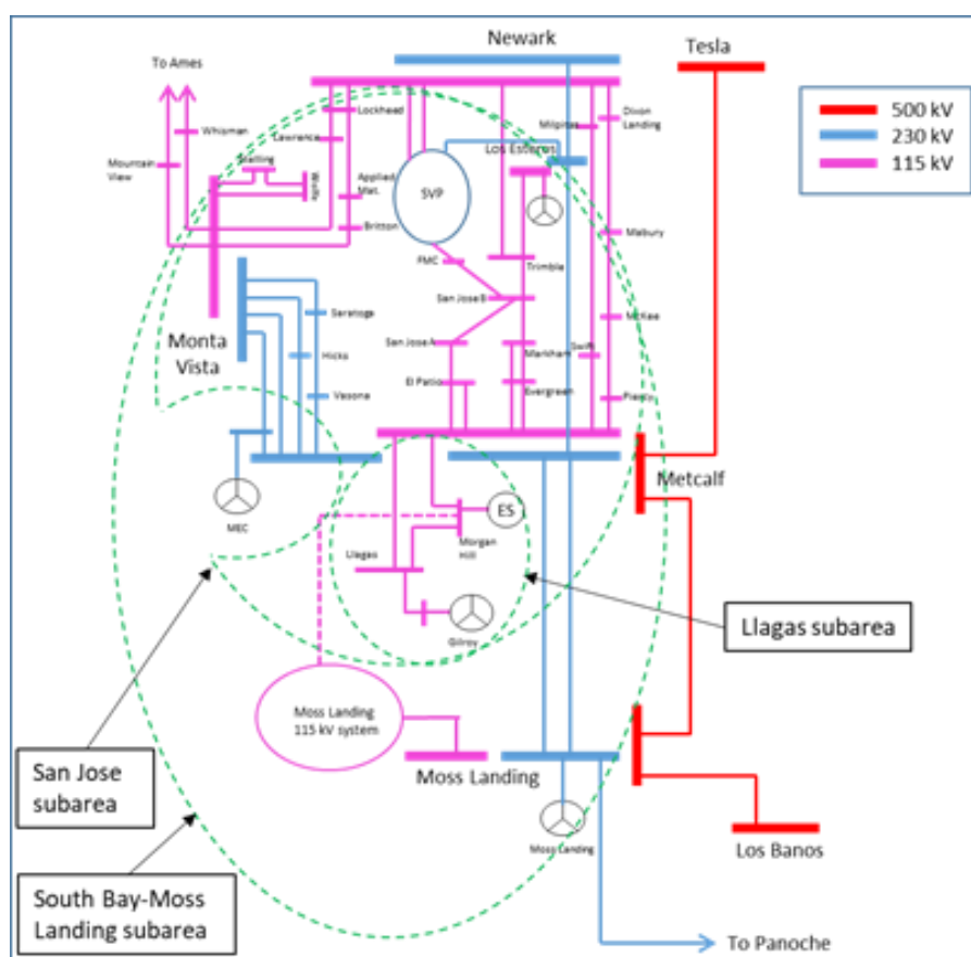
Figure 3.3-34 Llagas LCR Sub-area
