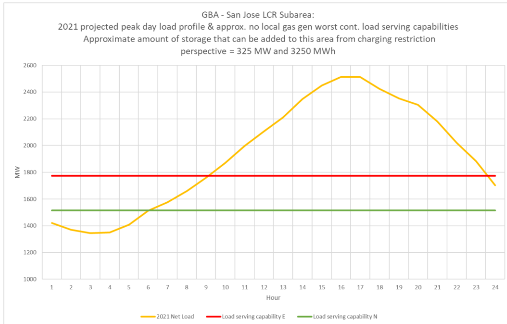
Figure 3.3-37 San Jose LCR Sub-area 2021 Peak Day Forecast Profiles
