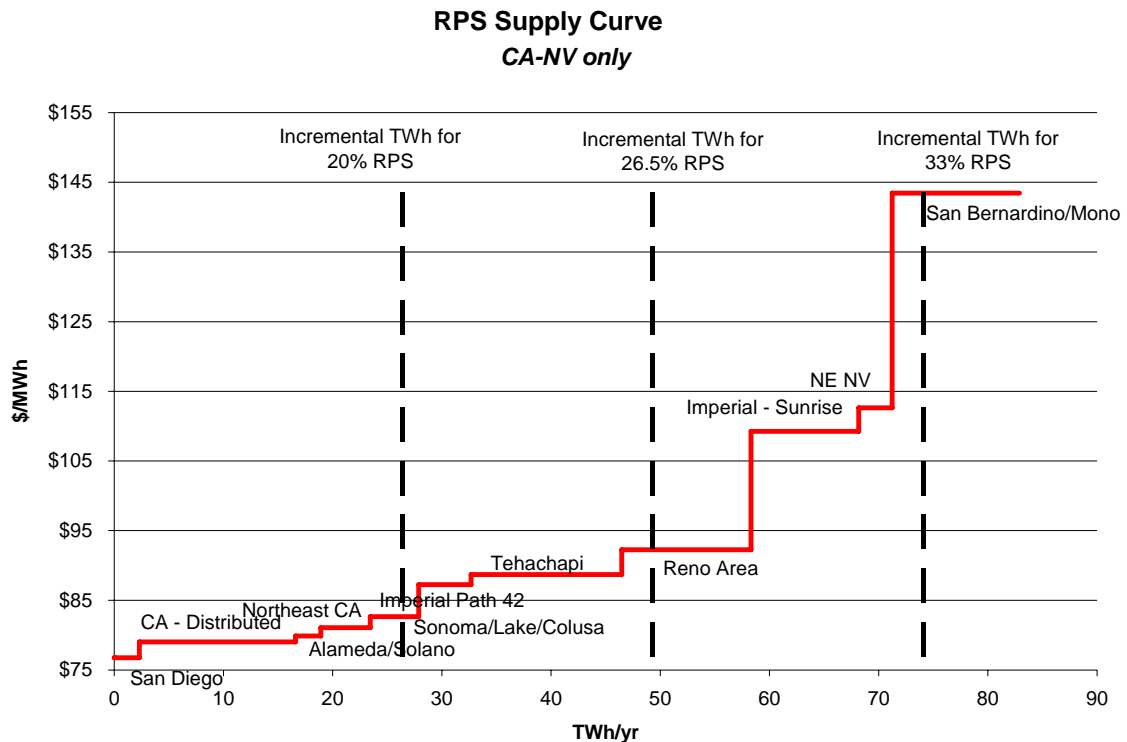
8 9 Figure 4.2. Supply curve of potential resources for meeting California’s RPS using CA 10 and NV resources only
