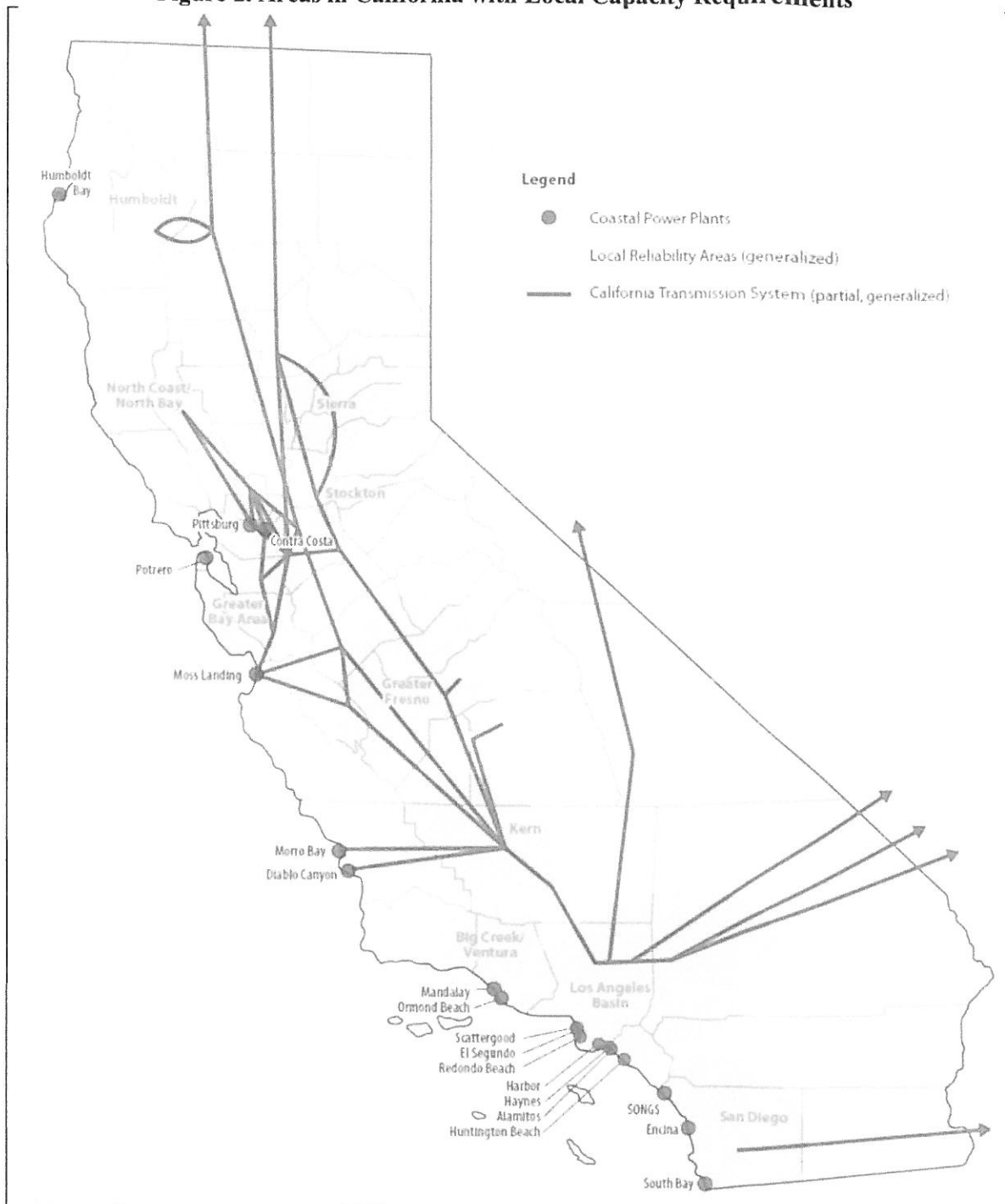
Figure 2. Areas in California with Local Capacity Requirements 11
