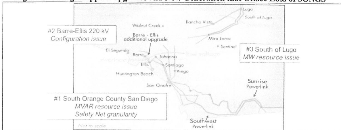
Figure 7. Voltage Support Upgrades and New Generation that Offset Loss of SONGS 44
