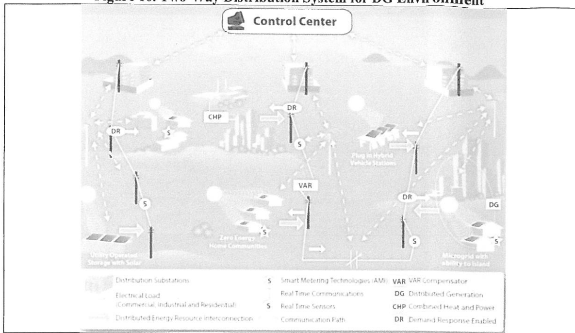
Figure 10. Two-Way Distribution System for DG Environment 57
