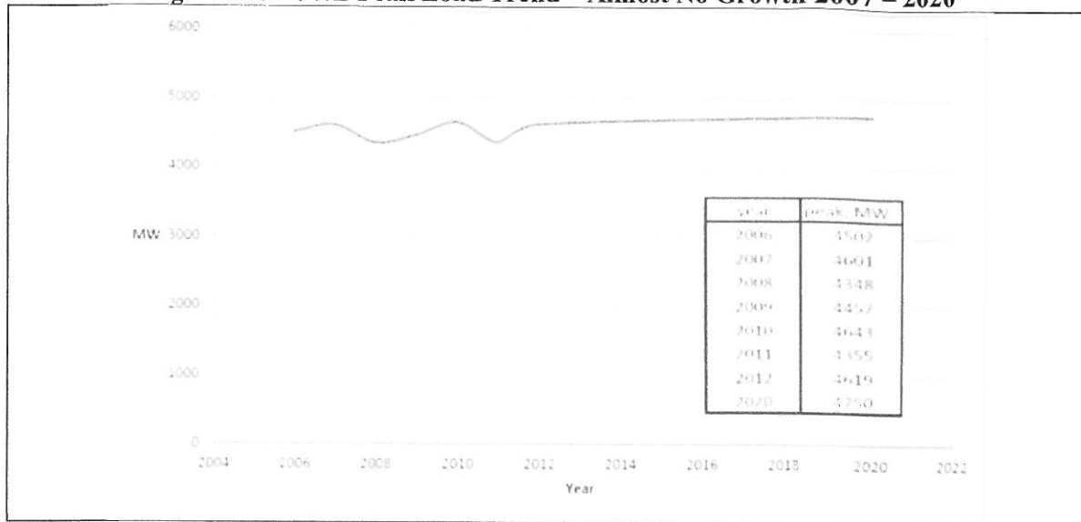
Figure 5. SDG&E Peak Load Trend – Almost No Growth 2007 – 2020
