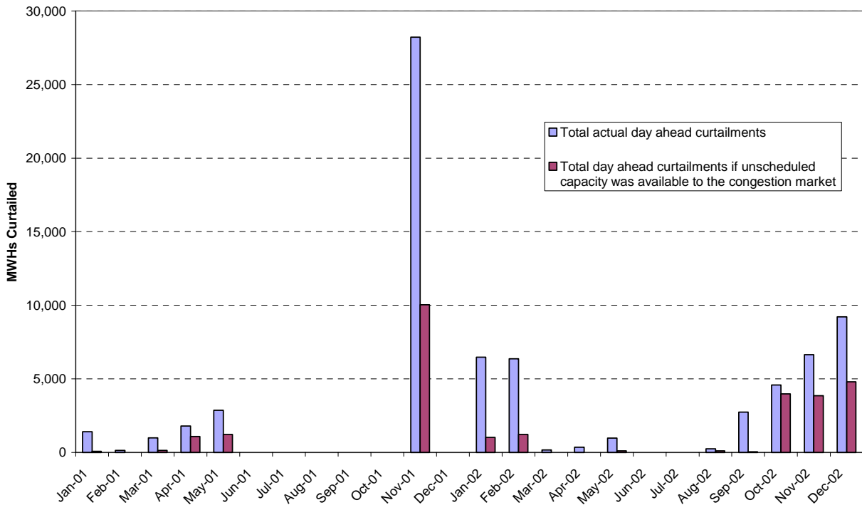
Day Ahead Import Curtailments of Palo Verde January 2001 - December 2002
