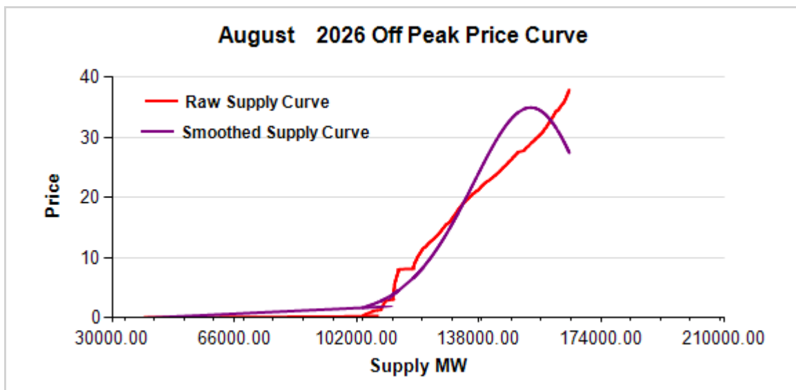
FIGURE 1: August 2026 OFF-PEAK REGRESSION RESULT
