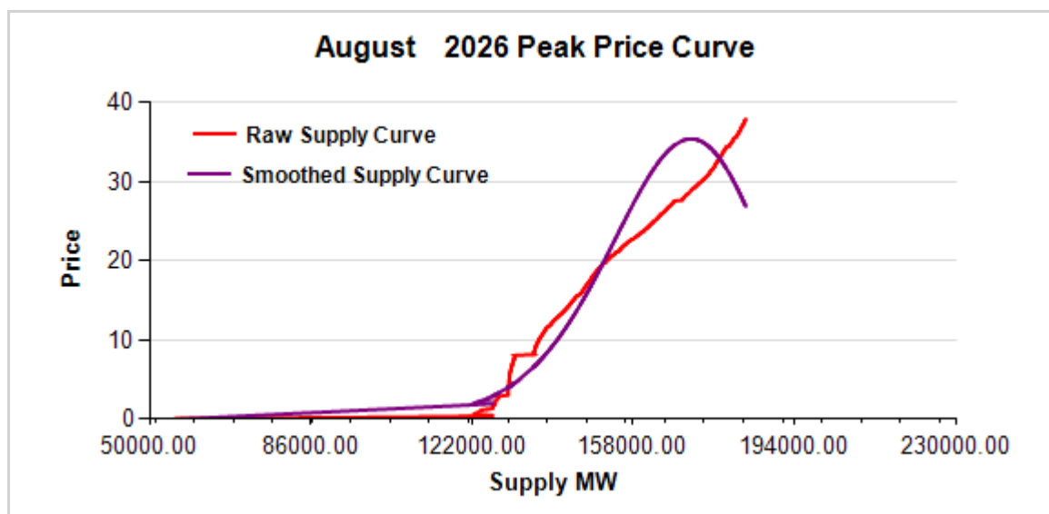
FIGURE 2: August 2026 ON-PEAK REGRESSION RESULT
