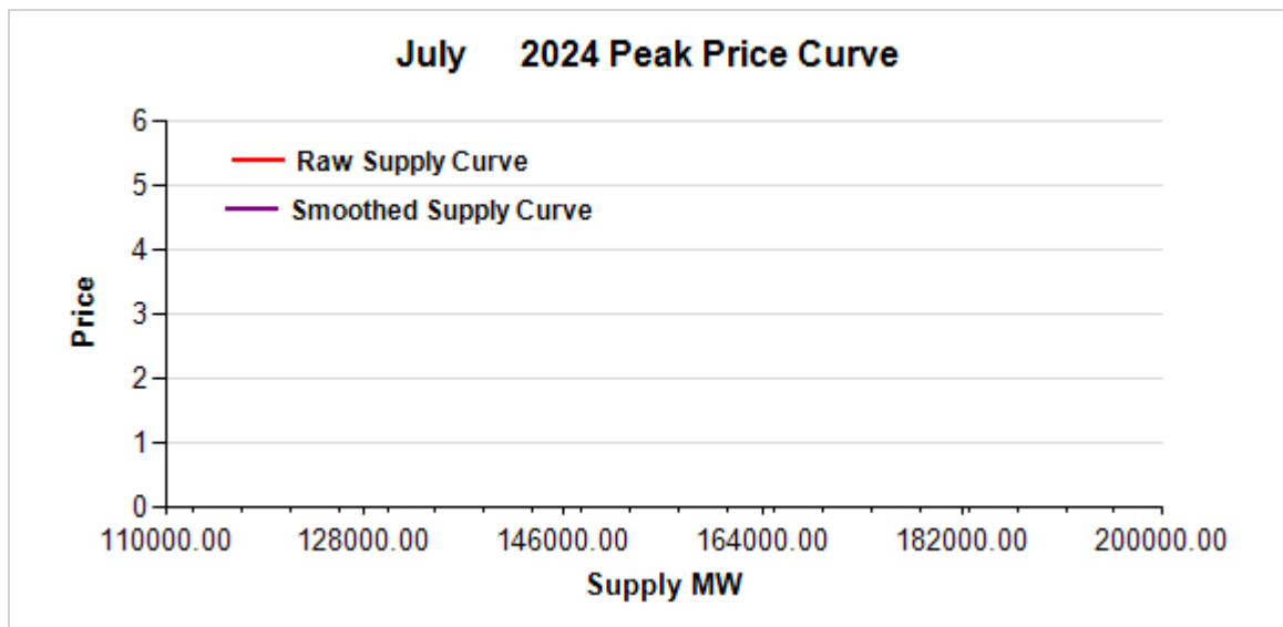
FIGURE 2: July 2024 ON-PEAK REGRESSION RESULT
