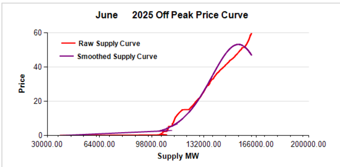
FIGURE 1: June 2025 OFF-PEAK REGRESSION RESULT
