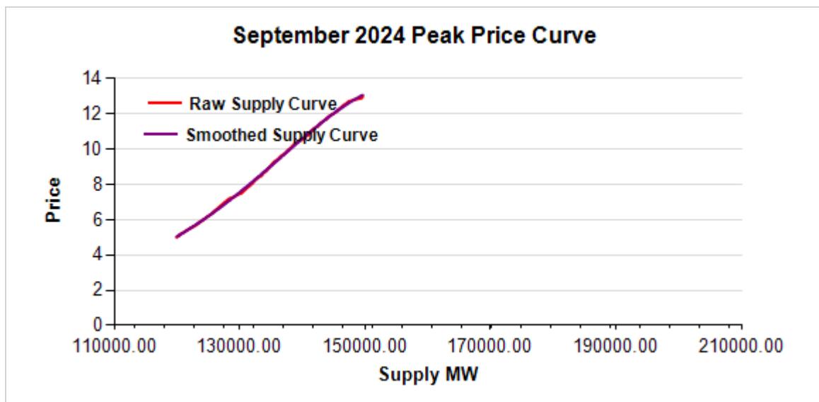
FIGURE 2: September 2024 ON-PEAK REGRESSION RESULT
