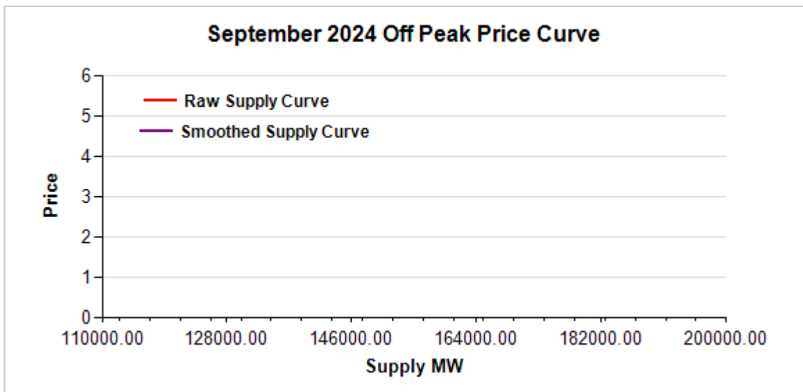
FIGURE 1: September 2024 OFF-PEAK REGRESSION RESULT
