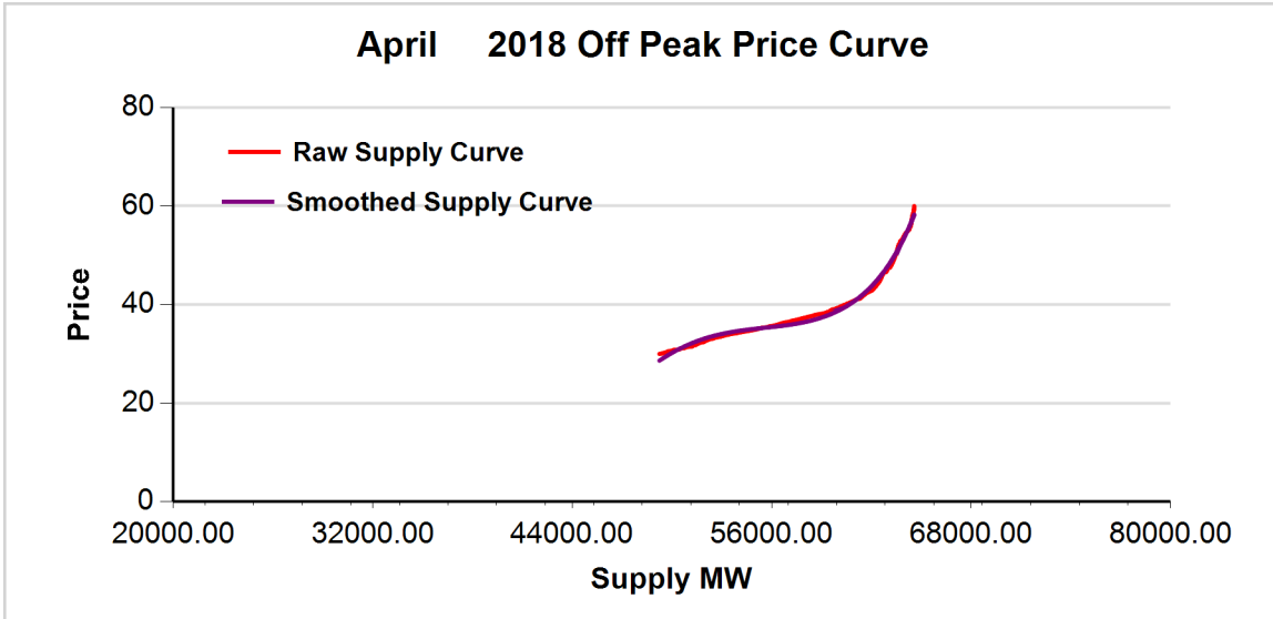
FIGURE 1: April 2018 OFF-PEAK REGRESSION RESULT
