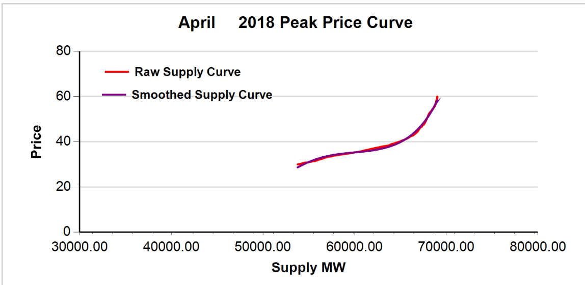
FIGURE 2: April 2018 ON-PEAK REGRESSION RESULT
