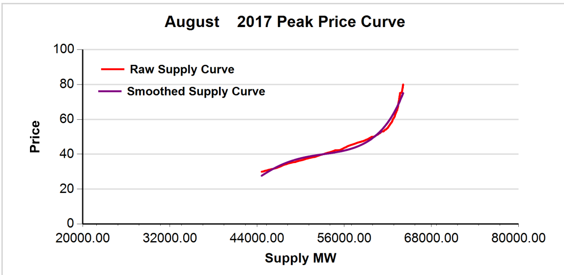
FIGURE 2: August 2017 ON-PEAK REGRESSION RESULT
