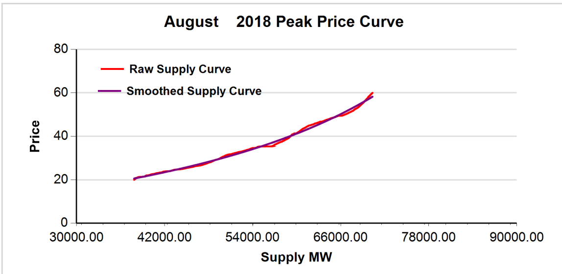
FIGURE 2: August 2018 ON-PEAK REGRESSION RESULT
