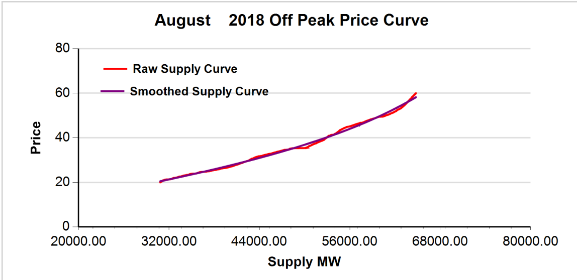
FIGURE 1: August 2018 OFF-PEAK REGRESSION RESULT
