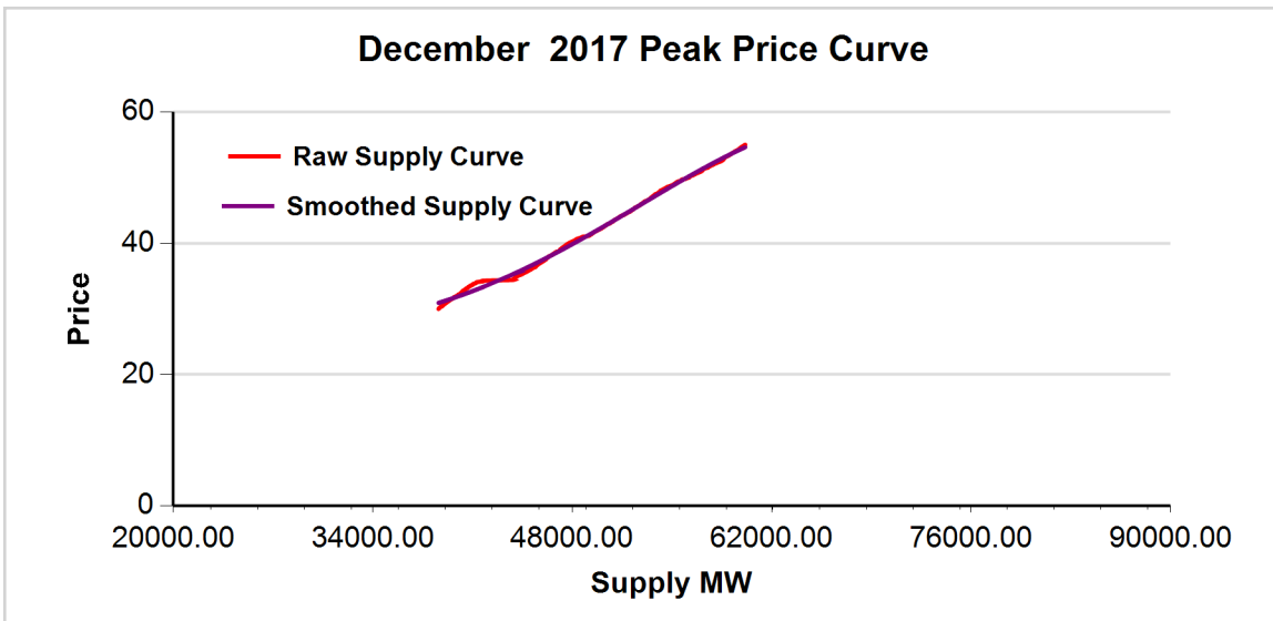
FIGURE 2: December 2017 ON-PEAK REGRESSION RESULT
