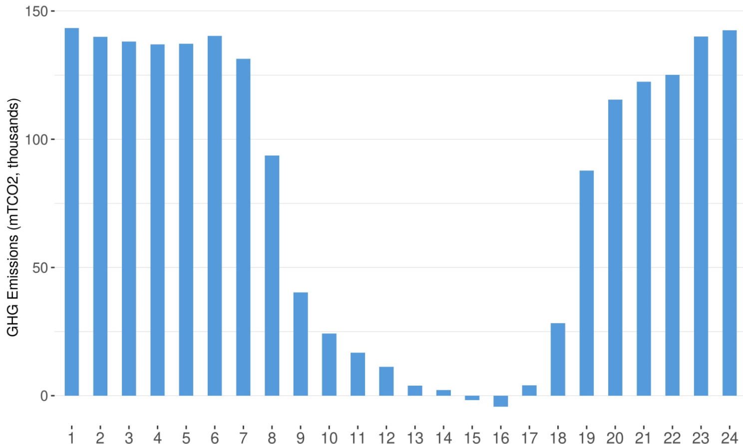
Figure 3 Hourly GHG emissions to serve ISO load for the month of April 2024
