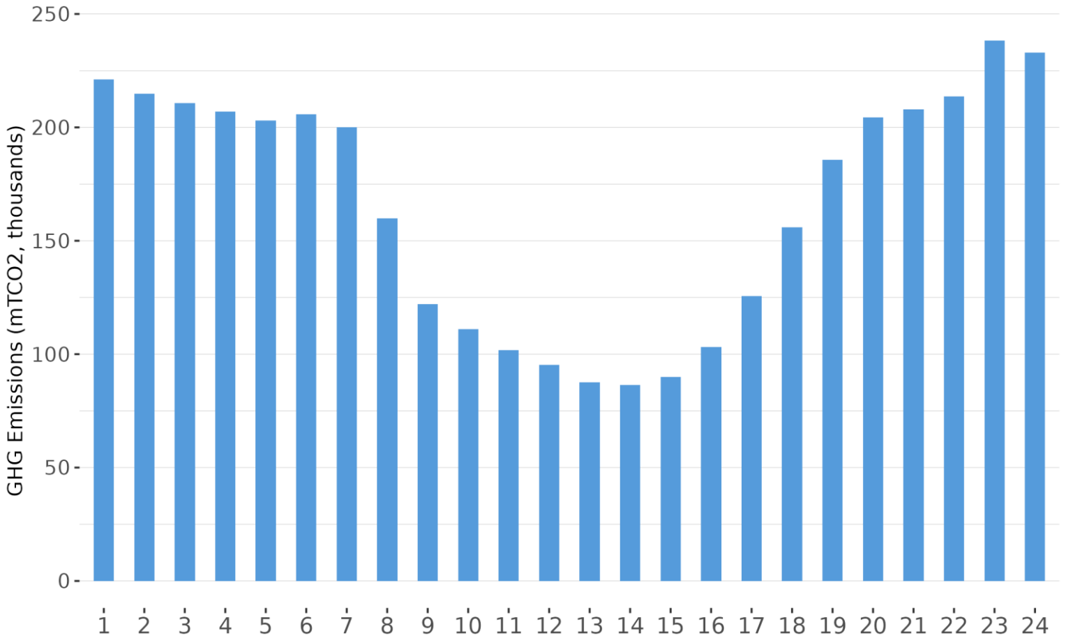
Figure 3 Hourly GHG emissions to serve ISO load for the month of August 2025
