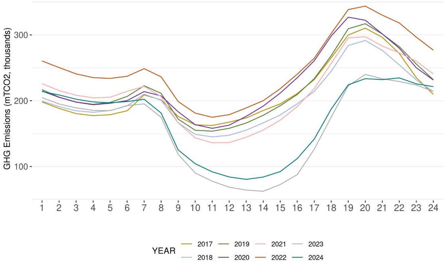
Figure 4 Comparison of hourly GHG emissions to serve ISO for the month of September
