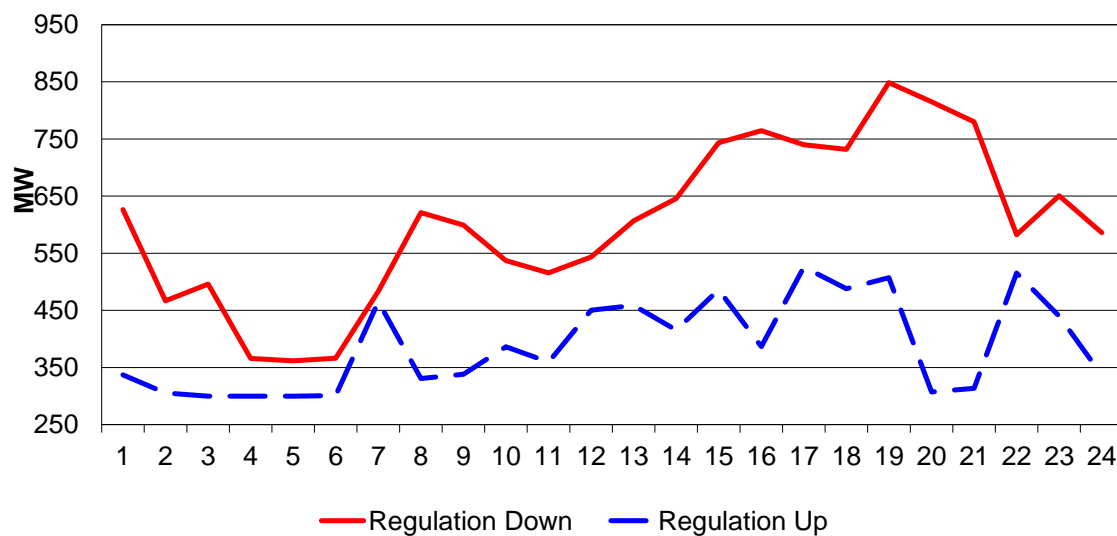
Figure 63: IFM (Day-Ahead) Hourly Average Regulation Requirement
