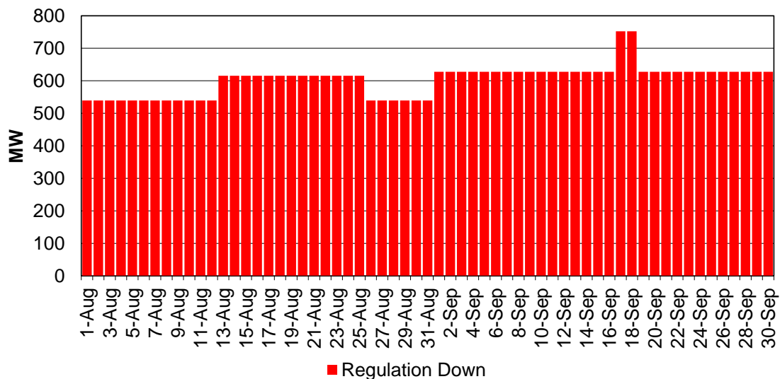
Figure 65: IFM (Day-Ahead) Regulation Down Procurement
