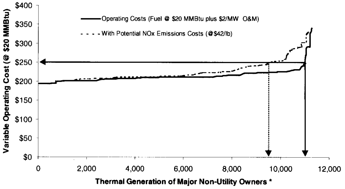
Figure 3. Potential Variable Operating Costs of Major Non-Utility Owned Thermal Generation within ISO Control Area Typical Conditions - December, 2000
