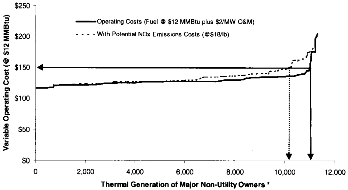
Figure 4. Potential Variable Operating Costs of Major Non-Utility Owned Thermal Generation within ISO Control Area Typical Conditions - January, 2001
