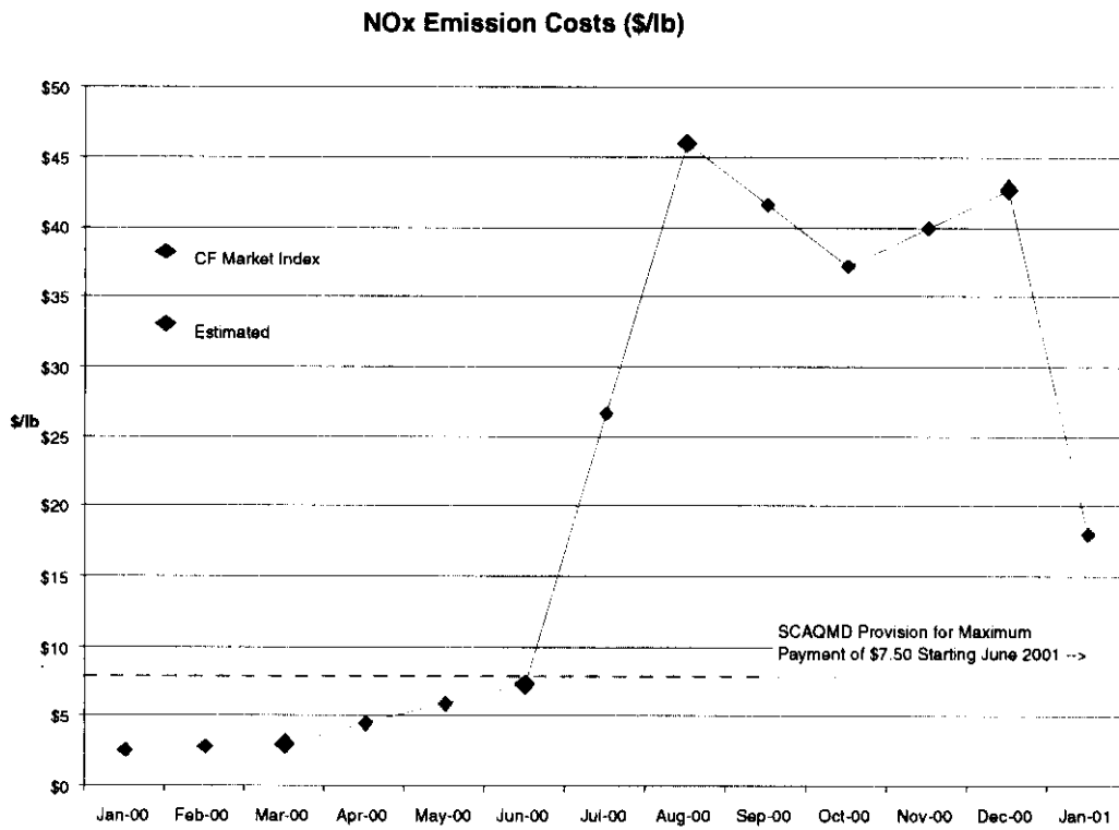
Figure 2. Potential NOx Emission Credit Costs
