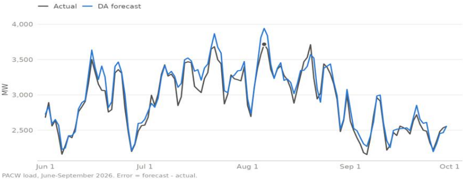
PACW: daily peak load, actual vs DA forecast, summer 2026 Highest hourly value each day. Summer peak (marked): 3,717 MW on Aug 6, HE 18
