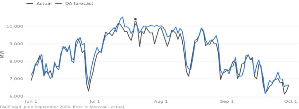
PACE: daily peak load, actual vs DA forecast, summer 2026 Highest hourly value each day. Summer peak (marked): 10,410 MW on Jul 20, HE 17
