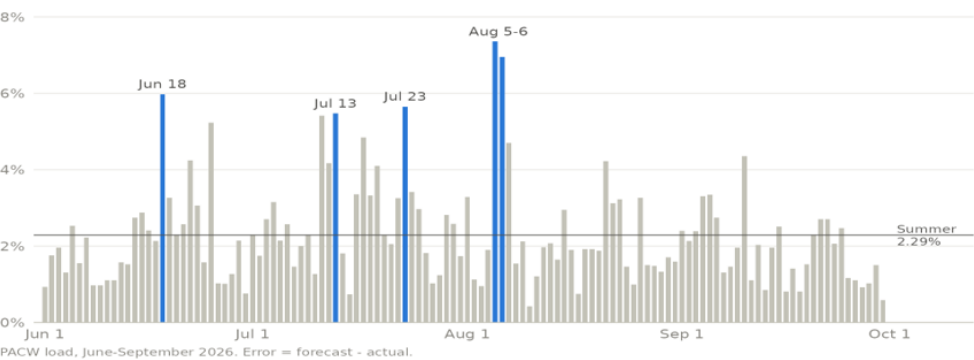
PACW: daily DA load forecast MAPE, summer 2026 The 5 highest-error days are highlighted and labeled
