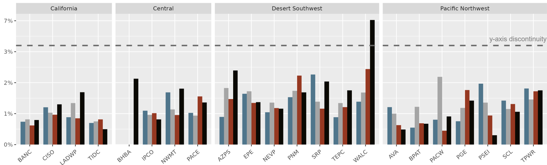
T-60 Accuracy During Peak Hour Average for 10 highest load days
