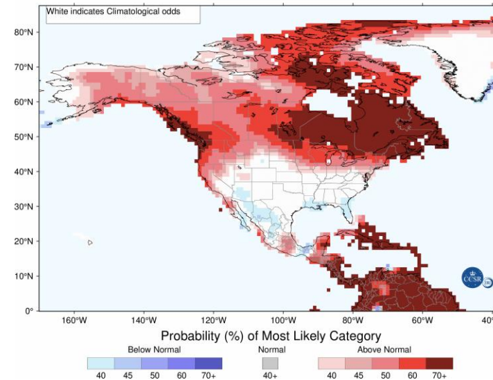
CCSR/IRI Multi-Model Probability Forecast for Temperature for December-January-February 2027, Issued October 2026
