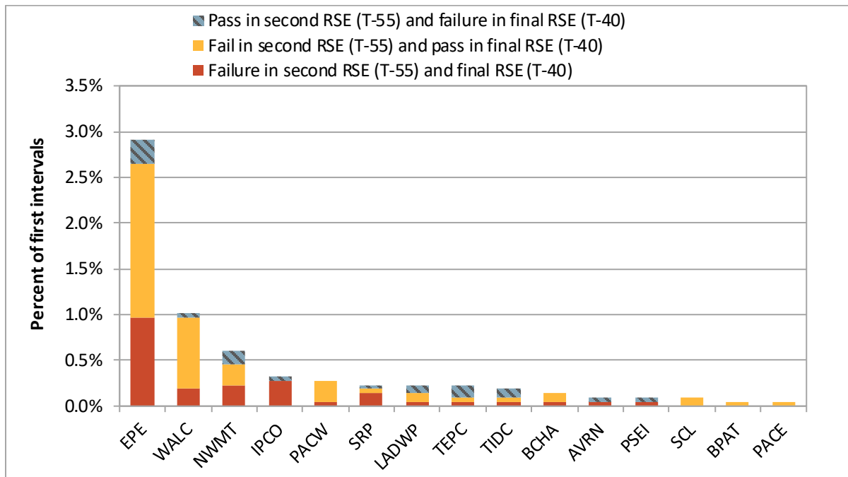
Figure 3.2 Downward resource sufficiency evaluation failures in first 15-minute interval of hour (January–March 2026)
