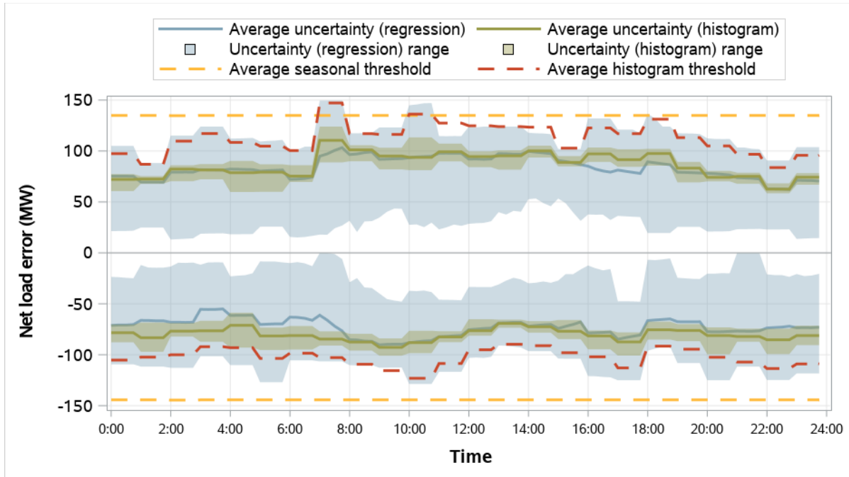
Figure 5.14 NorthWestern Energy resource sufficiency evaluation uncertainty requirements (January–March 2026)
