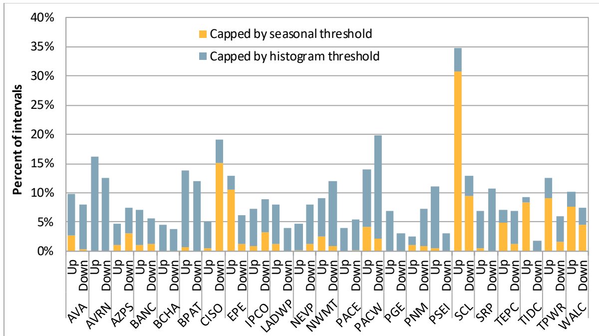
Figure 5.1 Quantile regression uncertainty capped by mosaic or histogram thresholds (January–March 2026)
