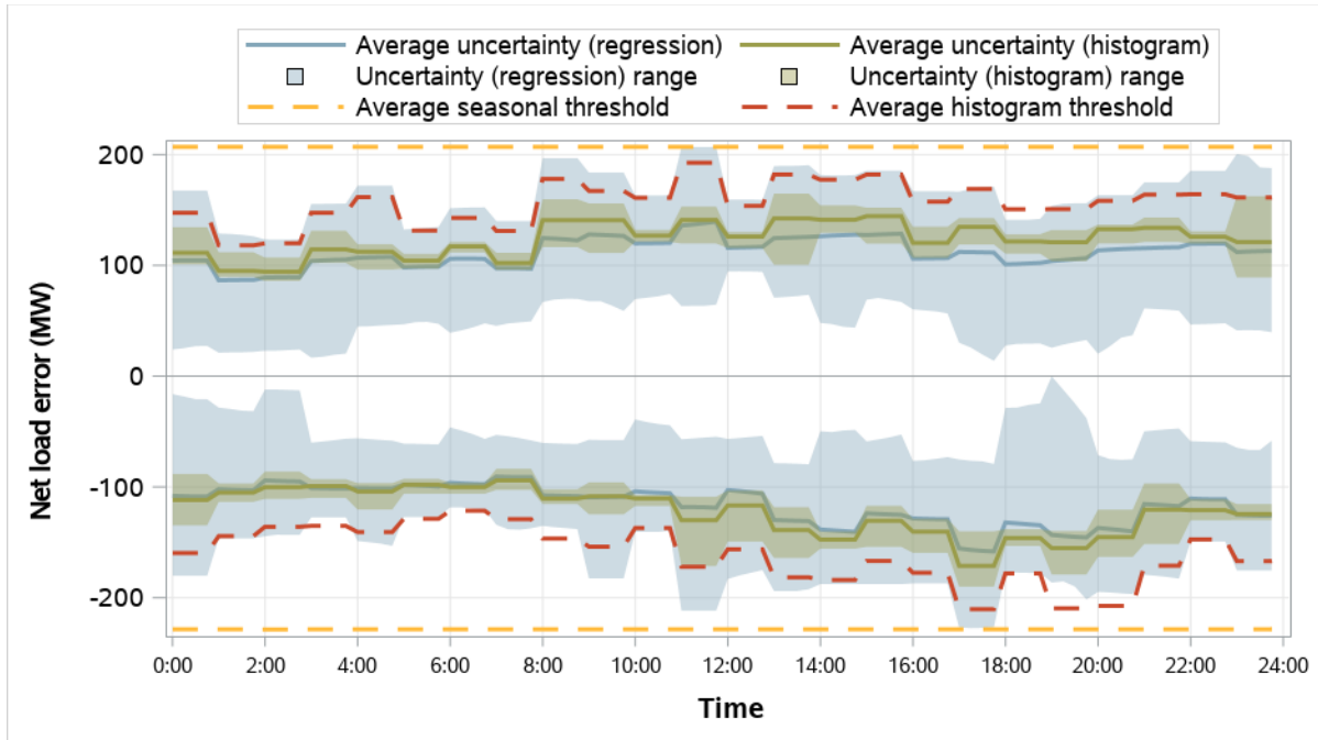
Figure 5.18 Portland General Electric resource sufficiency evaluation uncertainty requirements (January–March 2026)
