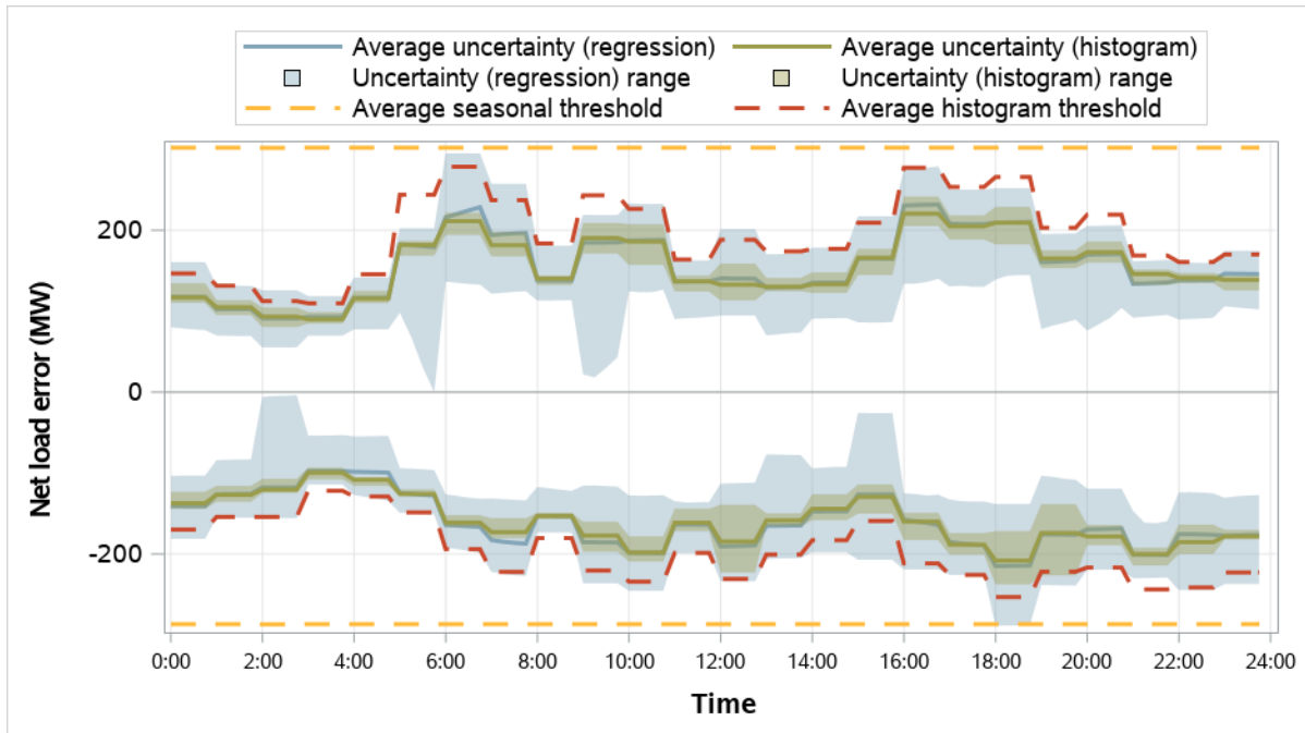
Figure 5.19 Powerex resource sufficiency evaluation uncertainty requirements (January–March 2026)
