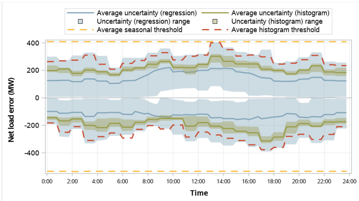
Figure 5.6 Avangrid resource sufficiency evaluation uncertainty requirements (January–March 2026)
