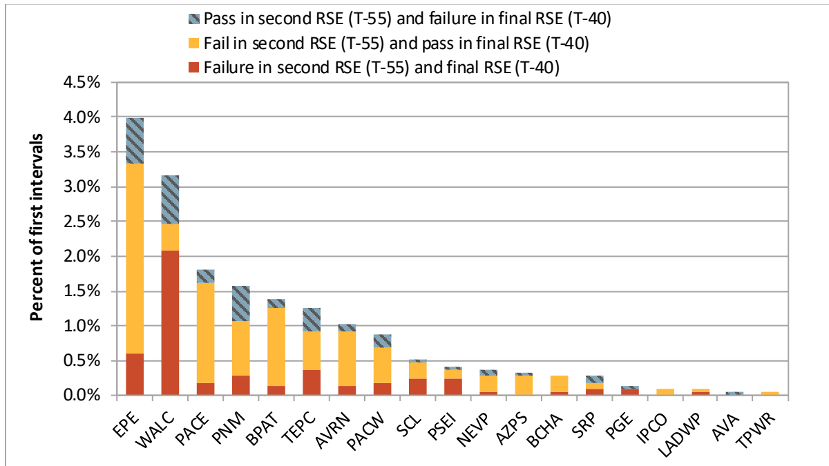
Figure 3.1 Upward resource sufficiency evaluation failures in first 15-minute interval of hour (January–March 2026)
