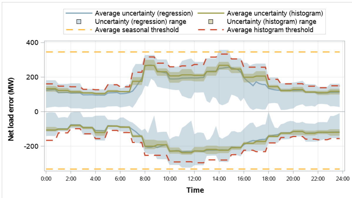
Figure 5.13 LADWP resource sufficiency evaluation uncertainty requirements (January–March 2026)
