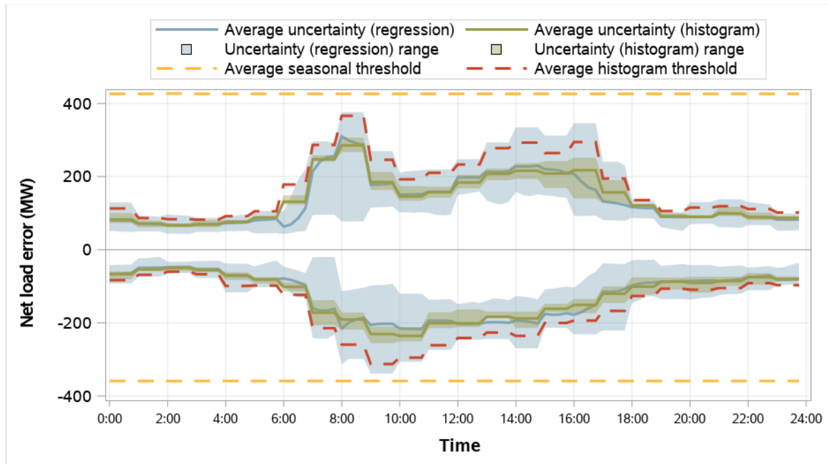
Figure 5.22 Salt River Project resource sufficiency evaluation uncertainty requirements (January–March 2026)
