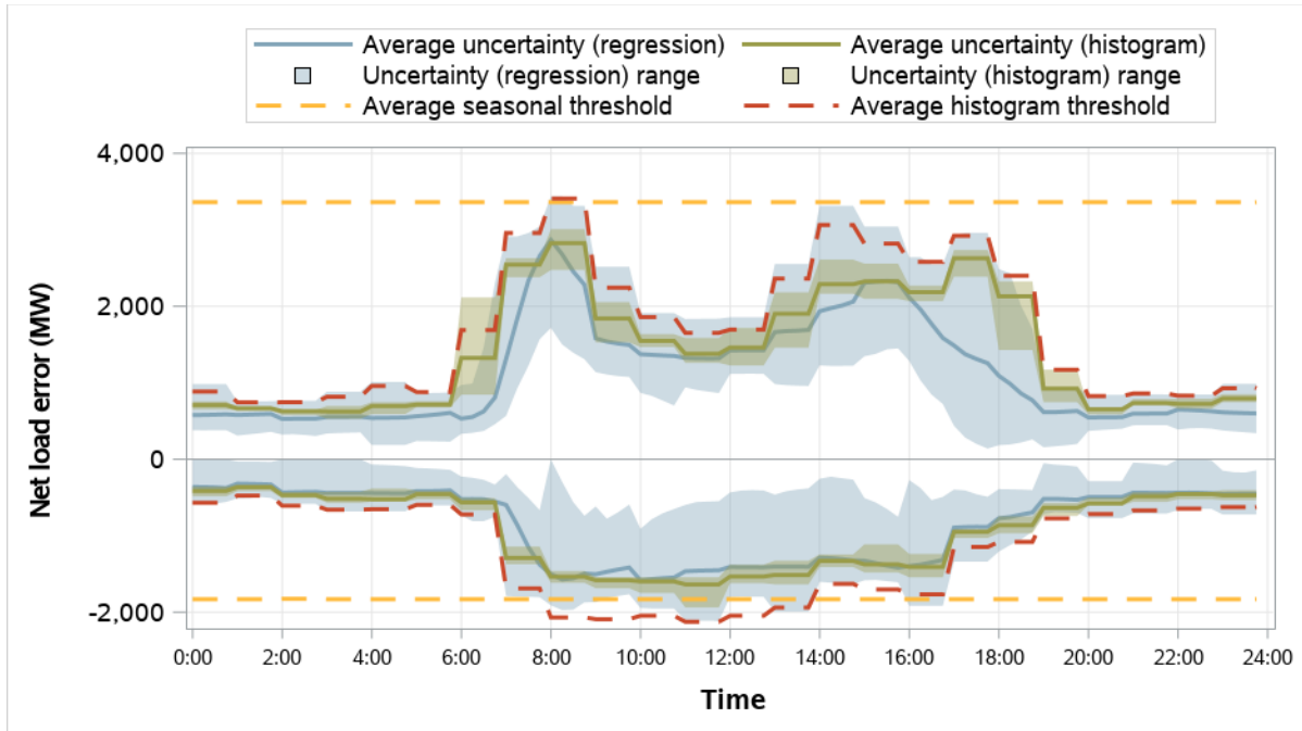
Figure 5.10 California ISO resource sufficiency evaluation uncertainty requirements (January–March 2026)
