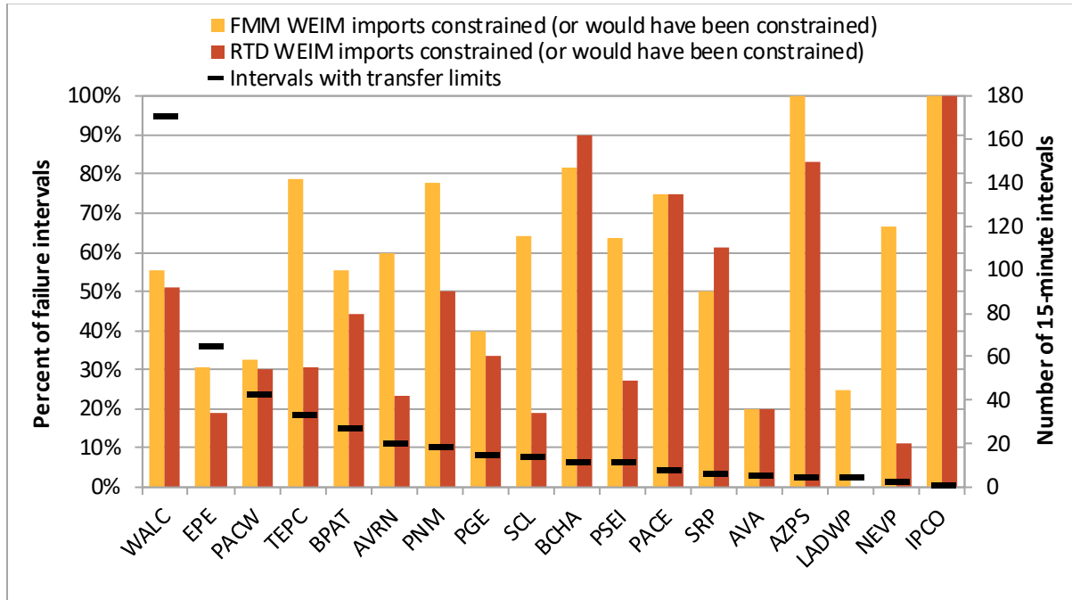
Figure 7.3 Percent of upward failure intervals in which WEIM imports were constrained or would have been constrained by test failure limits (January–March 2026)
