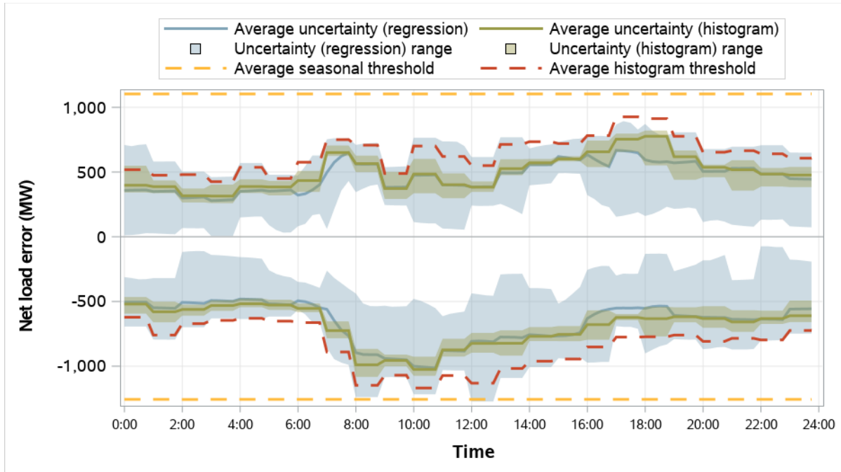
Figure 5.16 PacifiCorp East resource sufficiency evaluation uncertainty requirements (January–March 2026)
