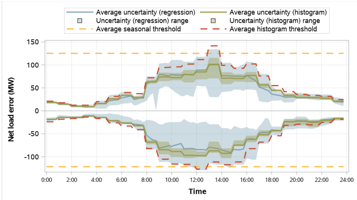
Figure 5.8 BANC resource sufficiency evaluation uncertainty requirements (January–March 2026)
