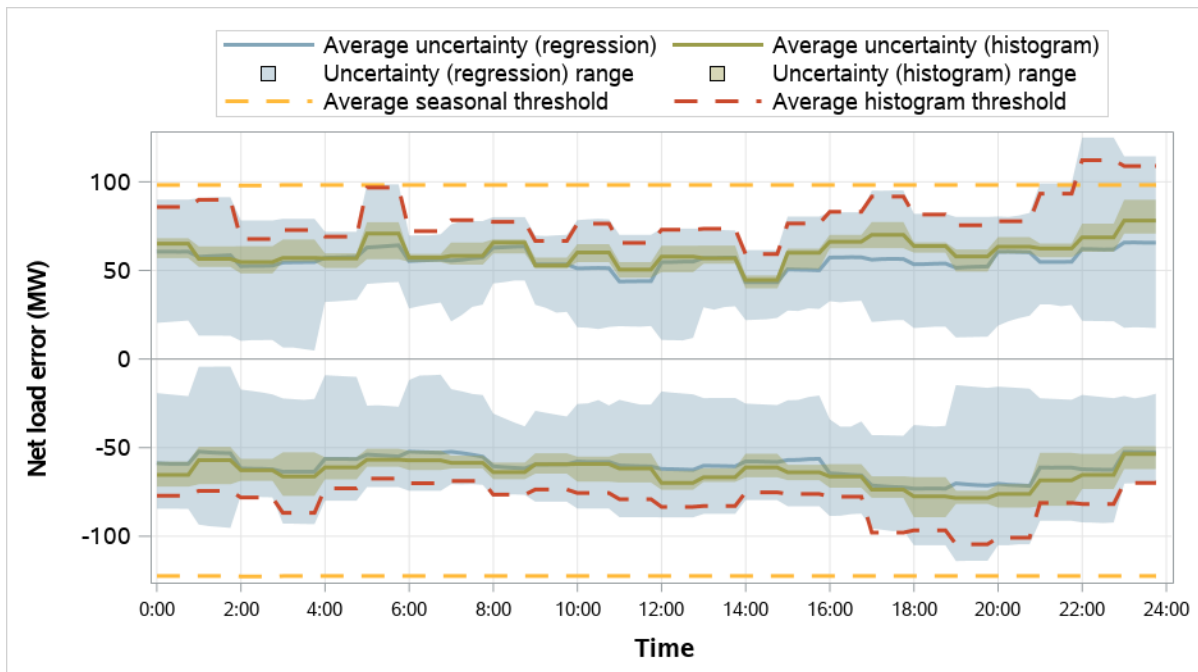
Figure 5.7 Avista resource sufficiency evaluation uncertainty requirements (January–March 2026)
