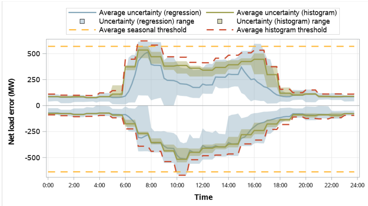
Figure 5.20 PNM resource sufficiency evaluation uncertainty requirements (January–March 2026)
