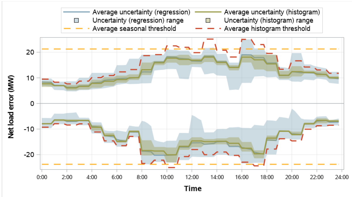
Figure 5.24 Tacoma Power resource sufficiency evaluation uncertainty requirements (January–March 2026)
