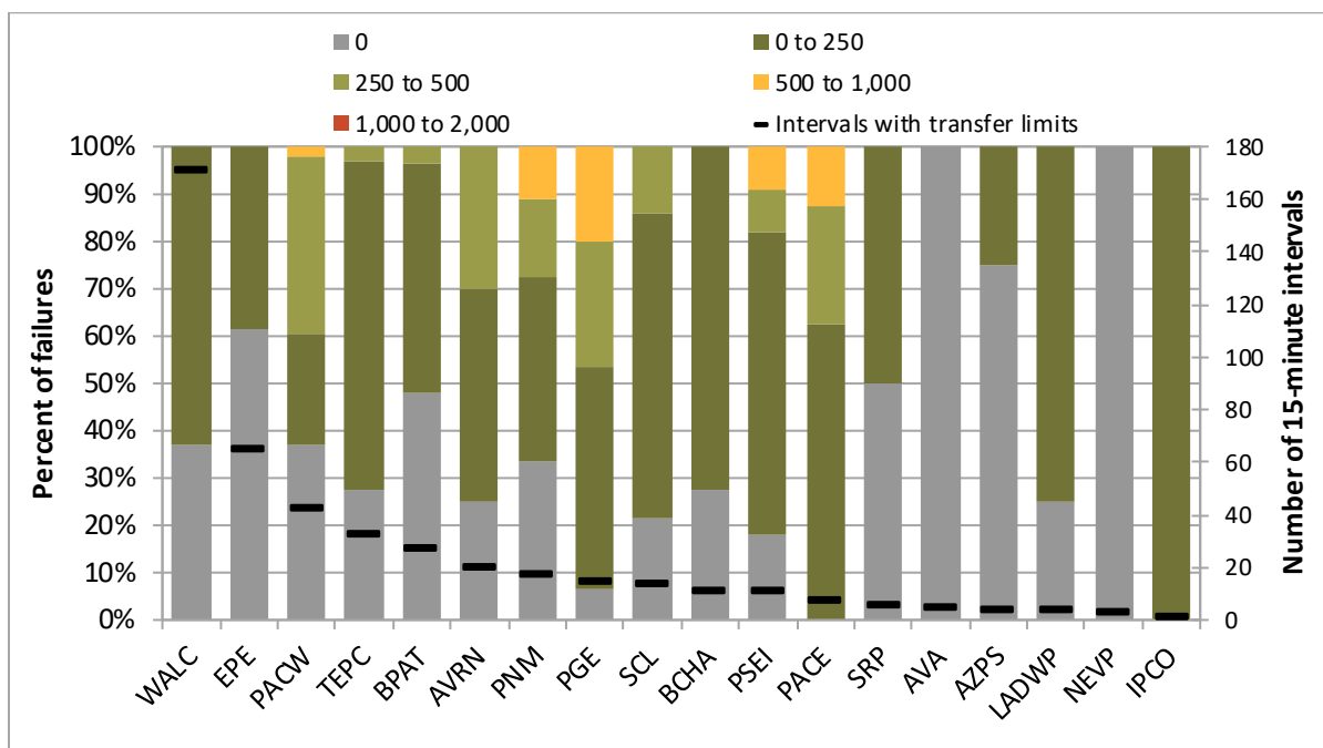
Figure 7.2 Upward capacity/flexibility test failure intervals by dynamic import limit (January–March 2026)
