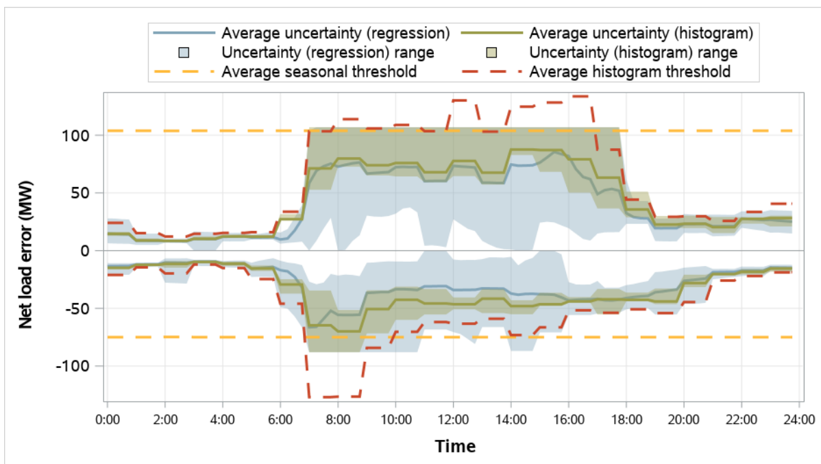
Figure 5.27 WAPA Desert Southwest resource sufficiency evaluation uncertainty requirements (January–March 2026)
