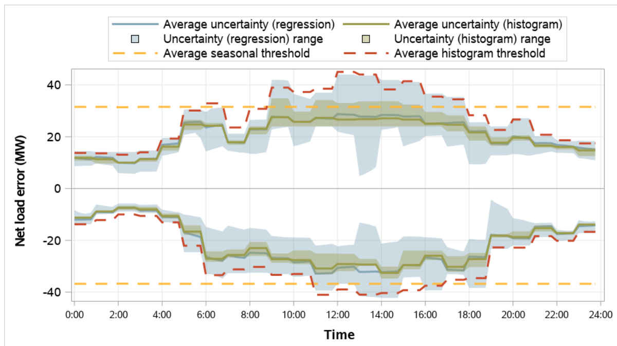
Figure 5.23 Seattle City Light resource sufficiency evaluation uncertainty requirements (January–March 2026)
