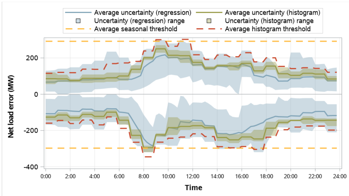
Figure 5.12 Idaho Power resource sufficiency evaluation uncertainty requirements (January–March 2026)
