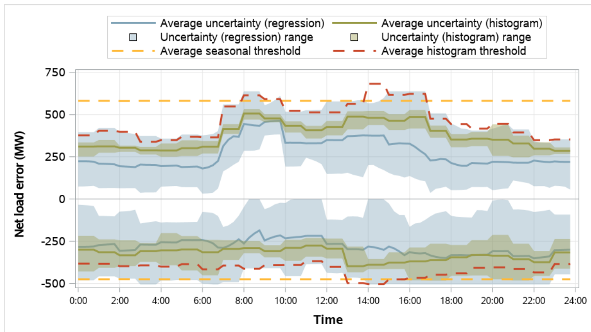
Figure 5.5 Arizona Public Service resource sufficiency evaluation uncertainty requirements (January–March 2026)
