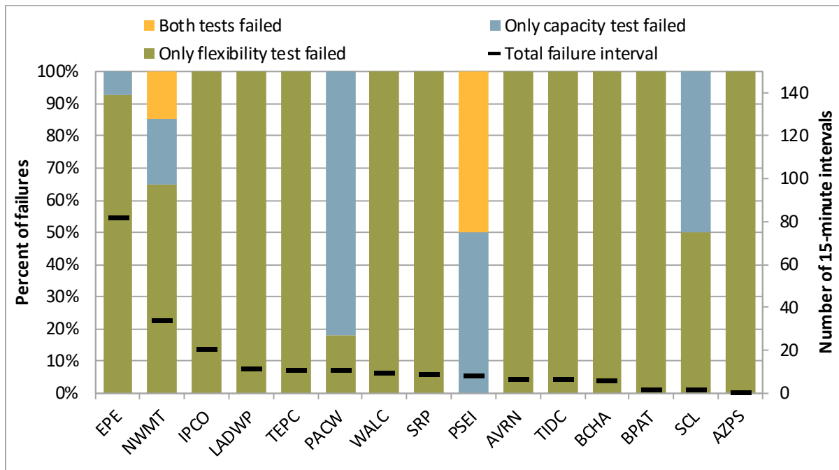
Figure 2.12 Downward capacity/flexibility test failure intervals by concurrence (January–March 2026)
