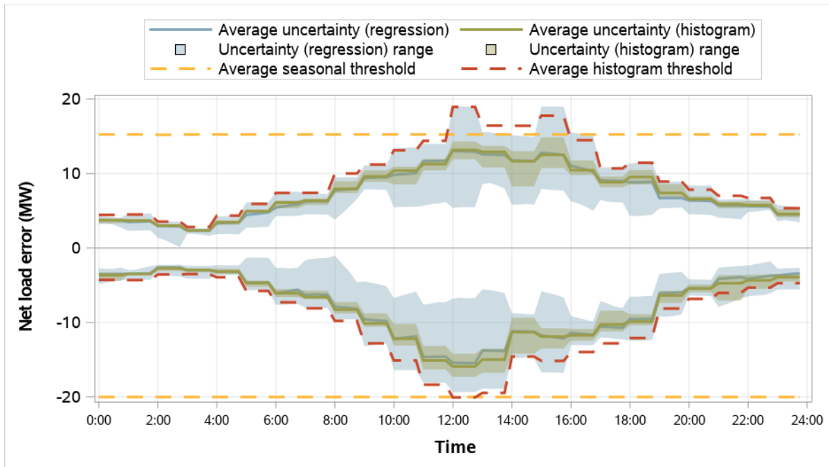
Figure 5.26 Turlock Irrigation District resource sufficiency evaluation uncertainty requirements (January–March 2026)
