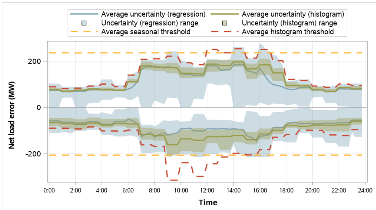
Figure 5.25 Tucson Electric Power resource sufficiency evaluation uncertainty requirements (January–March 2026)
