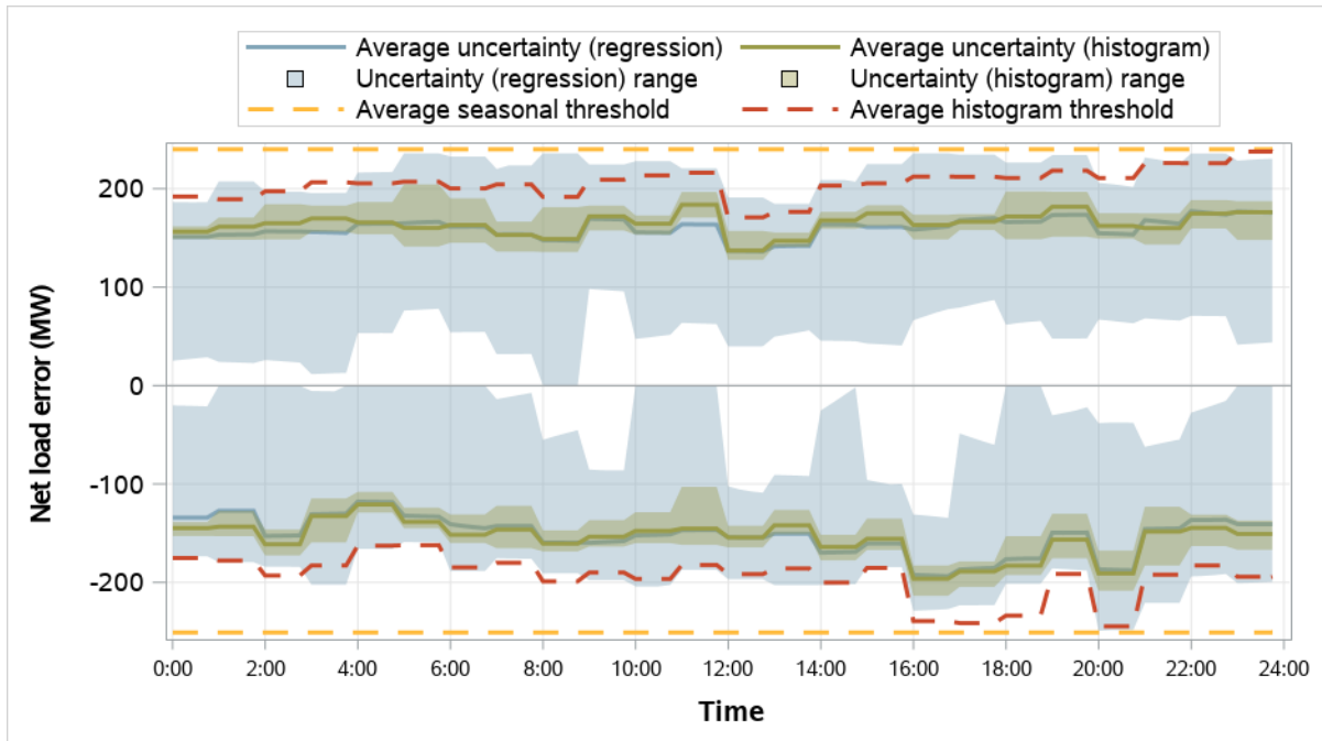
Figure 5.21 Puget Sound Energy resource sufficiency evaluation uncertainty requirements (January–March 2026)
