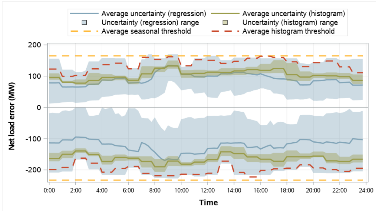
Figure 5.17 PacifiCorp West resource sufficiency evaluation uncertainty requirements (January–March 2026)
