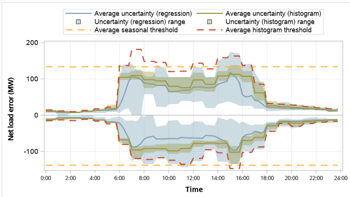
Figure 5.11 El Paso Electric resource sufficiency evaluation uncertainty requirements (January–March 2026)
