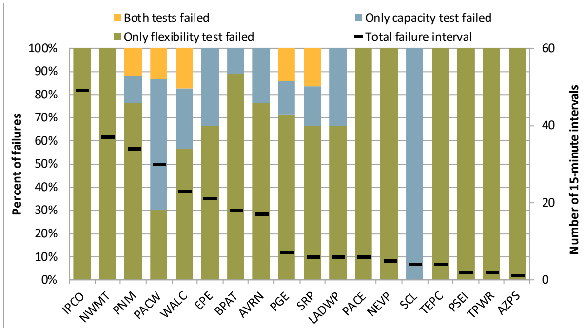
Figure 2.11 Upward capacity/flexibility test failure intervals by concurrence (January–March 2026)
