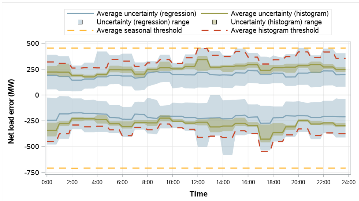
Figure 5.9 BPA resource sufficiency evaluation uncertainty requirements (January–March 2026)
