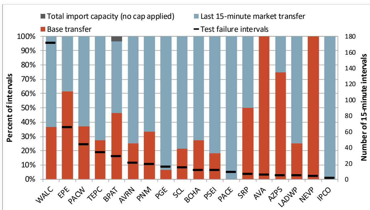
Figure 7.1 Upward capacity/flexibility test failure intervals by source of import limit (January–March 2026)
