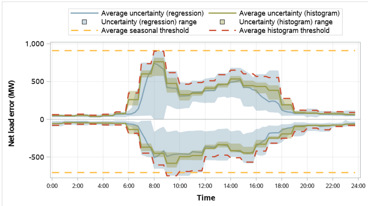
Figure 5.15 NV Energy resource sufficiency evaluation uncertainty requirements (January–March 2026)
