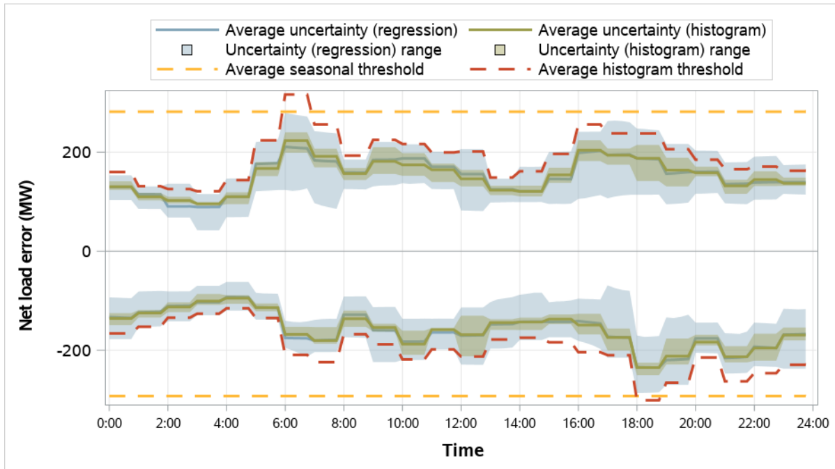
Figure 5.19 Powerex resource sufficiency evaluation uncertainty requirements (October–December 2025)
