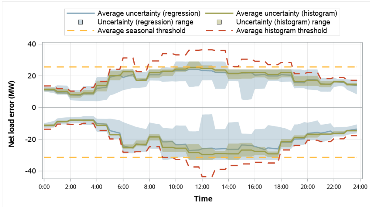
Figure 5.23 Seattle City Light resource sufficiency evaluation uncertainty requirements (October–December 2025)
