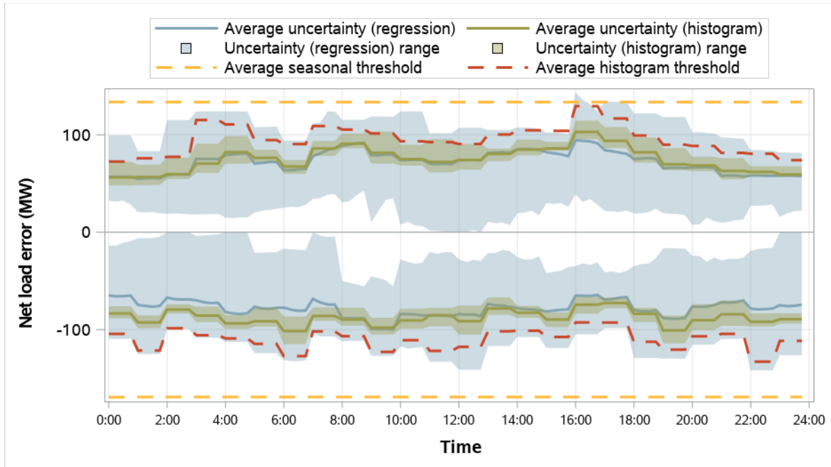
Figure 5.14 NorthWestern Energy resource sufficiency evaluation uncertainty requirements (October–December 2025)
