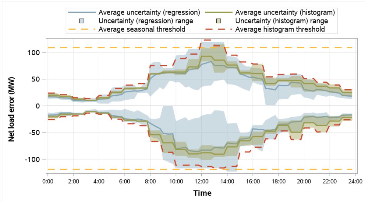
Figure 5.8 BANC resource sufficiency evaluation uncertainty requirements (October–December 2025)
