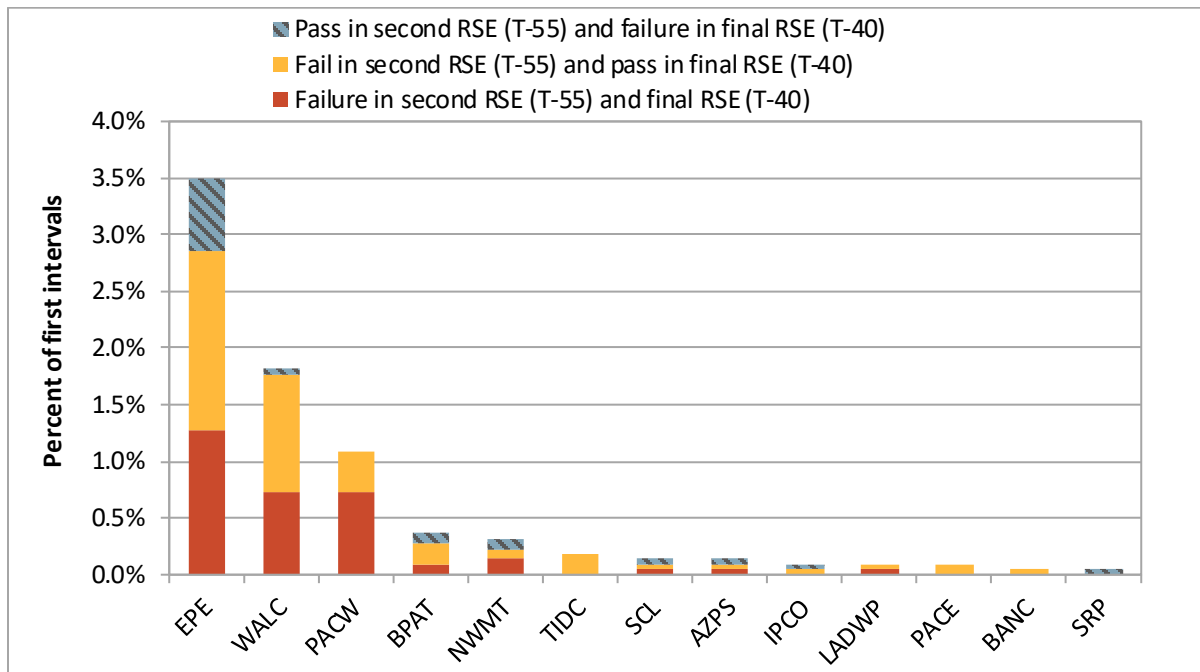
Figure 3.2 Downward resource sufficiency evaluation failures in first 15-minute interval of hour (October–December 2025)
