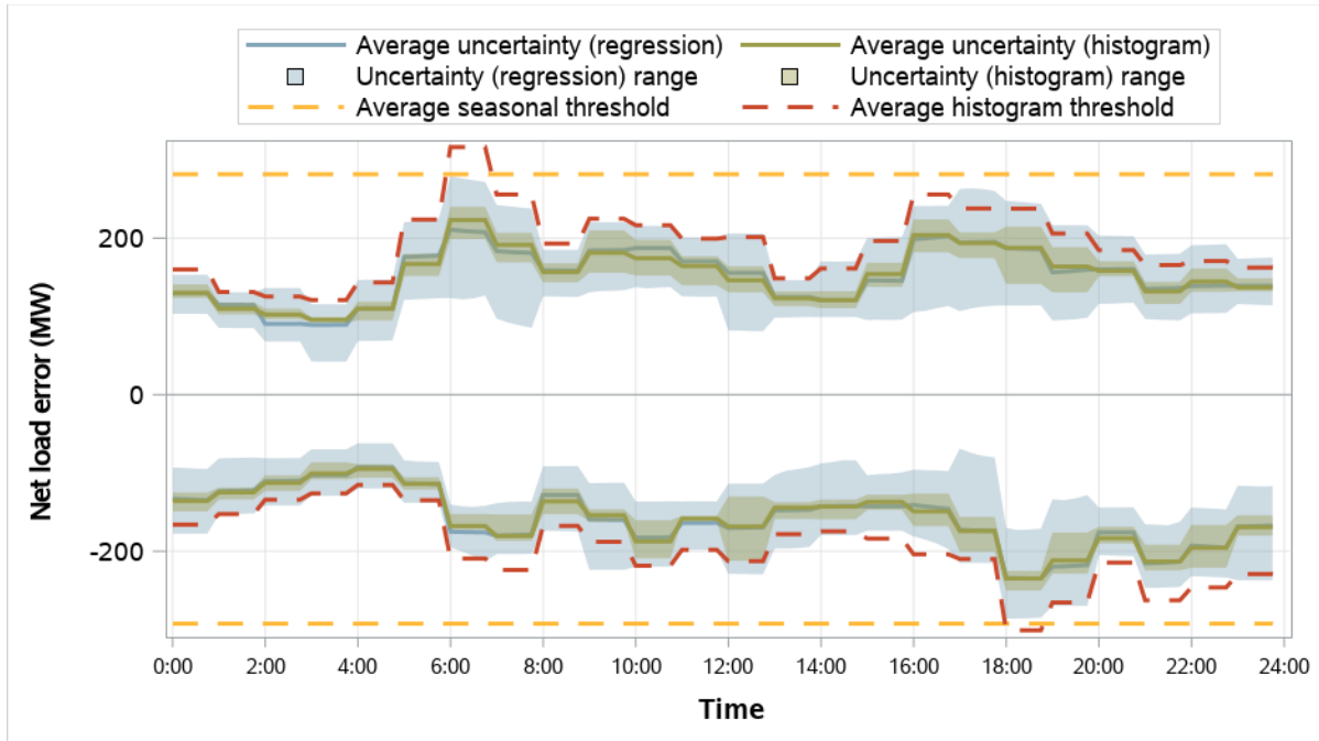
Figure 5.20 PNM resource sufficiency evaluation uncertainty requirements (October–December 2025)
