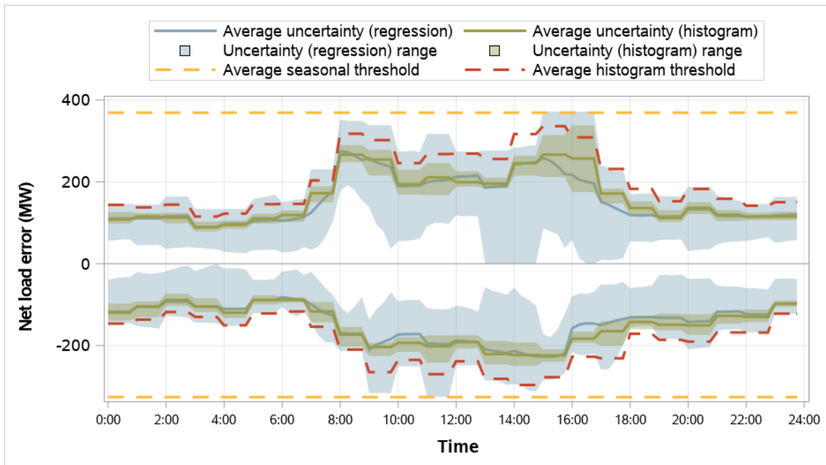
Figure 5.13 LADWP resource sufficiency evaluation uncertainty requirements (October–December 2025)
