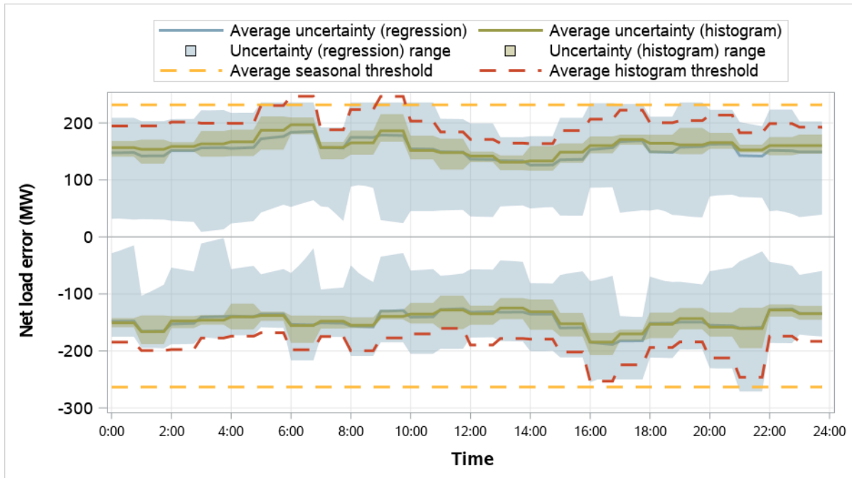
Figure 5.21 Puget Sound Energy resource sufficiency evaluation uncertainty requirements (October–December 2025)
