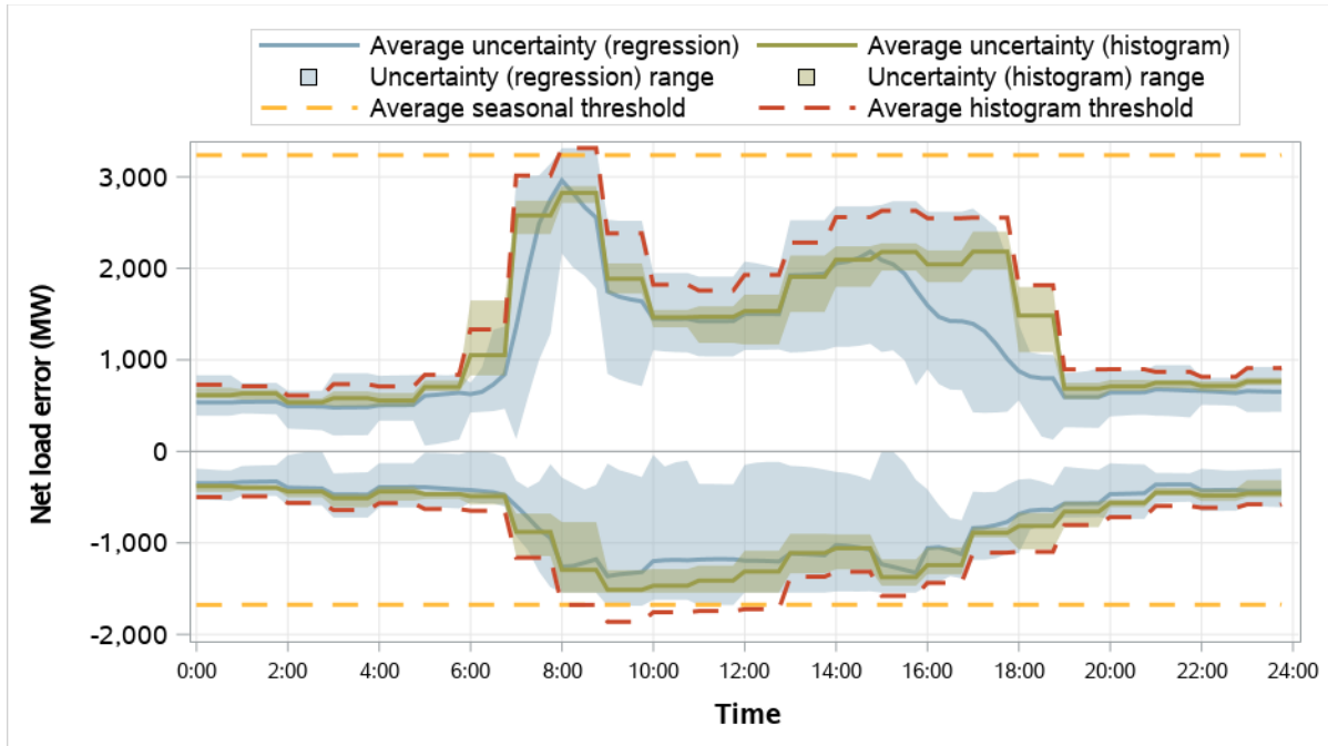
Figure 5.10 California ISO resource sufficiency evaluation uncertainty requirements (October–December 2025)
