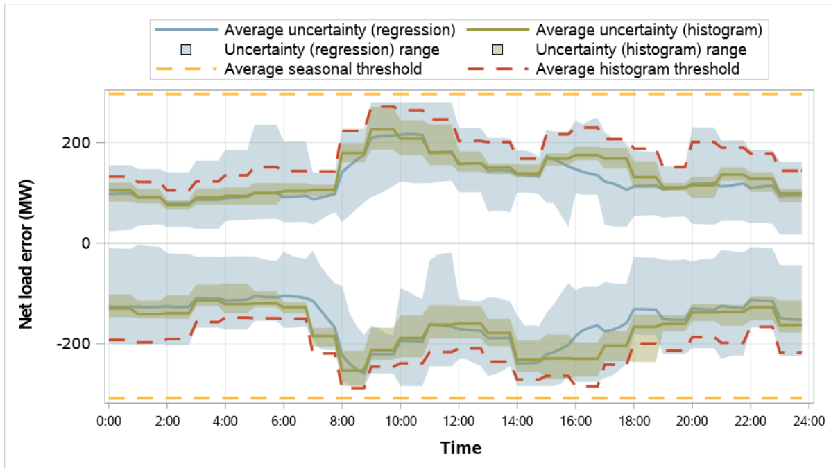
Figure 5.12 Idaho Power resource sufficiency evaluation uncertainty requirements (October–December 2025)
