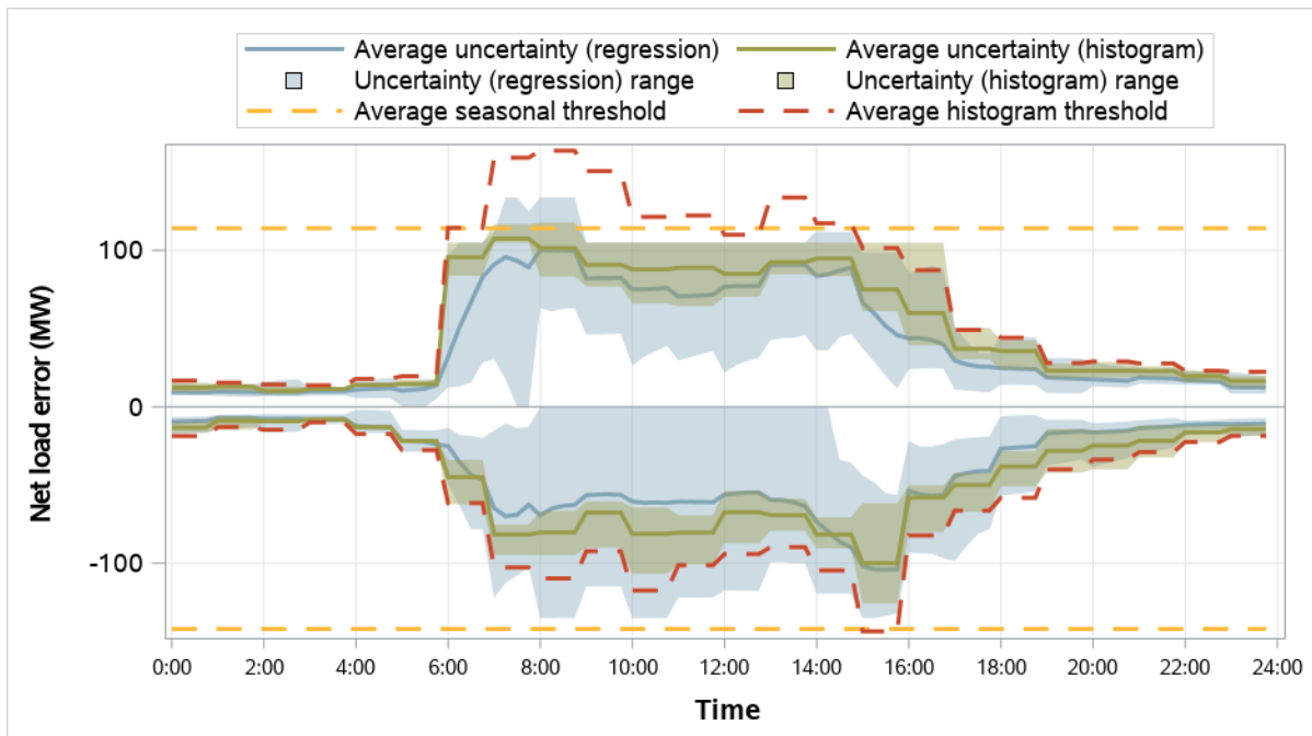
Figure 5.11 El Paso Electric resource sufficiency evaluation uncertainty requirements (October–December 2025)
