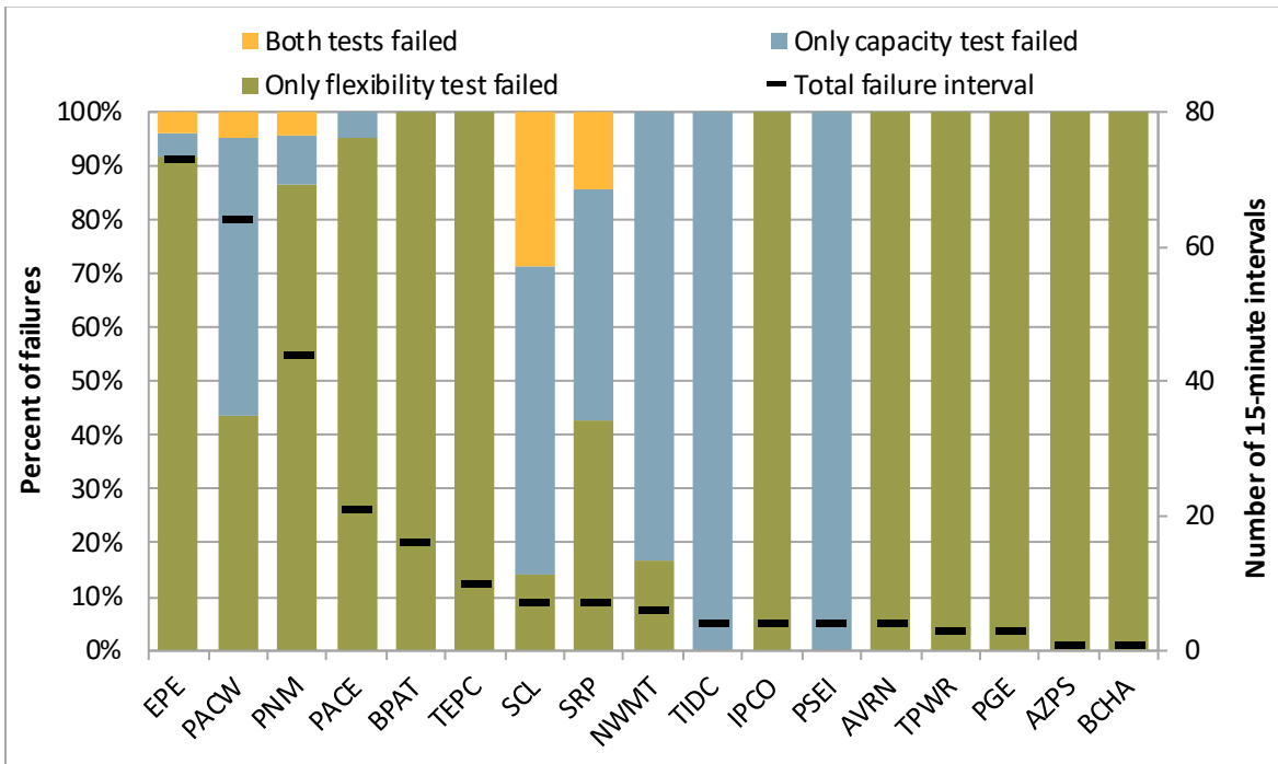
Figure 2.11 Upward capacity/flexibility test failure intervals by concurrence (October–December 2025)
