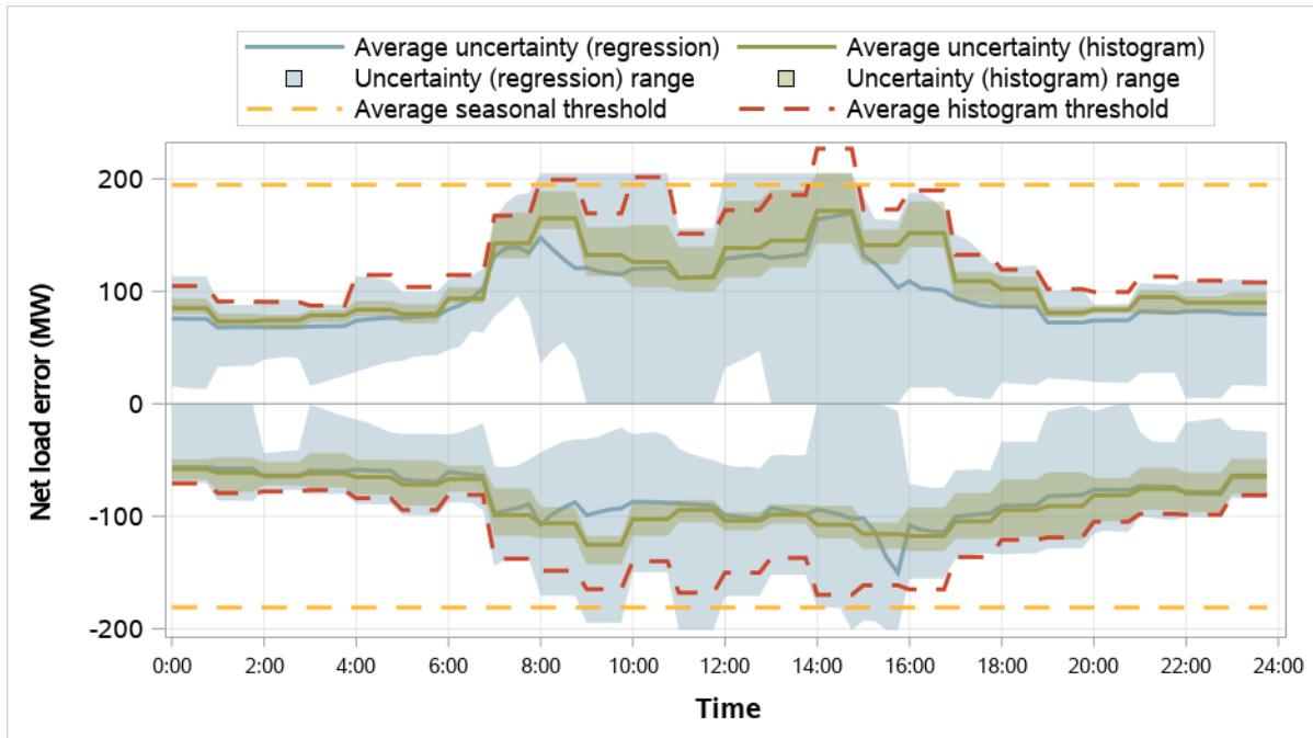
Figure 5.25 Tucson Electric Power resource sufficiency evaluation uncertainty requirements (October–December 2025)
