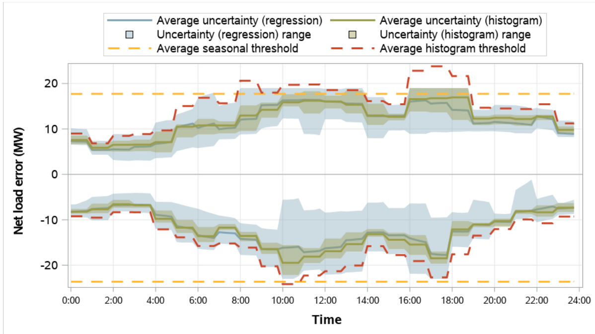
Figure 5.24 Tacoma Power resource sufficiency evaluation uncertainty requirements (October–December 2025)
