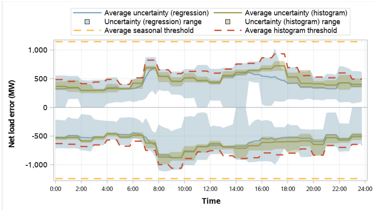
Figure 5.16 PacifiCorp East resource sufficiency evaluation uncertainty requirements (October–December 2025)
