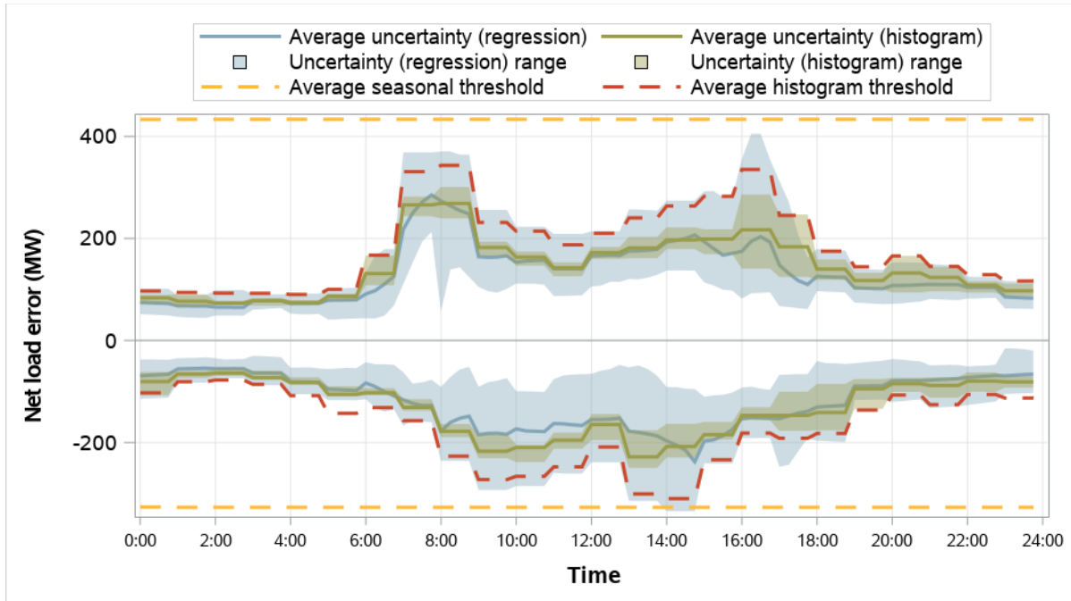
Figure 5.22 Salt River Project resource sufficiency evaluation uncertainty requirements (October–December 2025)
