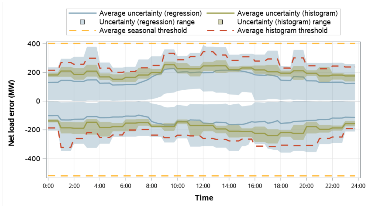
Figure 5.6 Avangrid resource sufficiency evaluation uncertainty requirements (October–December 2025)
