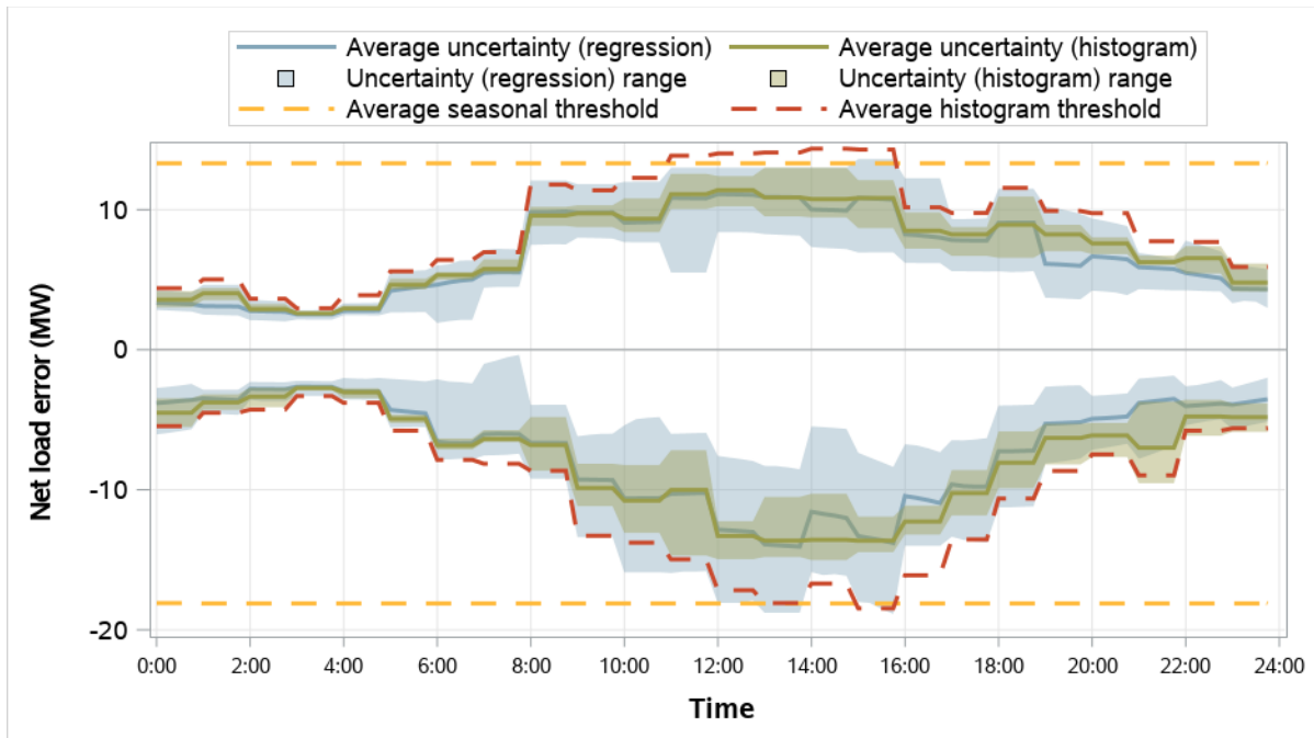
Figure 5.26 Turlock Irrigation District resource sufficiency evaluation uncertainty requirements (October–December 2025)
