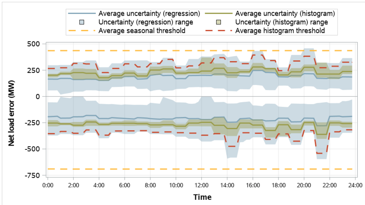
Figure 5.9 BPA resource sufficiency evaluation uncertainty requirements (October–December 2025)
