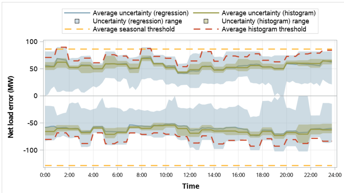
Figure 5.7 Avista resource sufficiency evaluation uncertainty requirements (October–December 2025)
