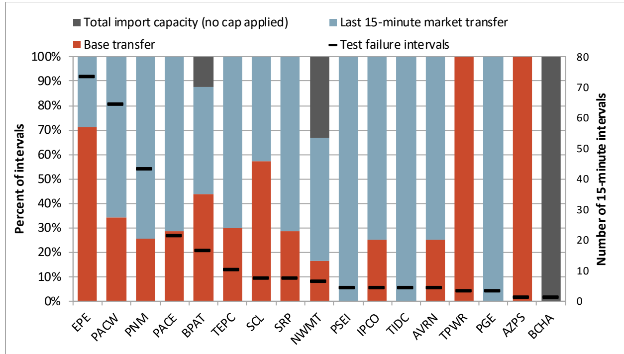
Figure 7.1 Upward capacity/flexibility test failure intervals by source of import limit (October–December 2025)
