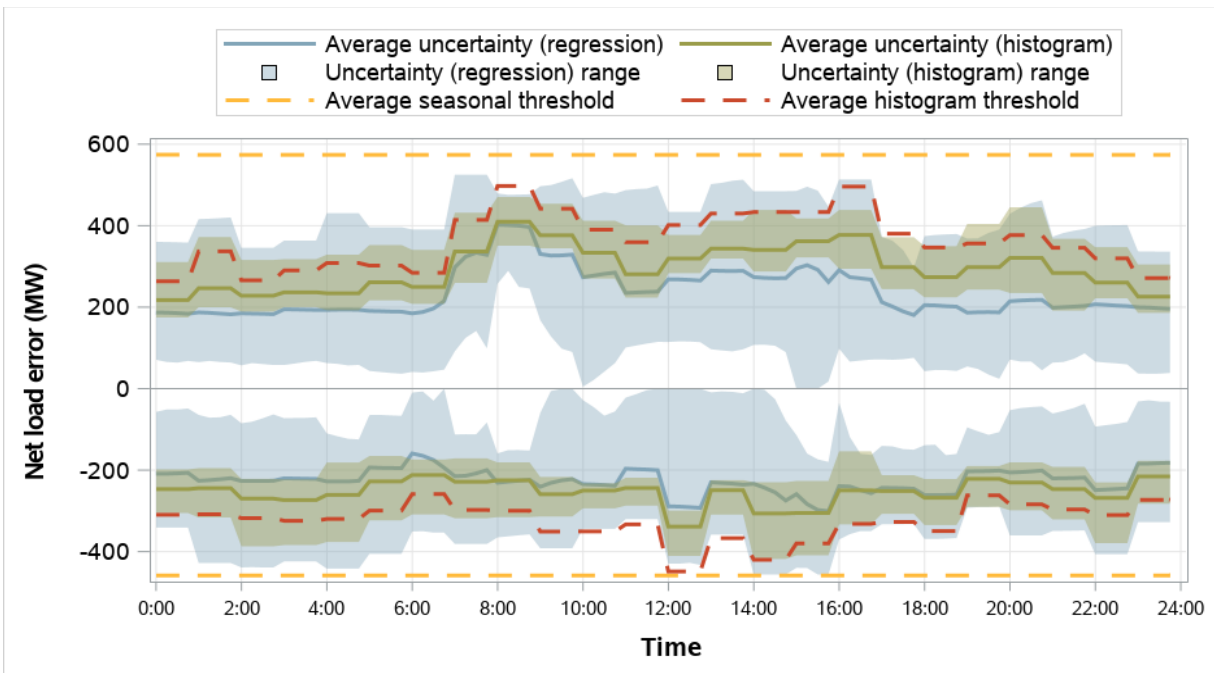
Figure 5.5 Arizona Public Service resource sufficiency evaluation uncertainty requirements (October–December 2025)
