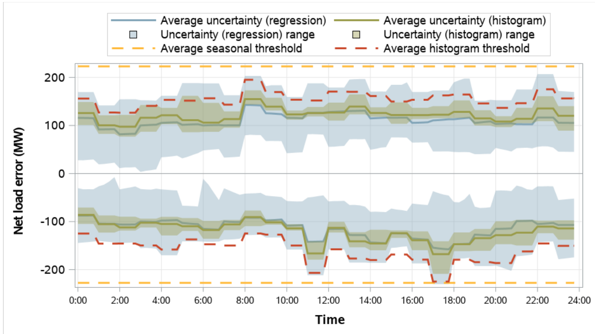
Figure 5.18 Portland General Electric resource sufficiency evaluation uncertainty requirements (October–December 2025)
