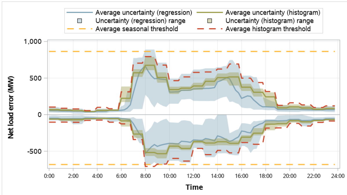
Figure 5.15 NV Energy resource sufficiency evaluation uncertainty requirements (October–December 2025)
