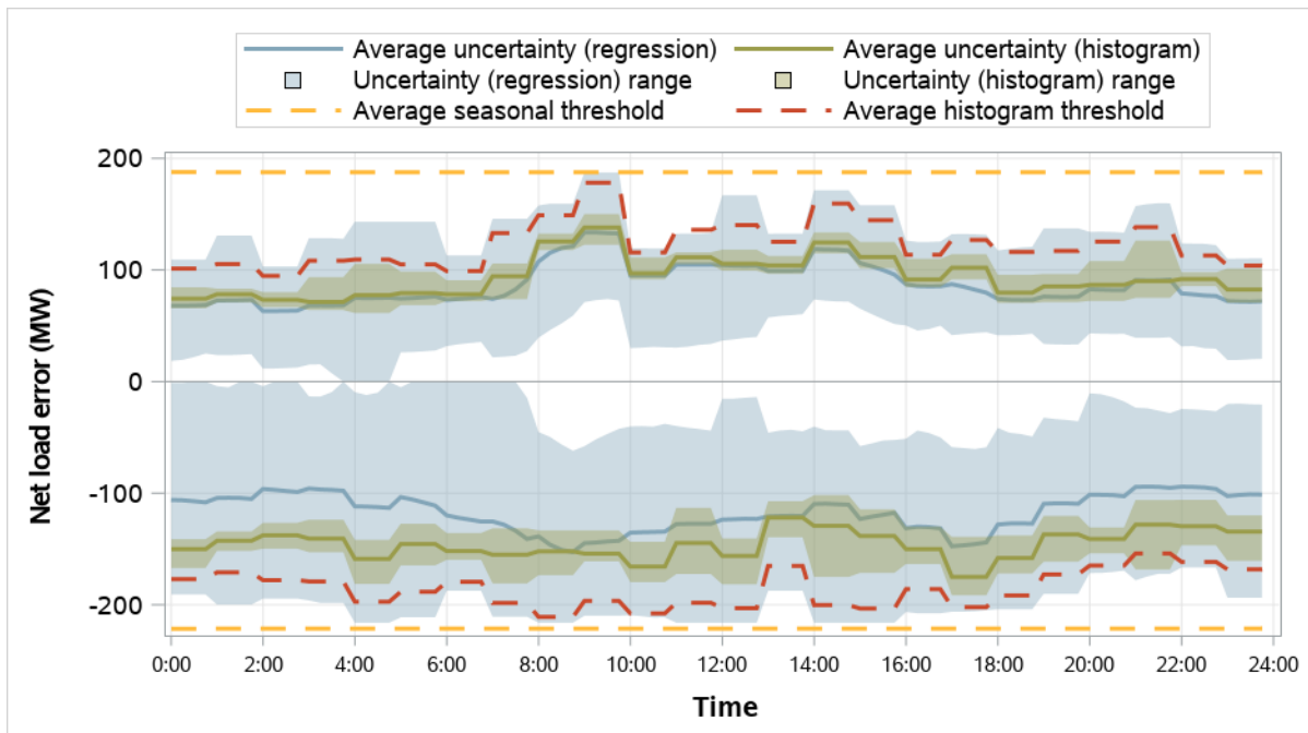
Figure 5.17 PacifiCorp West resource sufficiency evaluation uncertainty requirements (October–December 2025)
