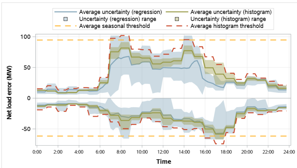
Figure 5.27 WAPA Desert Southwest resource sufficiency evaluation uncertainty requirements (October–December 2025)
