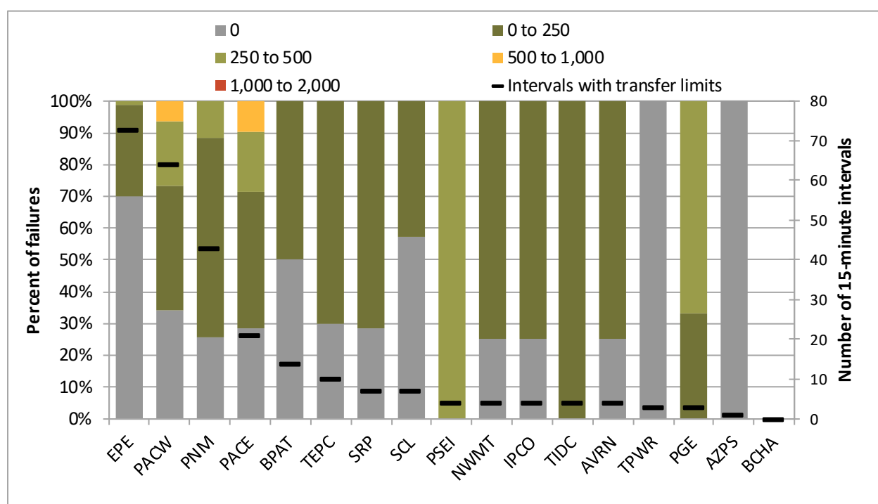
Figure 7.2 Upward capacity/flexibility test failure intervals by dynamic import limit (October–December 2025)
