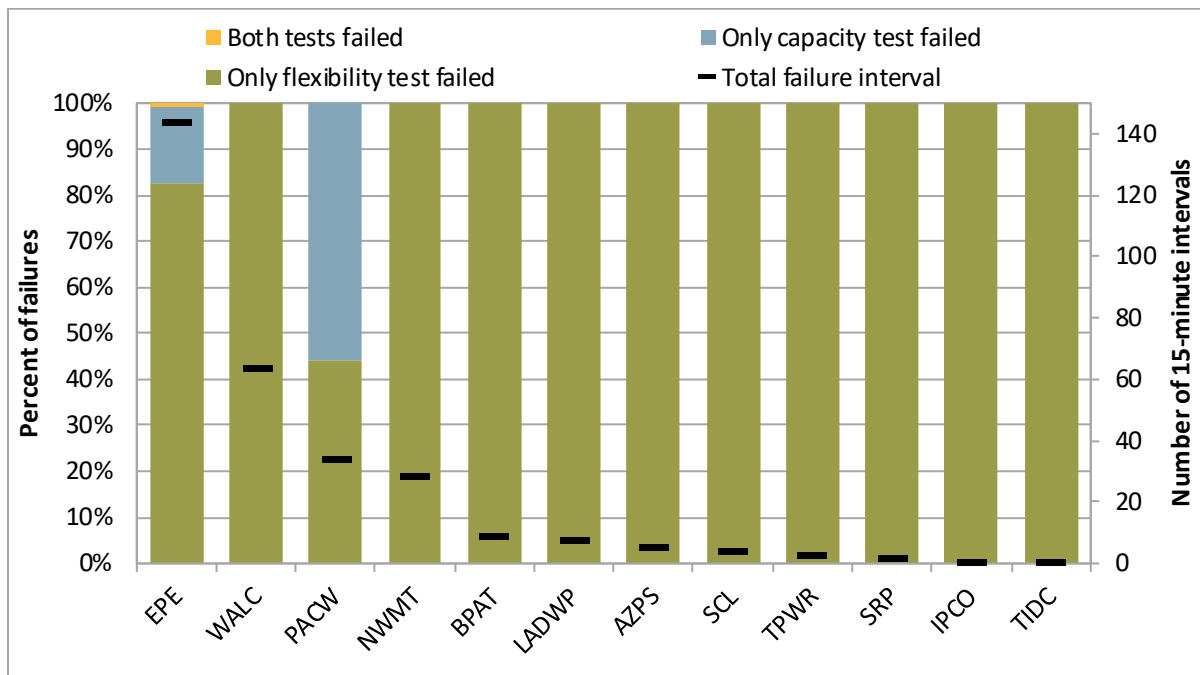
Figure 2.12 Downward capacity/flexibility test failure intervals by concurrence (October–December 2025)
