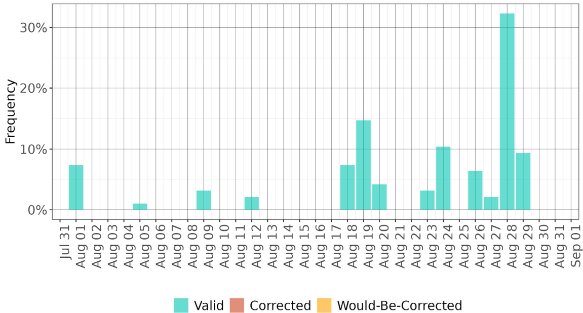
Figure 2: Frequency of FMM under-supply infeasibilities in the GWA BAA
