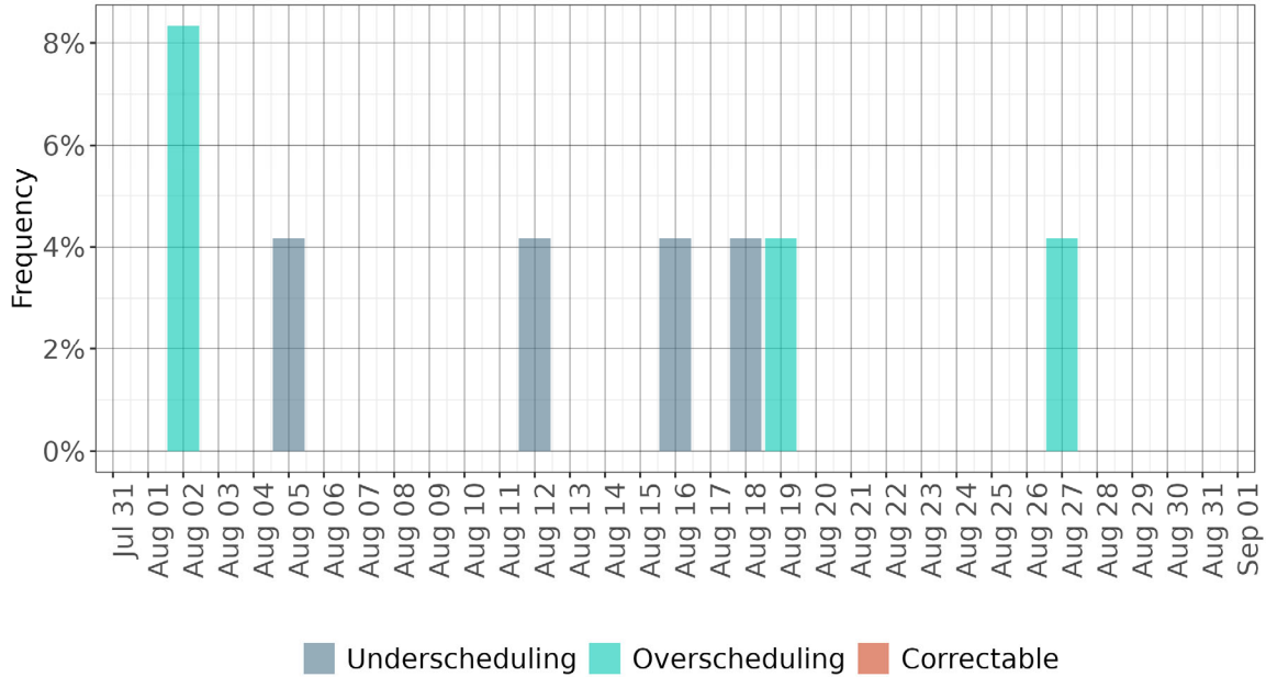
Figure 6: Frequency of Balancing test failures in the GWA BAA
