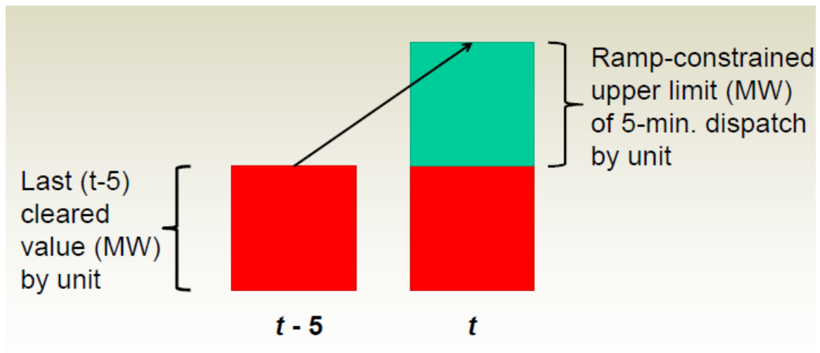
Figure 37: Measurement of 5-minute load following up capability
