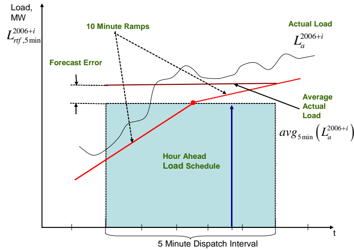
Figure 25: CAISO Simulated Real Time Load Forecast (Red Line)
