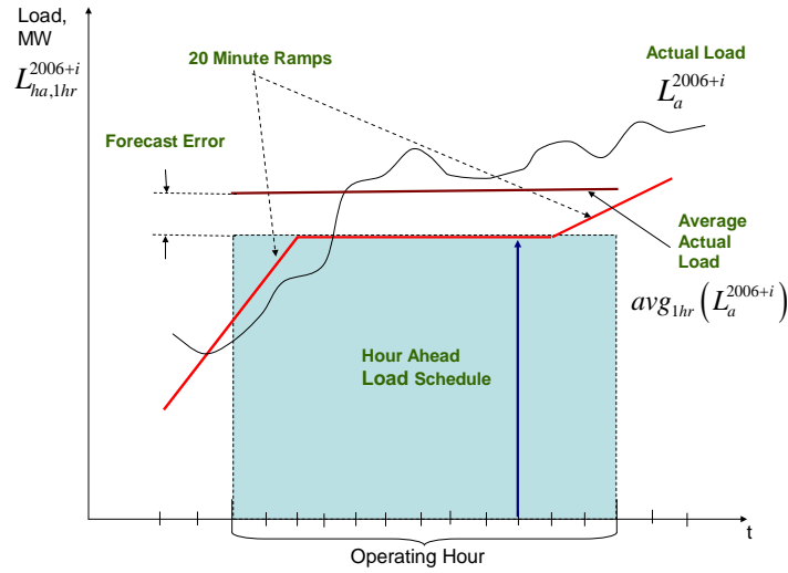
Figure 23: CAISO Simulated Hour Ahead Load Schedule (Red Line)
