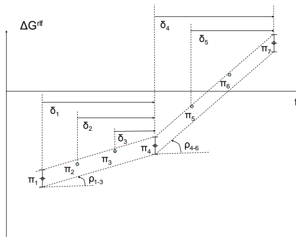
Figure 29: "Swinging Window" Algorithm – Obtaining Regulation, Ramps, and Their Duration
