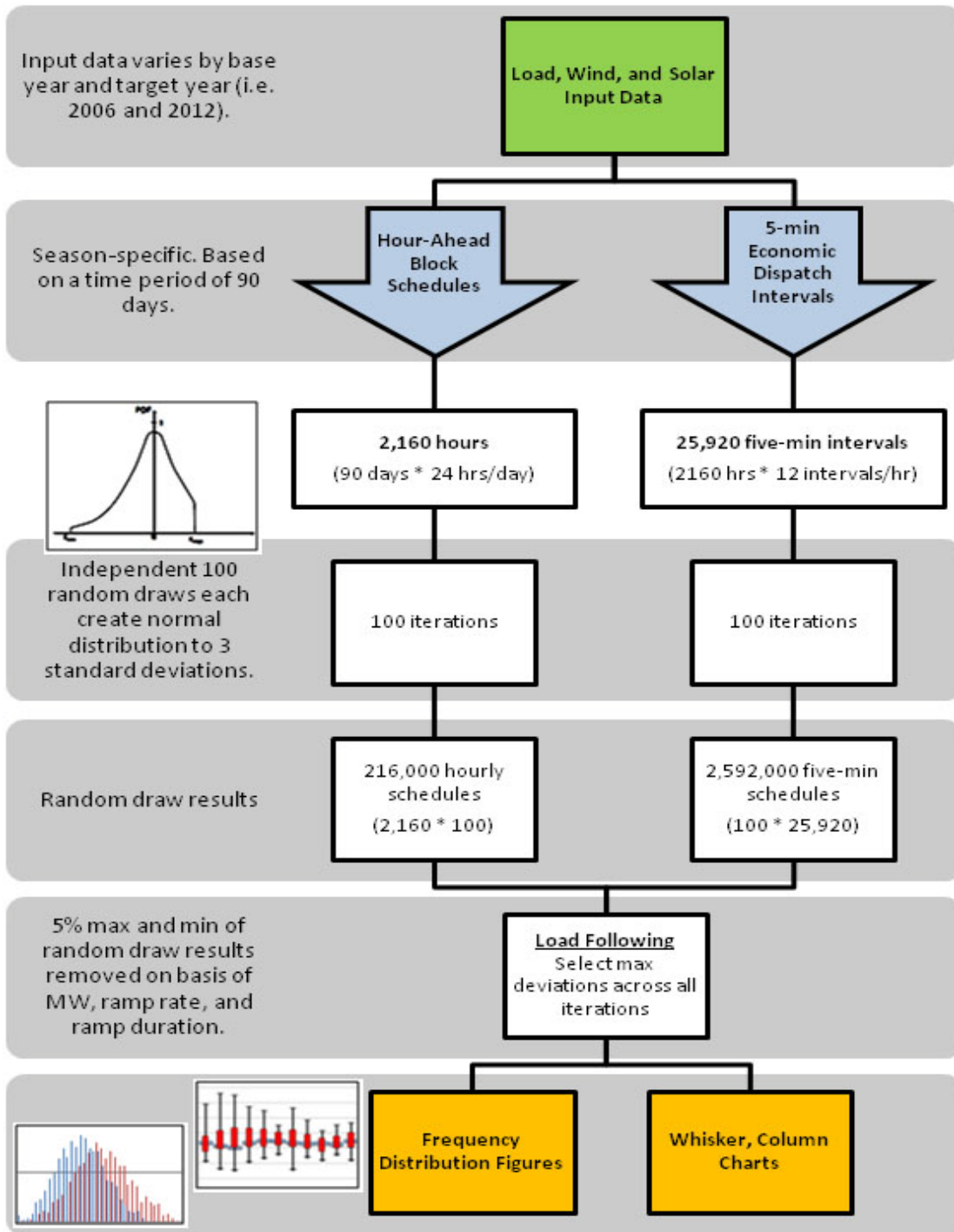
Figure 31: Analytical Flow Chart for Calculating Load-following Capacity Requirements
