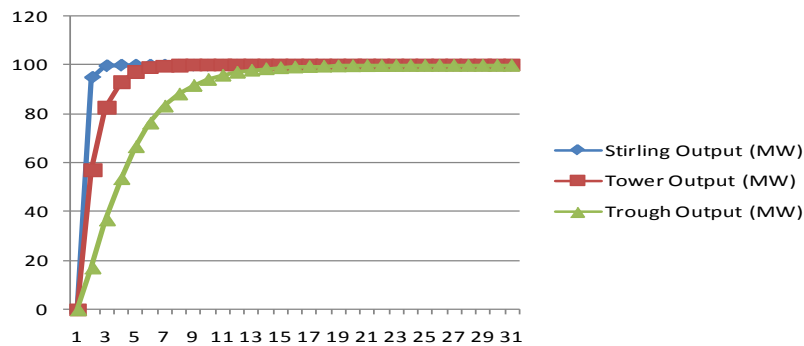
Figure 11: Response to Step Increase in Irradiance by Solar Thermal Technology vs. Time in Minutes
