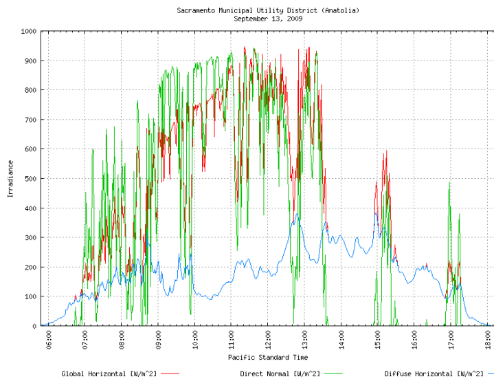
Figure 13: 1 Minute Irradiance for September 13, 2009
