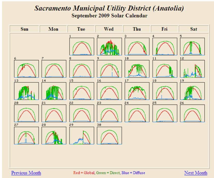
Figure 12: SMUD 1 Minute Irradiance Data for September 2009
