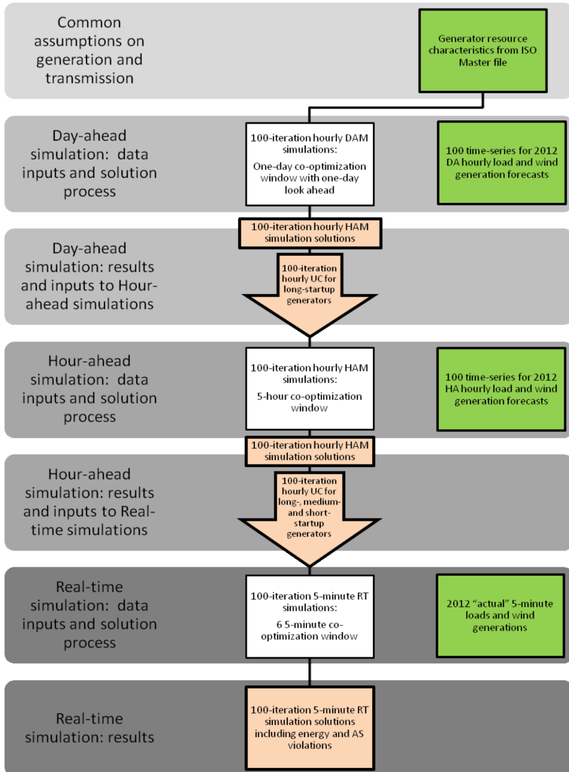
Figure 36: Flowchart of the Stochastic, Sequential Production Simulation Methodology
