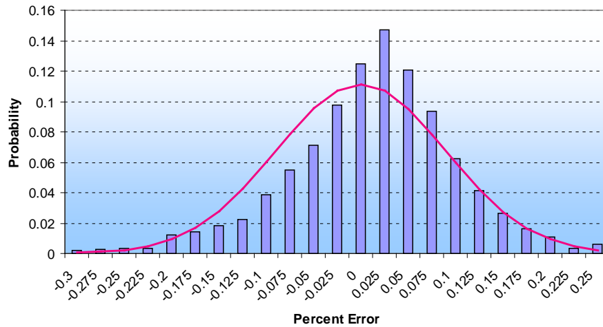
Figure 20: Two-hour-ahead wind forecasting error, Spring 2006
