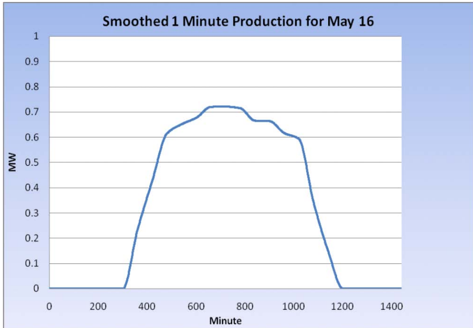
1 Minute Smoothed Production Data for a Tracking PV in the Mountain Pass/Tehachapi for May 16, 2020
