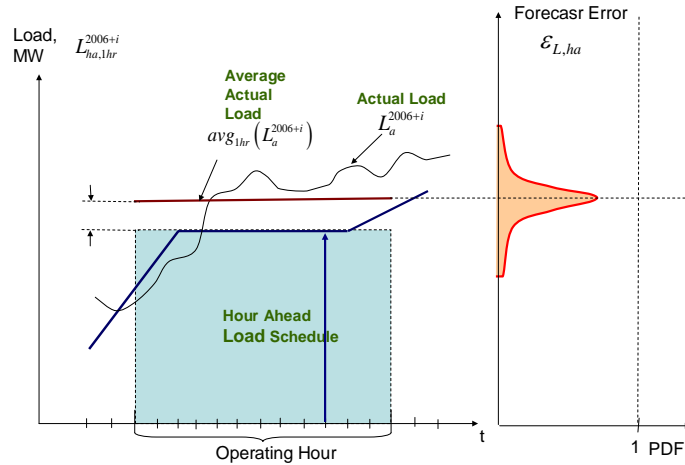
Figure 24: Probability Density Function (PDF) of the Load Forecast Function (Red Line)
