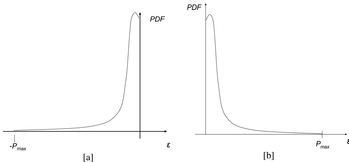
Figure 22: Distribution of solar forecast error on (a) a very cloudy day and (b) a very sunny day
