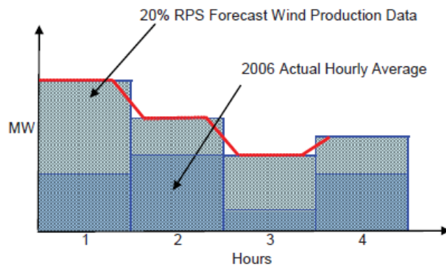
Figure 8: Possible Average Wind Generation Pattern
