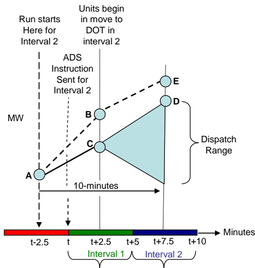
Figure 5: RTED Dispatch Ramping Projection
