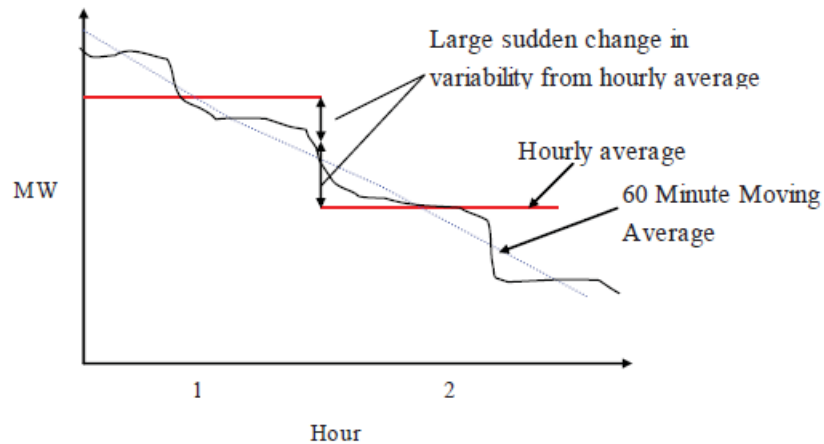
Figure 7: Sample Wind Production with Hourly Average and Moving Average
