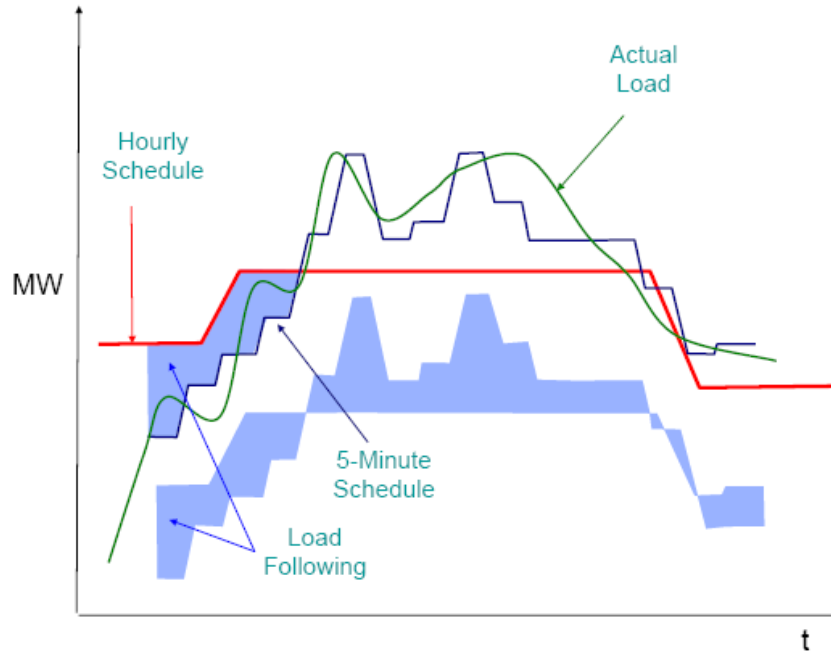
Figure 27: Depiction of hourly load-following requirement, shown as the blue area
