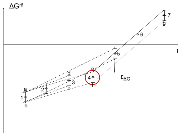
Figure 28: Concept for the "Swinging Door" Algorithm
