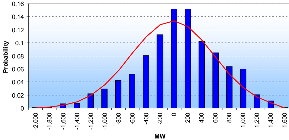
Figure 18: Hour-Ahead Load Forecasting Error, Spring 2006
