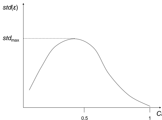
Figure 21: Distribution of the standard deviation of solar forecast error depending on the clearness index
