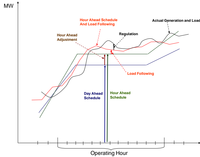
Figure 1: ISO Balancing Area Scheduling Process
