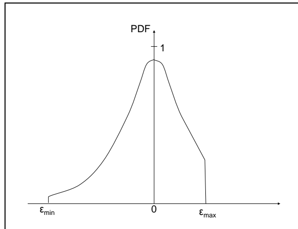
Figure 17: Unbiased Truncated Normal Distribution
