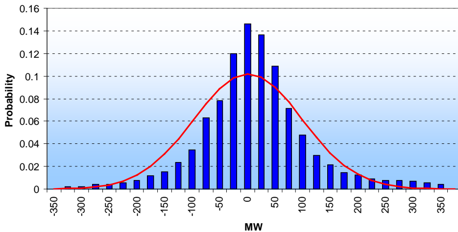
Figure 19: Comparison of five-minute load forecast error and theoretical error distribution, mid-May to mid-April, 2006
