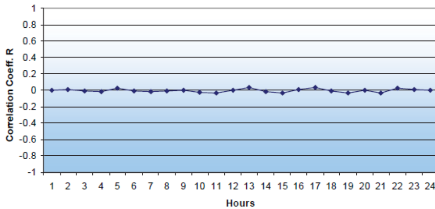
Figure 10: Correlation of Short-Term Variations of Two Wind Parks in Tehachapi Resource Area, May 2006
