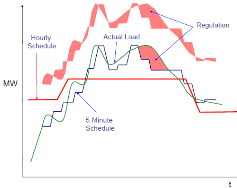
Figure 26: Depiction of the Regulation requirement, shown as the red shaded area
